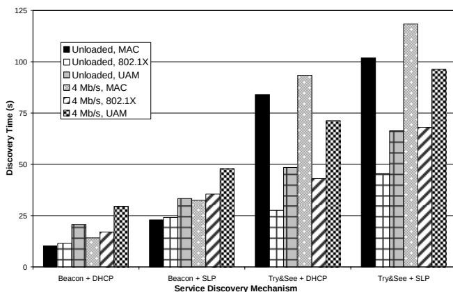
Fig. 8 – Colour printing: service discovery times.
