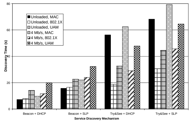
Fig. 9 – B/W printing: service discovery times.
