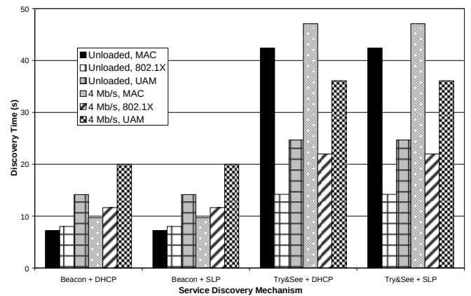
Fig. 10 – Web browsing: service discovery times.
