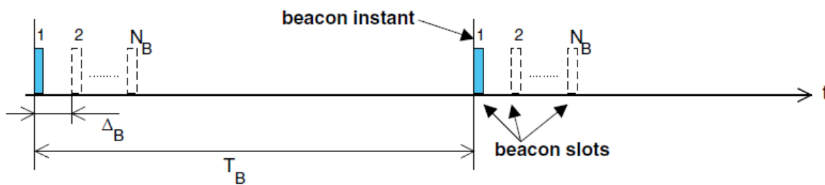
Figure 72—General beacon train format
