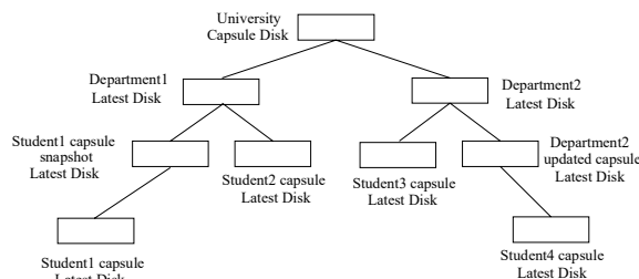
Figure 1: An example capsule hierarchy.
