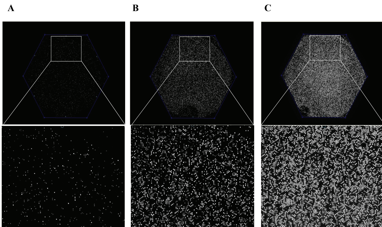
Supporting Figure S-1. Fluorescence images generated using SiMoA of singulated beads at approximately (A) AEB \sim 0.1 , where the majority of beads were associated with 0 or 1 enzyme molecules, (B) AEB \sim 0.6 , where a significant number of beads were associated with multiple enzyme molecules, and (C) AEB \sim 3.0 , where all beads were associated with at least 1 enzyme molecule. The images shown are of the analog, fluorescence signal generated by the experiment, i.e., (I_{\text{bead},F2} - I_{\text{bead},F1}) (see main text).
