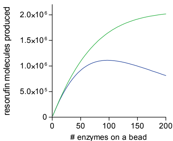
Supporting Figure S-4. Plot of the number of resorufin molecules produced during a 150 s experiment as a function of the number of enzymes on a bead. The theoretical limit of our system (green curve) is modeled where image acquisition begins at t=0 , immediately when the seal is made, and before any RGP is converted into resorufin. The current sealing and imaging condition (blue curve) is modeled with a 45 s time lapse between seal and image.
