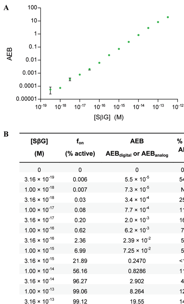
Figure 3. Broad dynamic range to enzyme label was achieved by combining digital and analog measurements in SiMoA. (A) Plot of AEB as a function of enzyme concentration. The error bars are standard deviations over three replicates. (B) % active and AEB values as a function of enzyme concentration. AEB was determined using eq 2 for % active <70%. AEB was determined using eq 3 for % active >70%. The threshold between analog and digital in this experiment was between 10 fM and 31.6 fM.
