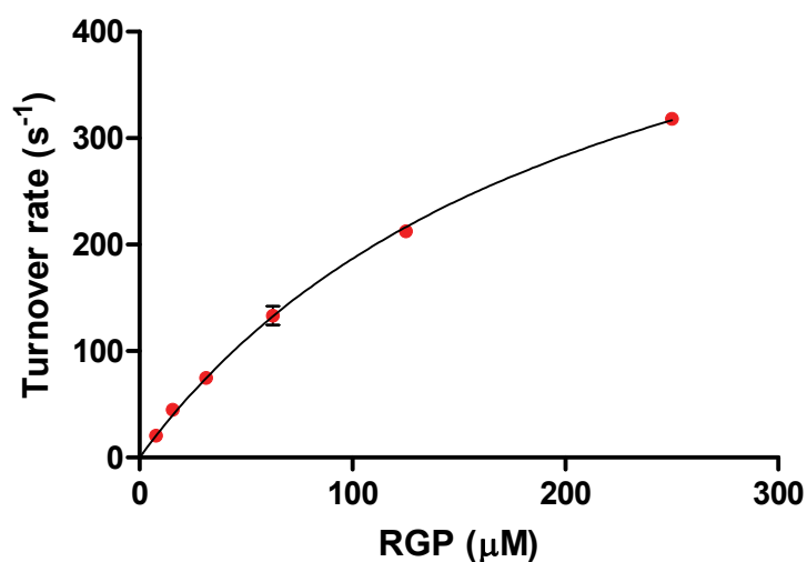
Supporting Figure S-3. Michaelis-Menten curve of RGP turnover by streptavidin- \beta -galactosidase. K_M and V_{max} were calculated using curve fitting software (GraphPad) to be 217 \mu\text{M} and 591 \text{s}^{-1} , respectively.
