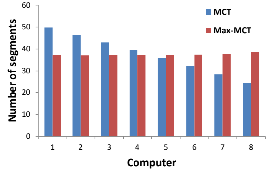
Fig. 5. The number of segments in different computers
