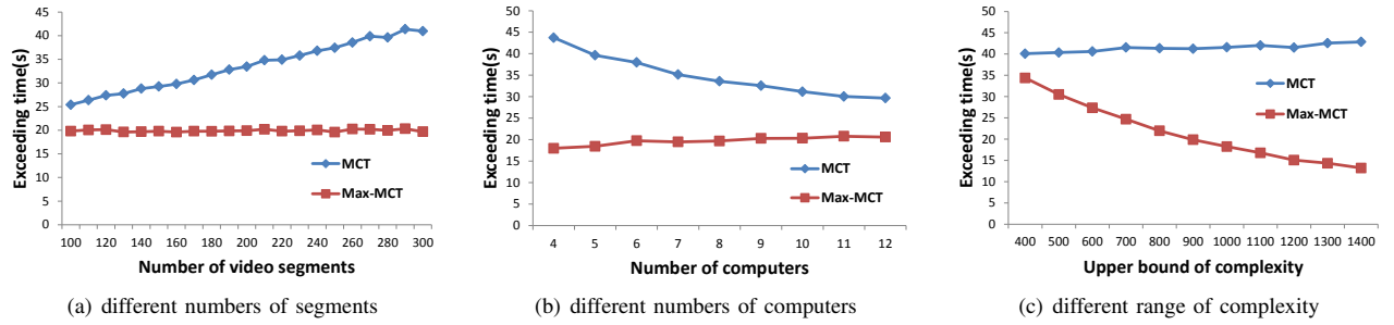
Fig. 4. Exceeding time with different environments
