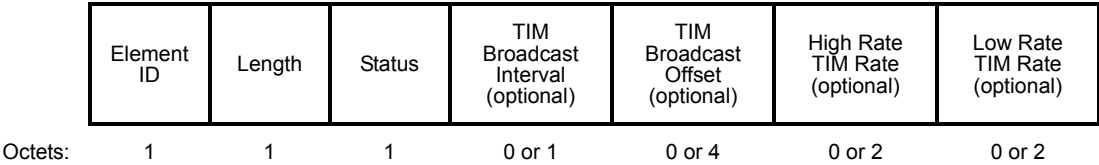
Figure 8-340—TIM Broadcast Response element format
