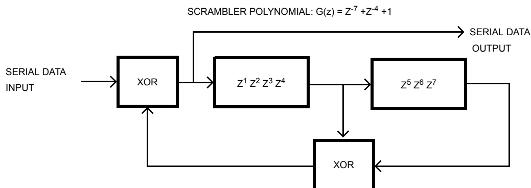
Figure 17-5—Data scrambler
