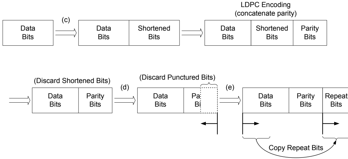
Figure 20-13—LDPC PPDU encoding padding and puncturing of a single codeword
