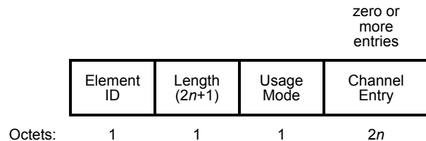
Figure 8-343—Channel Usage element format
