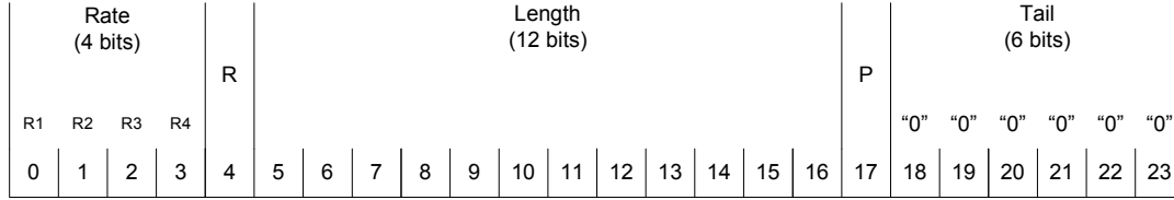
Figure 20-5—L-SIG structure
