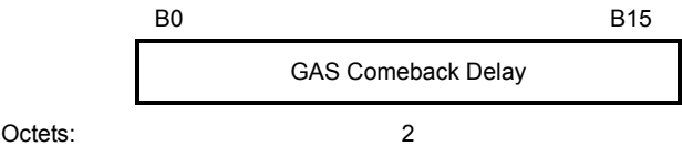
Figure 8-457—GAS Comeback Delay field
