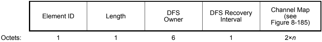
Figure 8-184—IBSS DFS element format
