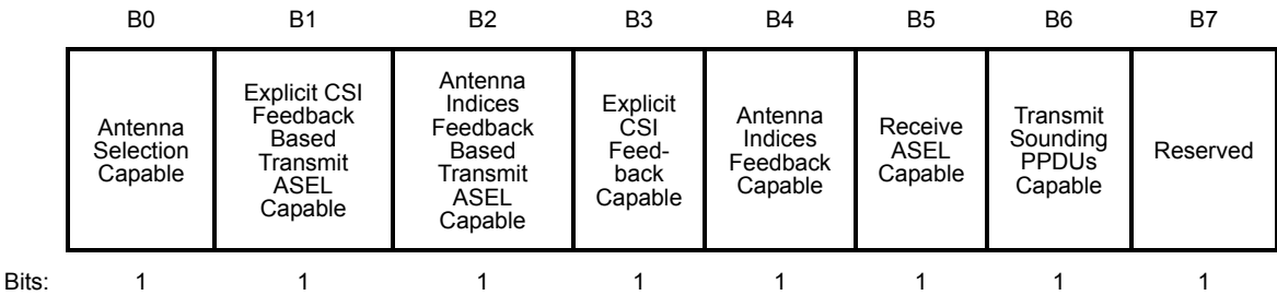
Figure 8-254—ASEL Capability field
