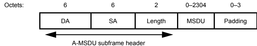
Figure 8-32—A-MSDU subframe structure
