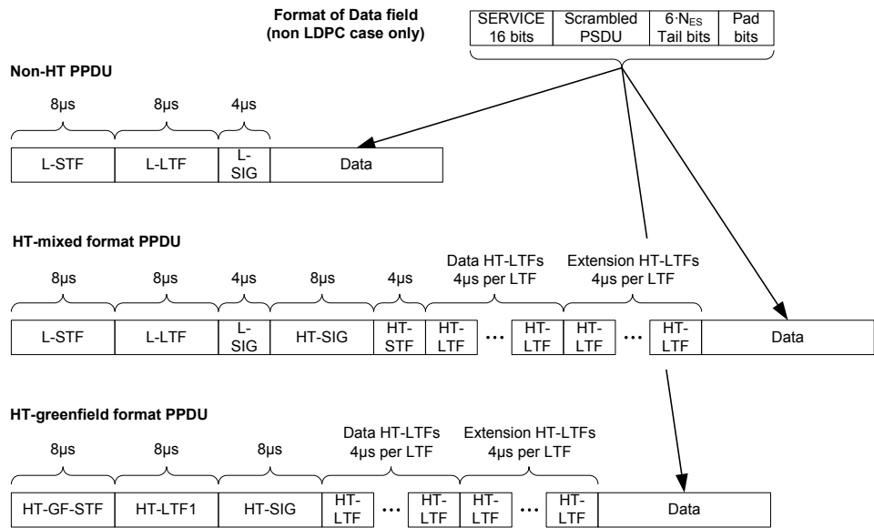
Figure 20-1—PPDU format
