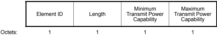
Figure 8-98—Power Capability element format
