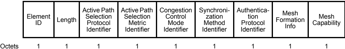
Figure 8-363—Mesh Configuration element format
