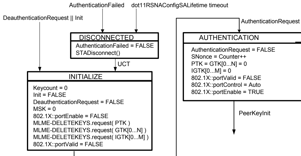
Figure 11-43—RSNA Supplicant key management state machine
