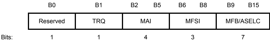
Figure 8-6—Link Adaptation Control subfield
