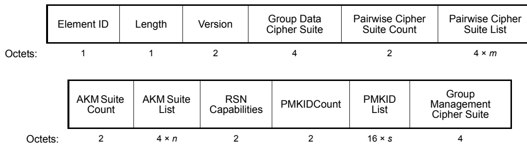
Figure 8-186—RSNE format
