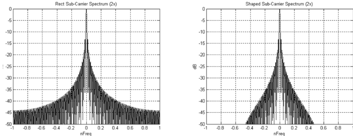
Figure 19-10—Subcarrier spectra for rectangular windowing and Clause 18 suggested windowing
