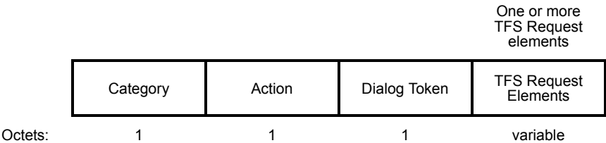
Figure 8-484—TFS Request frame format
