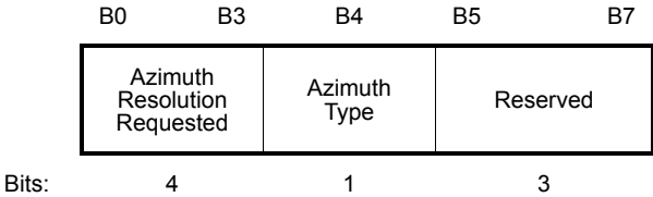
Figure 8-125—Azimuth Request field
