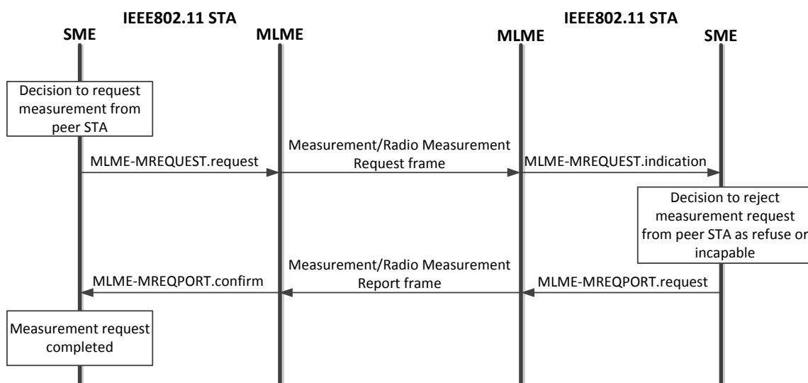
Figure 6-4—Measurement request—rejected
