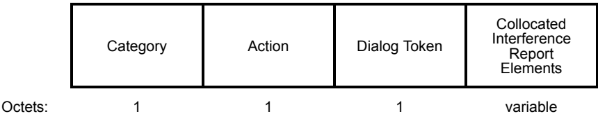
Figure 8-483—Collocated Interference Report frame format
