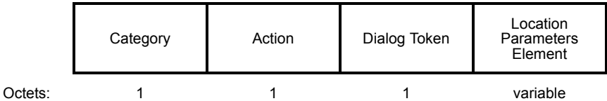
Figure 8-472—Location Configuration Response frame body format
