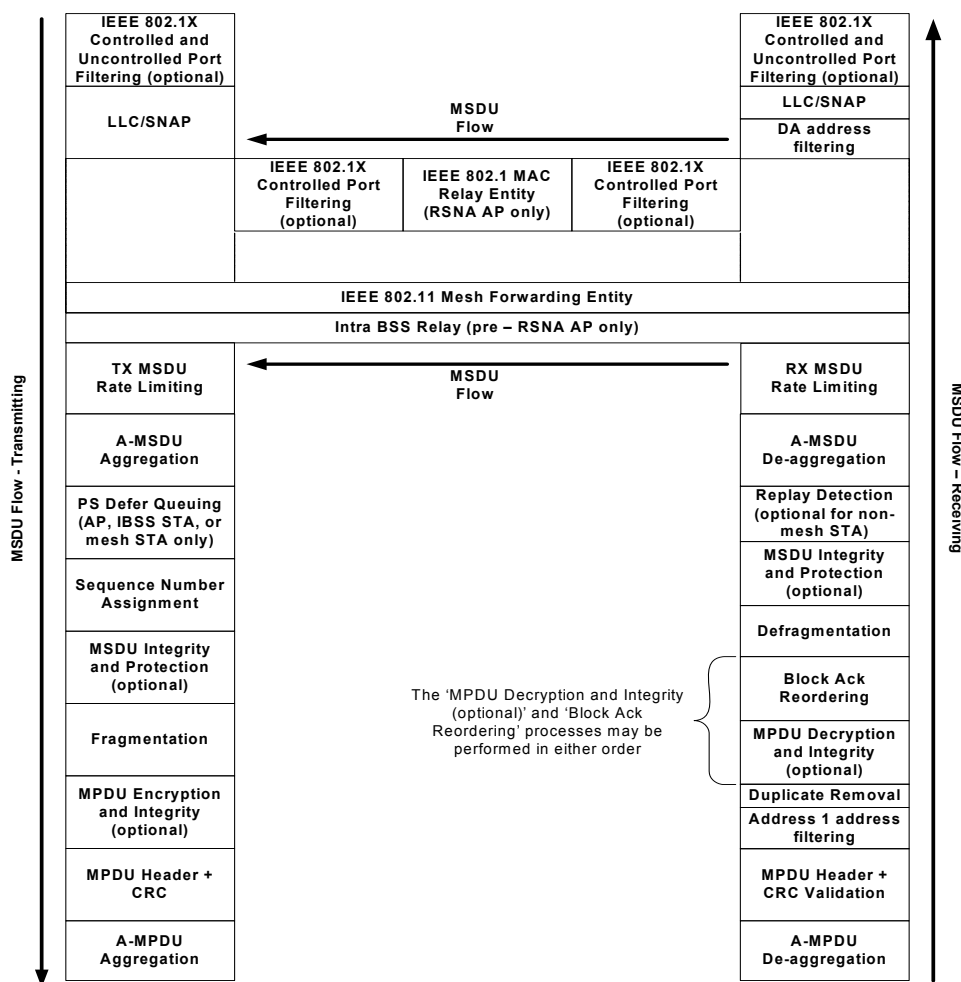
Figure 5-1—MAC data plane architecture
