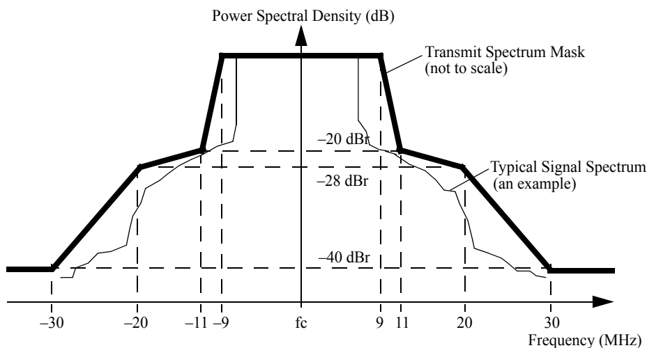
Figure 18-13—Transmit spectrum mask for 20 MHz transmission
