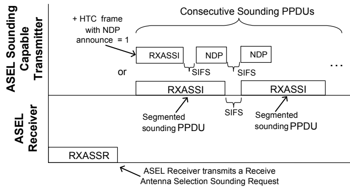
Figure 9-41—Receive ASEL
