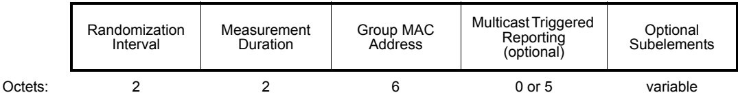
Figure 8-135—Measurement Request field format for a Multicast Diagnostics Request
