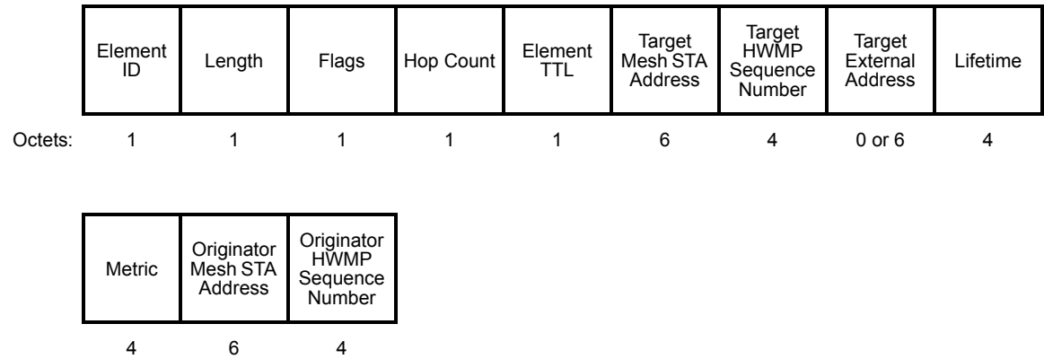
Figure 8-392—PREP element format
