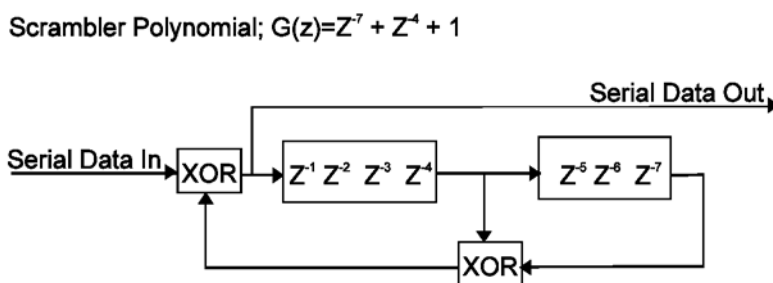
Figure 16-4—Data scrambler
