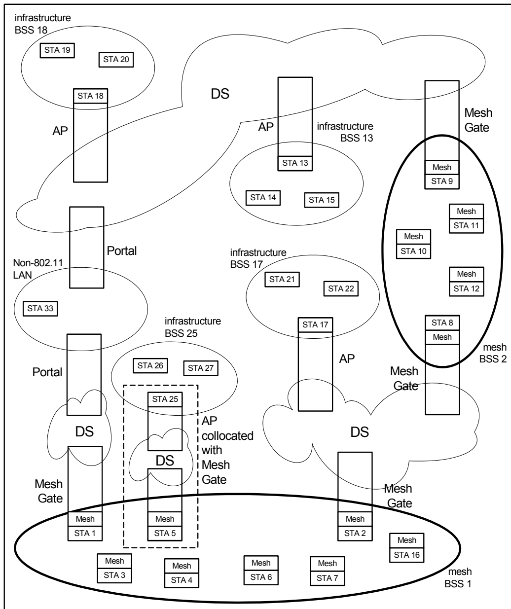
Figure 4-8—Example MBSS containing mesh STAs, mesh gates, APs, and portals
