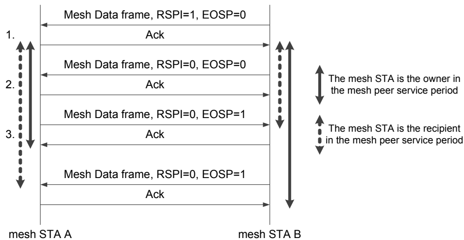
Figure 13-7—Mesh peer service period
