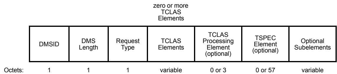
Figure 8-346—DMS Descriptor
