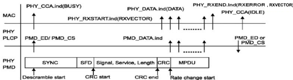
Figure 16-8—Receive PLCP
