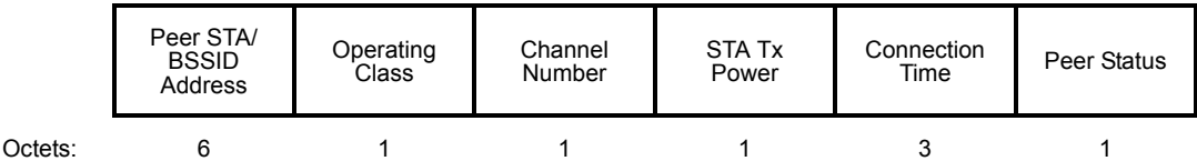
Figure 8-284—Event Report format for Peer-to-Peer Link event
