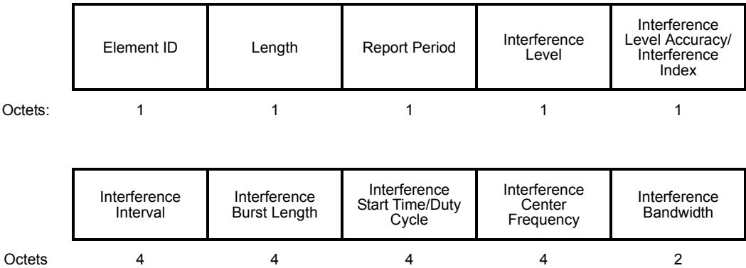
Figure 8-341— Collocated Interference Report element format
