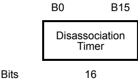
Figure 8-476—Disassociation Timer field format
