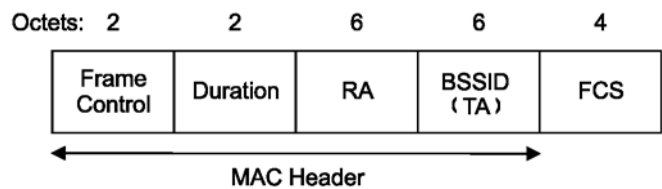
Figure 8-17—CF-End frame
