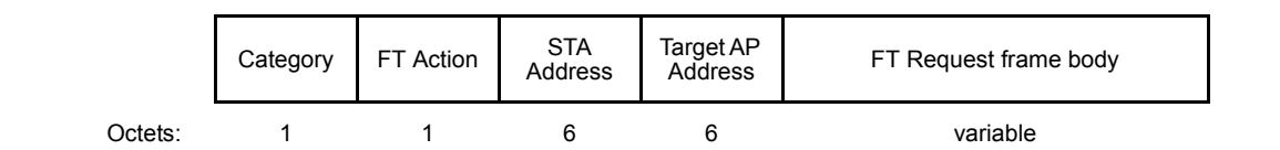
Figure 8-461—FT Request frame Action field format
