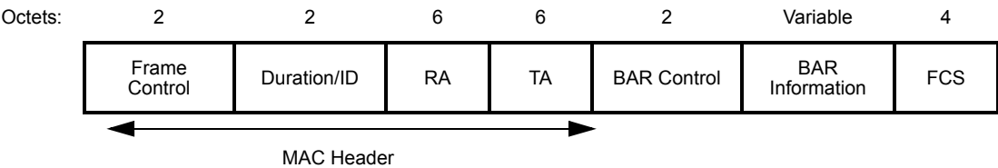
Figure 8-19—BlockAckReq frame
