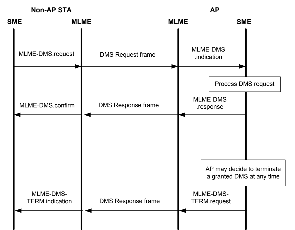
Figure 6-25—DMS setup protocol exchange
