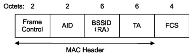
Figure 8-16—PS-Poll frame
