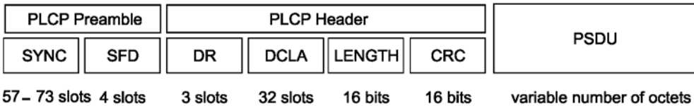
Figure 15-1—PPDU frame format
