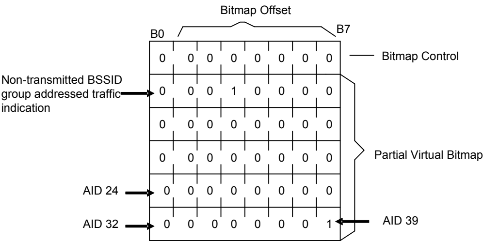
Figure O-6—Virtual Bitmap Example #5, Method A
