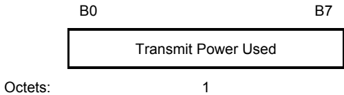
Figure 8-55—Transmit Power Used field
