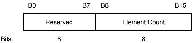
Figure 8-235—MIC Control field
