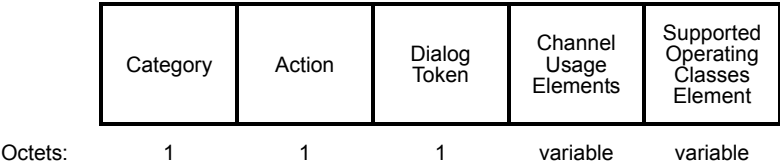
Figure 8-494—Channel Usage Request frame format
