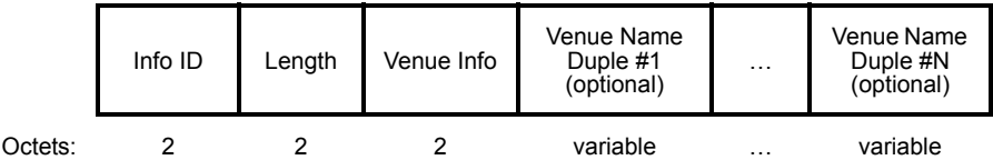
Figure 8-406—Venue Name ANQP-element format
