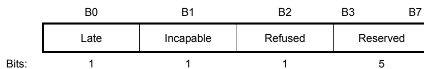
Figure 8-141—Measurement Report Mode field
