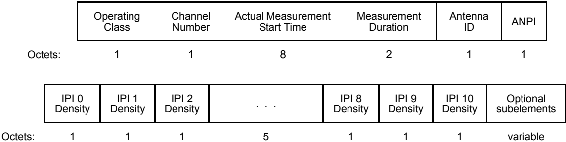
Figure 8-147—Measurement Report field format for Noise Histogram Report
