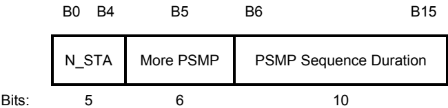
Figure 8-59—PSMP Parameter Set fixed field
