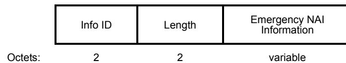
Figure 8-429—Emergency NAI ANQP-element format
