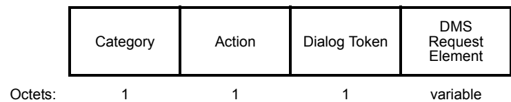
Figure 8-496—DMS Request frame format
