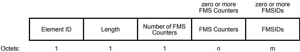
Figure 8-324—FMS Descriptor element format
