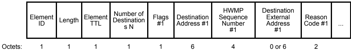
Figure 8-394—PERR element format
