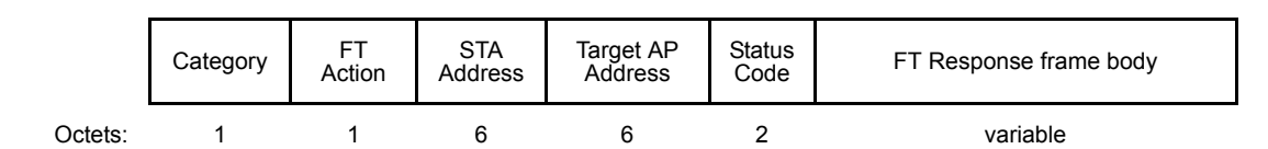
Figure 8-462—FT Response frame Action field format
