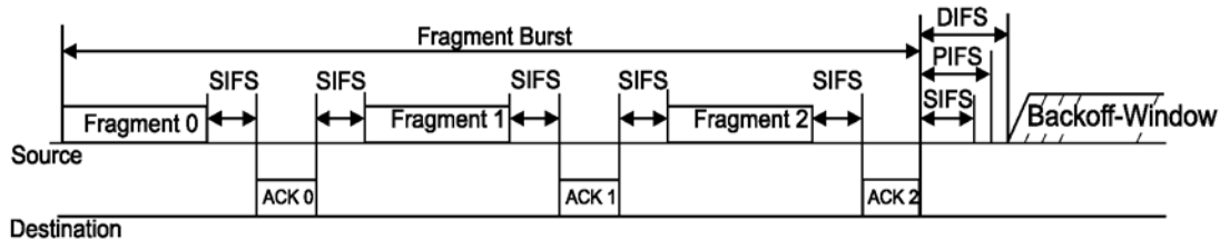
Figure 9-13—Transmission of a multiple-fragment MSDU using SIFS
