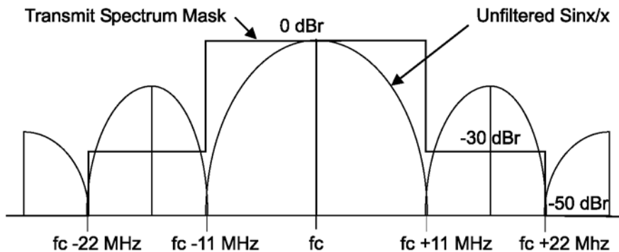
Figure 16-11—Transmit spectrum mask
