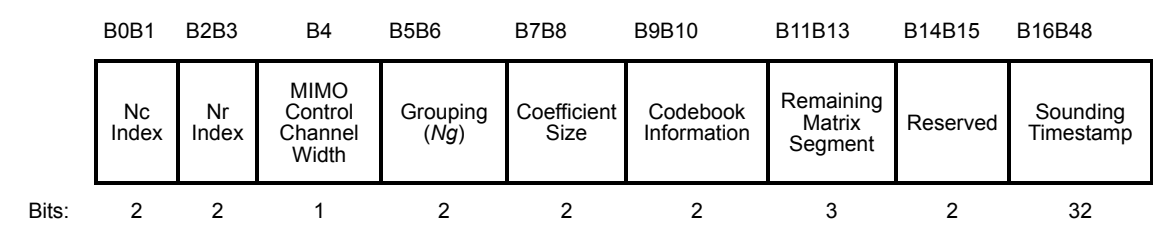
Figure 8-62—MIMO Control field
