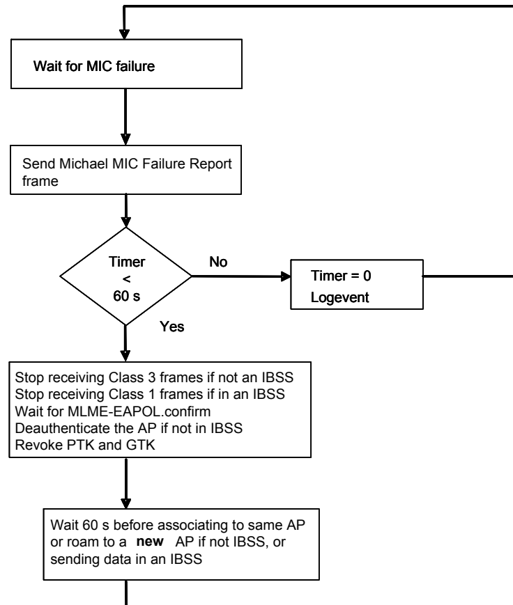
Figure 11-13—Supplicant MIC countermeasures
