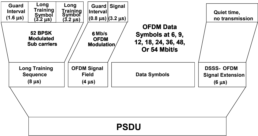
Figure 19-6—DSSS-OFDM PSDU
