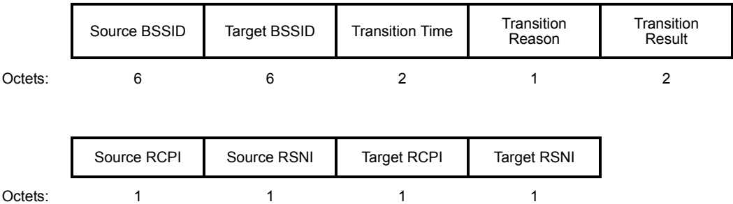
Figure 8-282—Event Report format for Transition event
