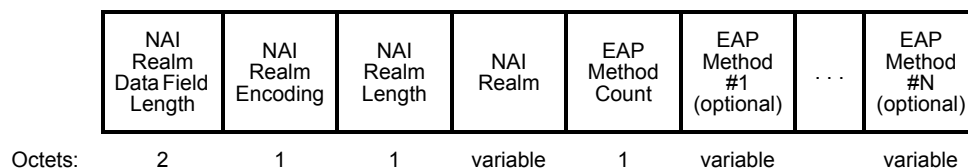
Figure 8-418—NAI Realm Data field format
