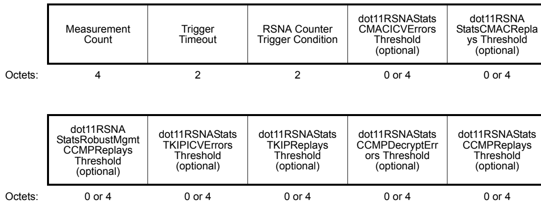
Figure 8-121—Triggered Reporting subelement for RSNA Counters
