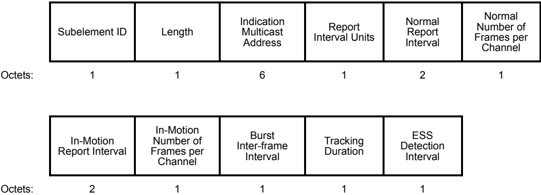
Figure 8-311—Location Indication Parameters subelement
