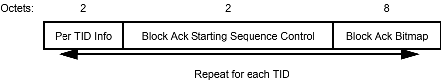
Figure 8-28—BA Information field (Multi-TID BlockAck)
