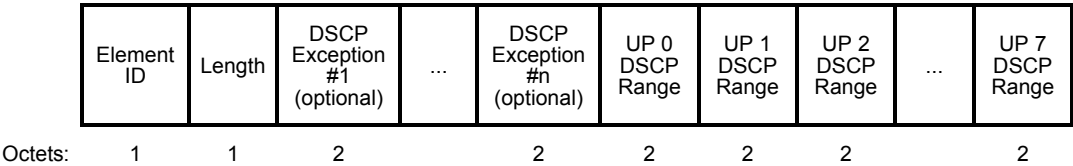
Figure 8-357—QoS Map Set element description
