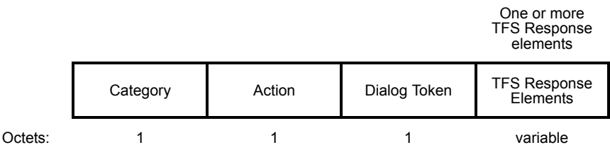
Figure 8-485—TFS Response frame format
