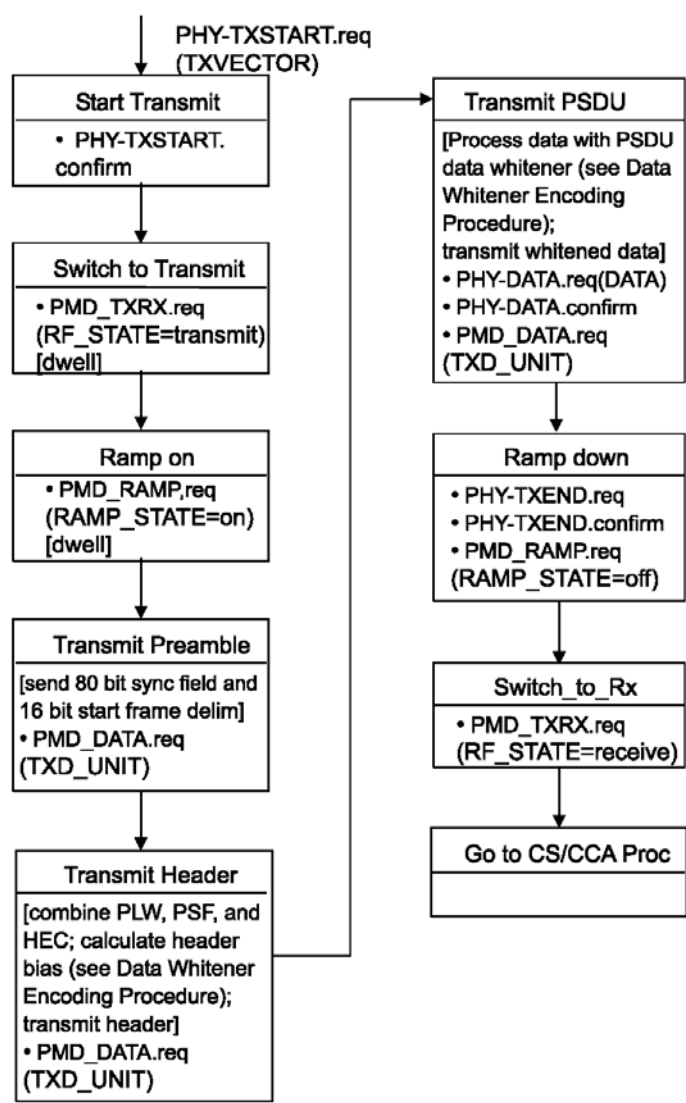
Figure 14-6—Transmit state machine
