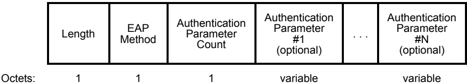
Figure 8-420—EAP Method subfield format
