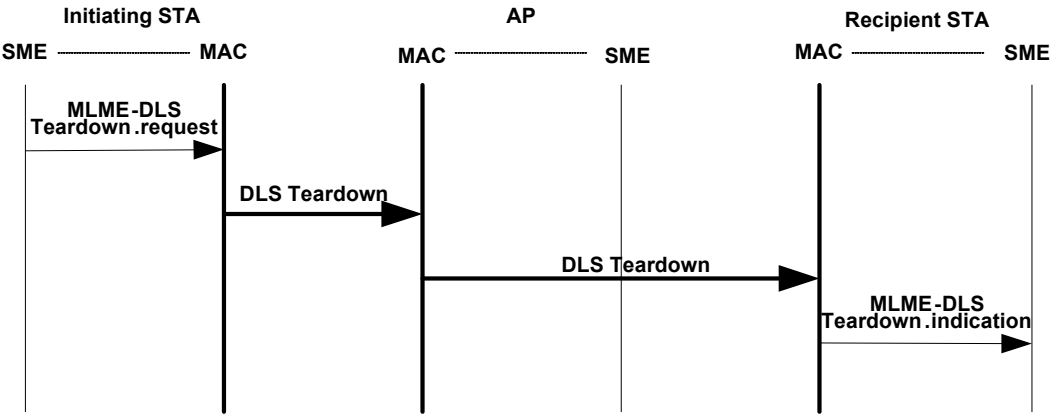
Figure 10-17—STA-initiated DLS teardown message flow
