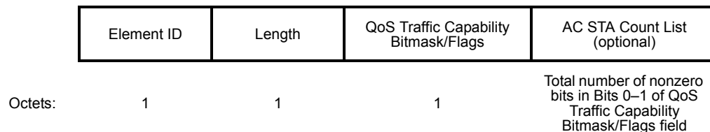
Figure 8-331—QoS Traffic Capability Element format
