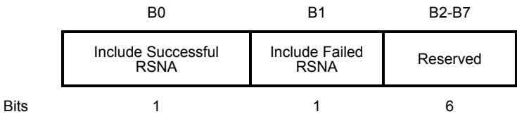
Figure 8-278—Match Value field definitions
