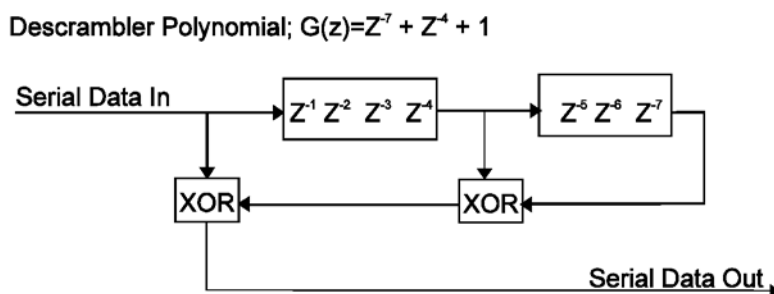
Figure 16-5—Data descrambler
