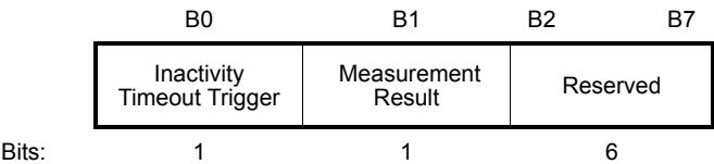
Figure 8-168—Multicast Reporting Reason field
