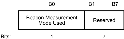
Figure 8-320—Options Used field format
