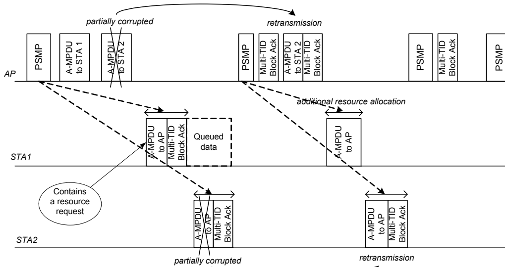
Figure 9-34—PSMP burst showing retransmission and resource allocation
