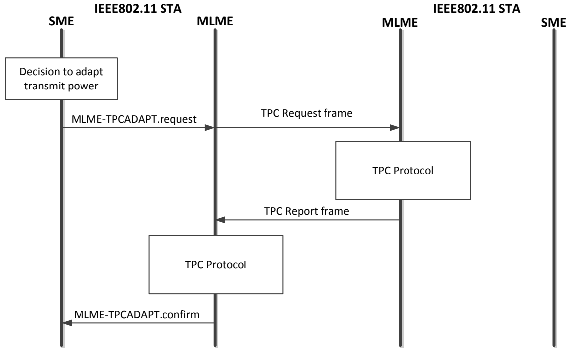
Figure 6-5—TPC adaptation
