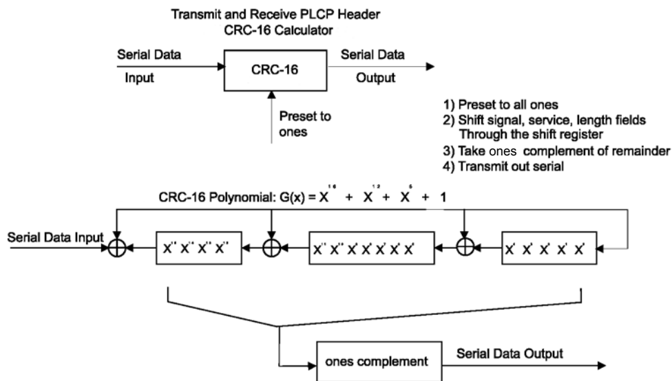
Figure 16-2—CRC-16 implementation
