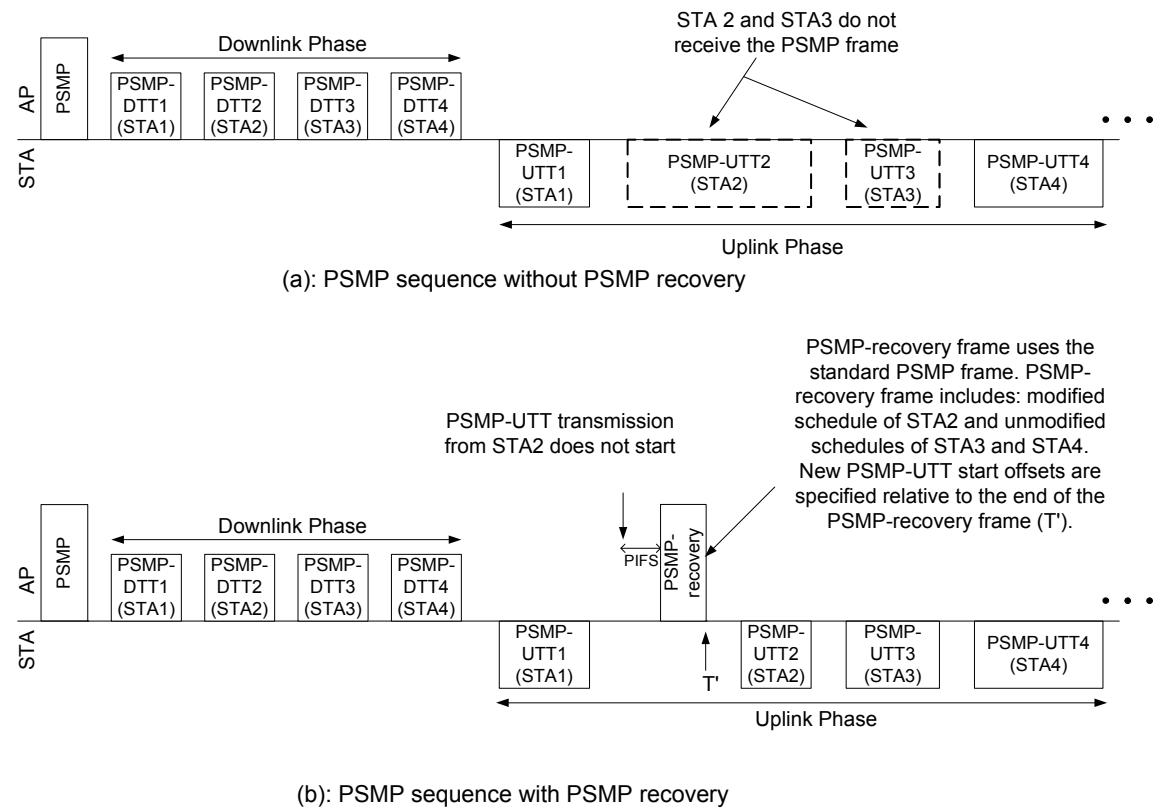
Figure 9-31—Illustration of PSMP sequence with and without PSMP recovery
