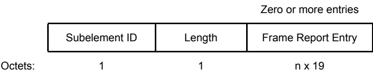
Figure 8-151—Frame Count Report subelement format
