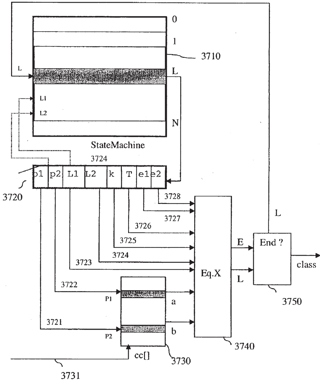
Figure 3h State machine
