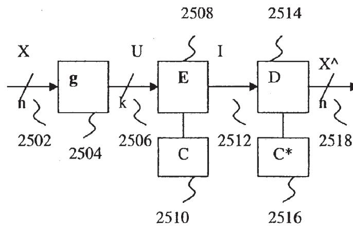
Figure 2f Gersho NLIVQ '90 (Fig.2)
