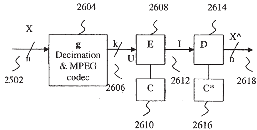
Figure 2g Gersho NLIVQ '90 adopted to interpolation of MPEG coded video
