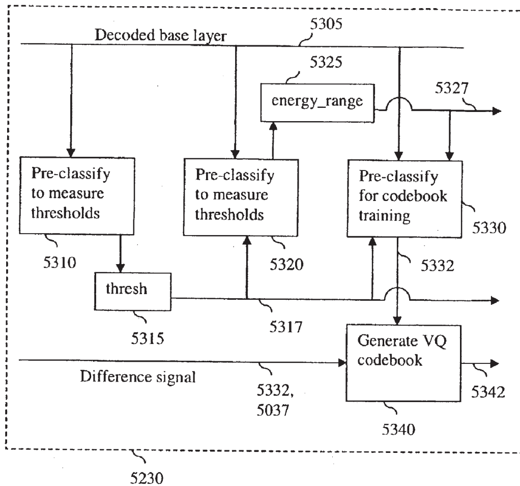
Figure 5d PHD pre-pass operations
