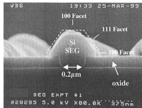
FIG. 3. SEG silicon grown from a 0.2-μm-wide seed hole.
