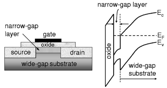
FIG. 19. A possible MOSFET structure that uses composite channel to enhance the mobility and reduce the BTBT current.
