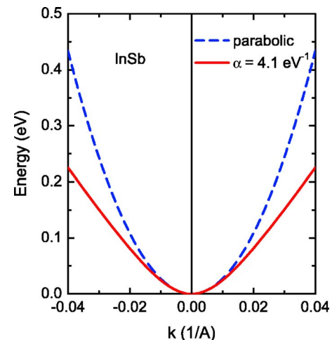
FIG. 16. Nonparabolic conduction band for InSb with parameter \alpha = 4.1 \text{ eV}^{-1} and the parabolic conduction band with effective mass m = 0.014m_0 .
