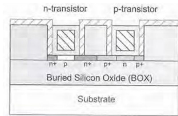
Weste, Figure 3.12
