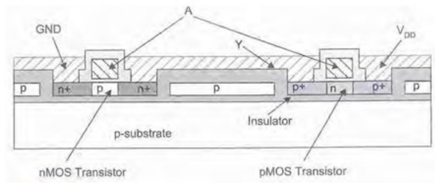
Weste, Figure 6.69
