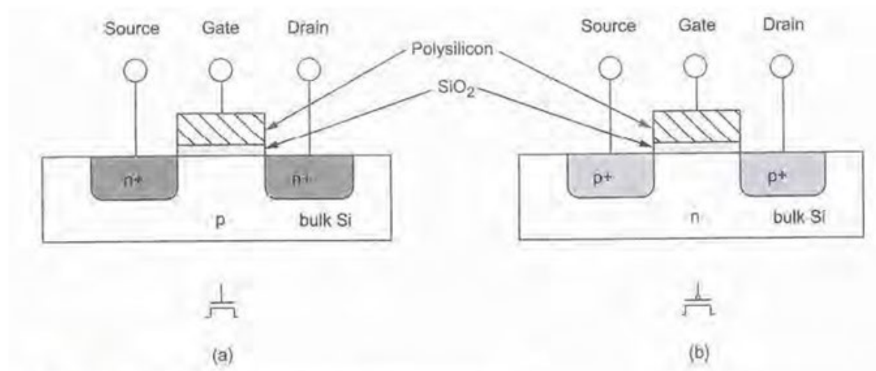
Weste, Figure 1.8
