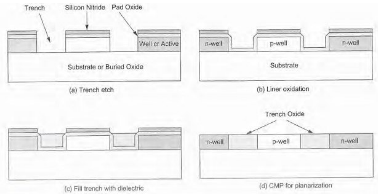
Weste, Figure 3.3
