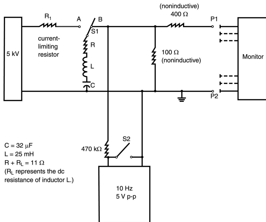
Figure 6—Test circuit for defibrillator energy-shunting test (5.2.5.2)—Switch S1 must withstand peak current of 60 A in the closed position and not break down for voltages up to 5000 V in the open position
