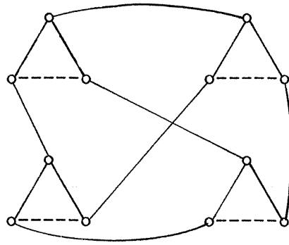
Figure 1. The Compound (12,3,3) of (3,2,1)
