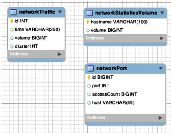
Fig. 3. Database Entity Relationship Diagram (ERD).
