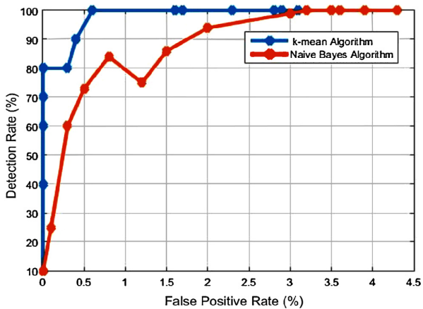
Fig. 13. ROC curve of our detection methods.
