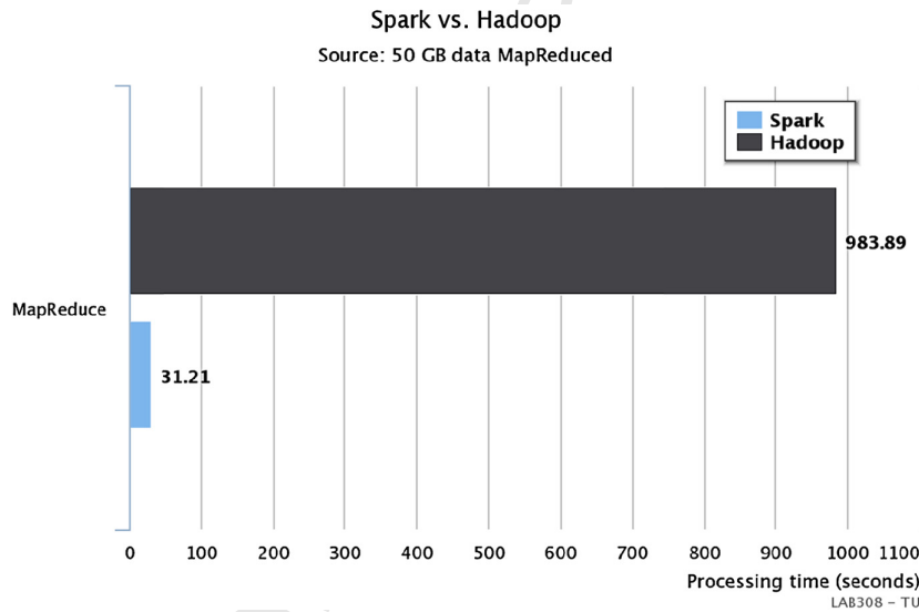
Fig. 16. Processing time comparison between Spark and Hadoop.
