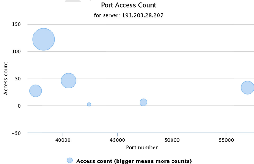
Fig. 14. Detection of port-scanning attack.
