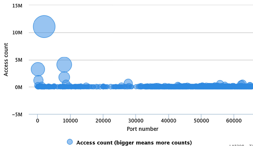
Fig. 9. The number of access in each port.
