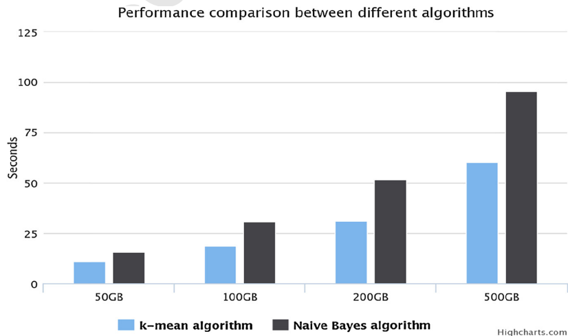
Fig. 17. Performance comparison between k-mean and Naive Bayes.
