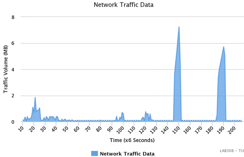
Fig. 10. Network traffic of simulated DDoS attacks.
