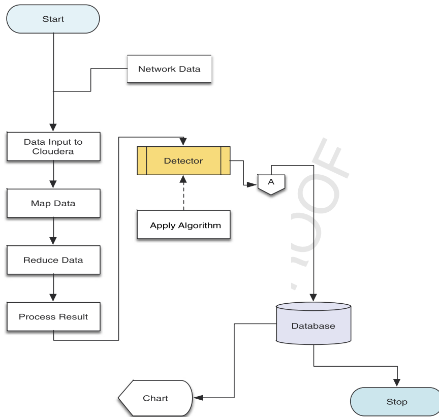
Fig. 2. System workflow.
