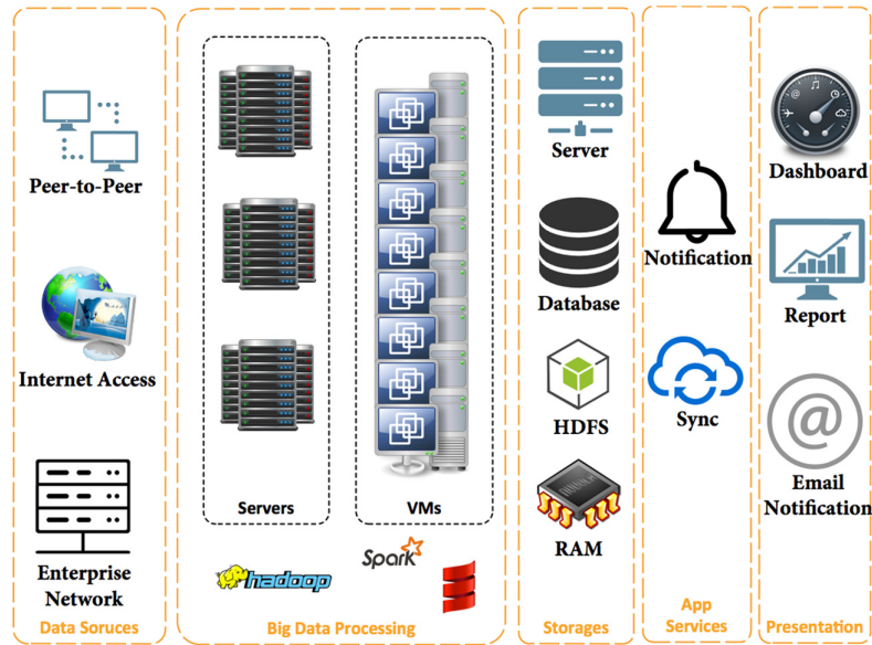
Fig. 5. Testbed setup.
