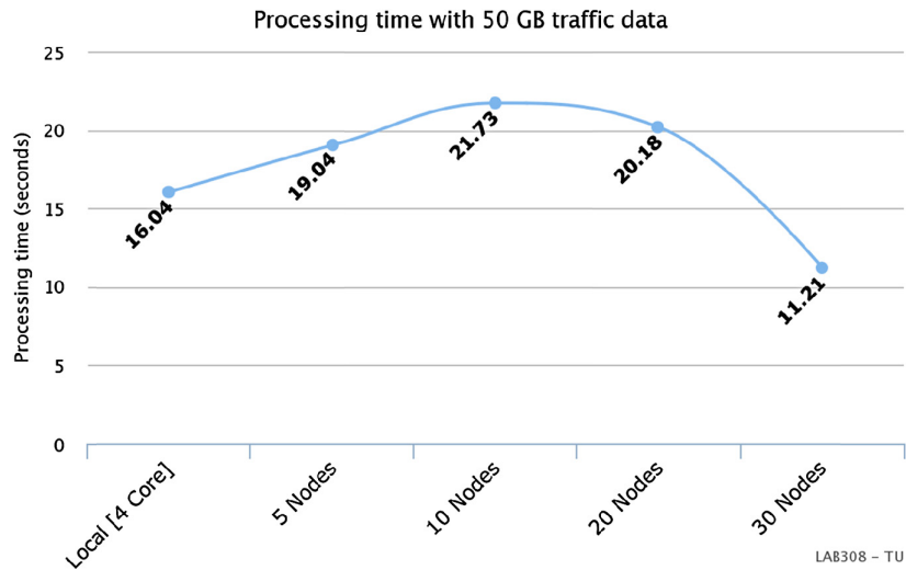
Fig. 15. Processing time of Spark.
