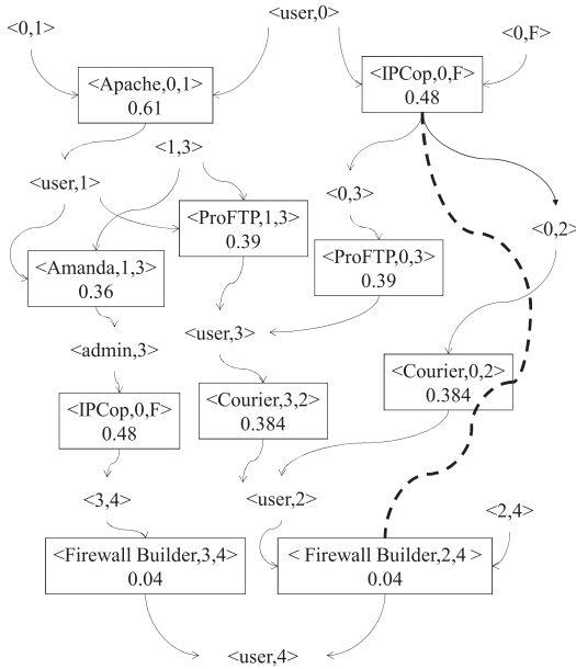
Fig. 3. The resource graph.
