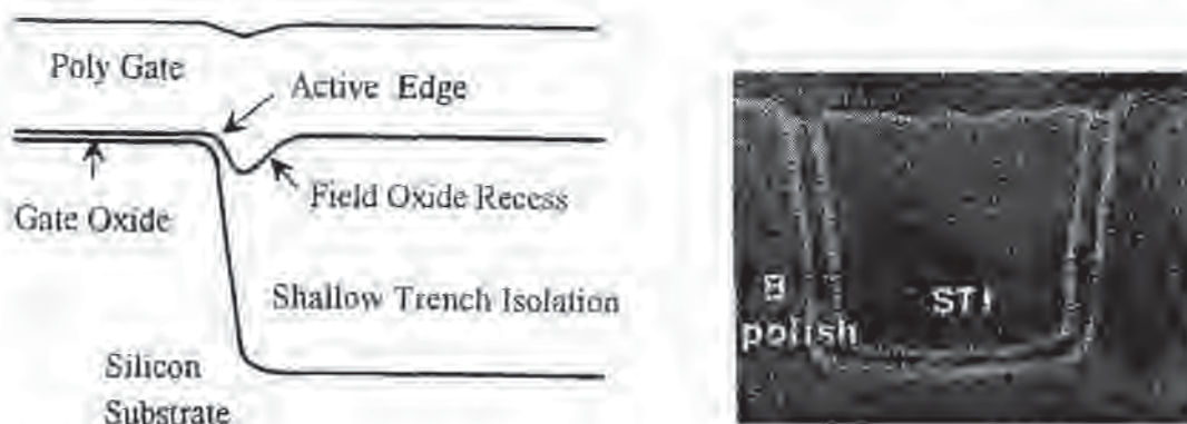
Fig. 9-30 Field-oxide recess (or divot ) formed at the active edge of an STI structure.
