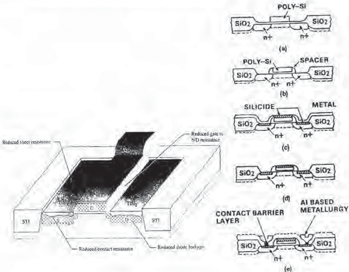
Fig. 13-4 Salicide processing steps and final structure.
