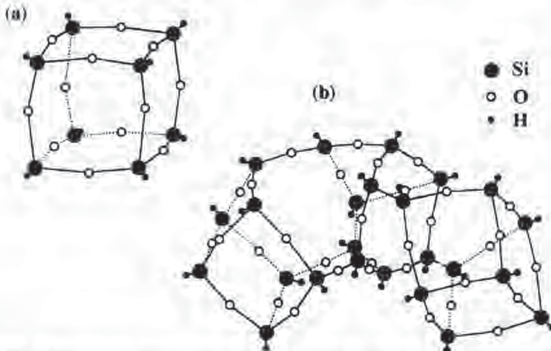
Fig. 14-5 Schematic representation of the molecular structure of HSQ: a) eight-corner oligomer; and b) resinous material.
