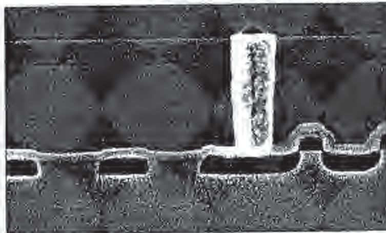
Fig. 9-4 SEM of a shallow-trench isolation structure.
