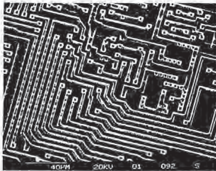
Fig. 12-3 SEM showing the patterned metal layer on a circuit with only one layer of metal.
