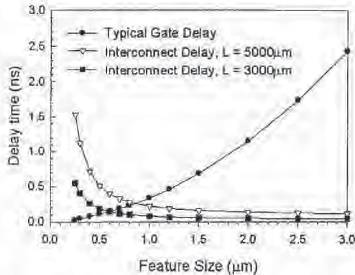
Fig. 12-23 Gate and interconnect delay versus feature size. Interconnect delay is shown for repeater spacings ( L ) of 3000- \mu\text{m} and 5000- \mu\text{m} . 14
