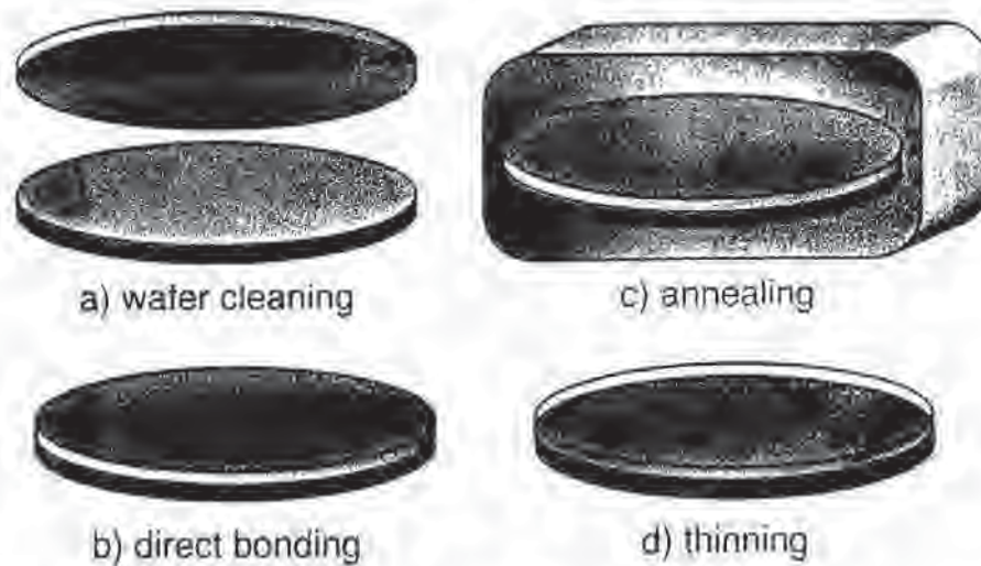
Fig. 11-21 Generic direct-wafer-bonding process flow.
