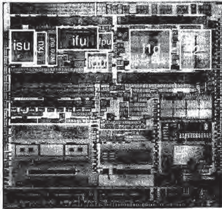
Fig. 11-20 Photograph of an IBM Power4™ processor using a SIMOX-SOI-based process, first bonded by applying pressure to the wafers at room temperature (Fig. 11-21). A subsequent furnace anneal is used to increase the bonding strength. After such bonding, most of the silicon from one of the wafers is removed, leaving a thinned
