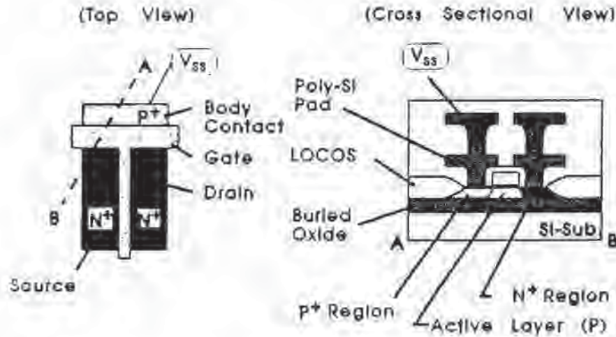
Fig. 11-10 A top-down and diagonal cross-sectional view of an SOI-NMOSFET with a body-contact made on one side of the MOSFET channel.
