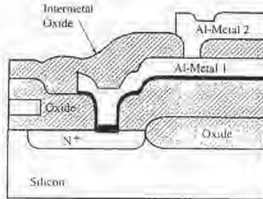
Fig. 12-4 Schematic of a double-level-metal structure used in early bipolar-ICs.
