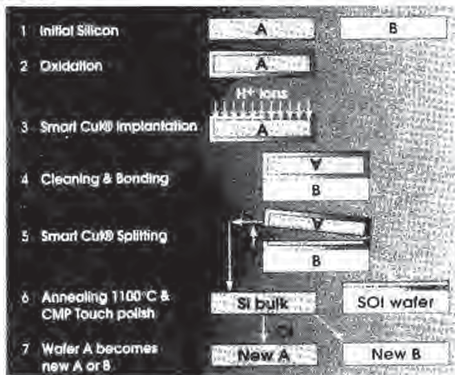
Fig. 11-24 Process flow for fabricating Smart-Cut ® wafers.
