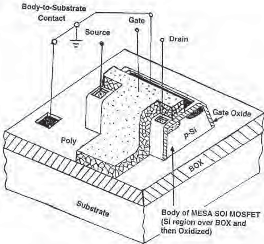
11-31 Mesa lateral-isolation SOI NMOSFET with a T-gate and body-to-substrate contact. when LOCOS is applied as the technique for producing lateral-isolation in SOI. These issues are discussed in this section.
