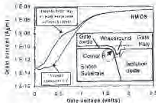
Fig. 9-29 “Kink” in MOSFET I_D - V_{GS} characteristic due to parasitic corner conduction caused by poly wraparound.
