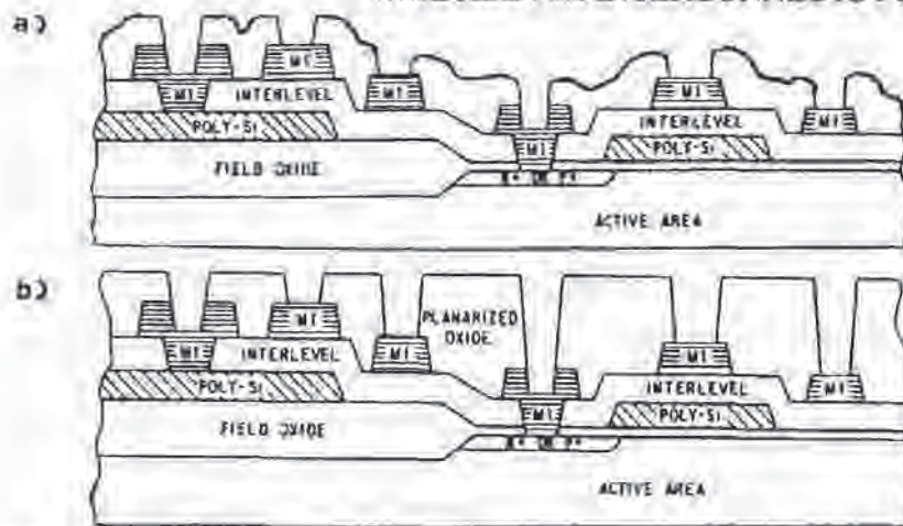
Fig. 12-10 a) If no planarization is used, the via and contact holes between adjacent conductor levels all have approximately the same depth; b) If planarization of the intermetal dielectric layer is achieved, the vias will vary widely in depth.
