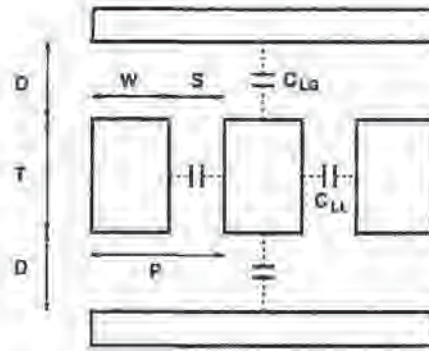
Fig. 12-10 Simplified RC -delay test-structure. 11 (© IEEE 1995)
