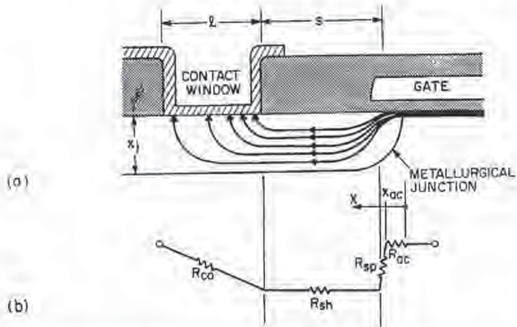
Fig. 11-4 Schematic drawing showing: a) current paths within the source and drain regions, of a planar MOSFET and; b) their corresponding representative series resistance components. 5 (© 1979 IEEE)
