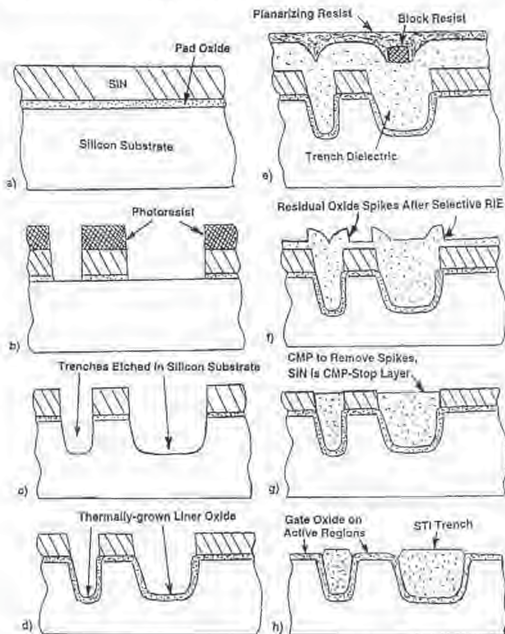
Fig. 9-10 Baseline process flow used to form an STI structure: a) Form pad oxide by thermal oxidation, then deposit a silicon-nitride layer by LPCVD; b) Pattern the nitride and pad-oxide layers; c) Etch trenches, strip resist; d) Grow liner-oxide on the trench walls, using thermal oxidation; e) Deposit the trench dielectric & densify it, then deposit a block-resist layer & pattern it. Finally deposit the planarizing resist layer; f) Use a selective-RIE-etch process to simultaneously remove the resist and the trench-oxide-layer, leaving residual oxide spikes; g) CMP the CVD-oxide-layer to abrade spikes and planarize its surface. The silicon nitride acts as a CMP-stop-layer; h) Strip the nitride and then grow the gate-oxide on active regions. The STI structure is now completed.
