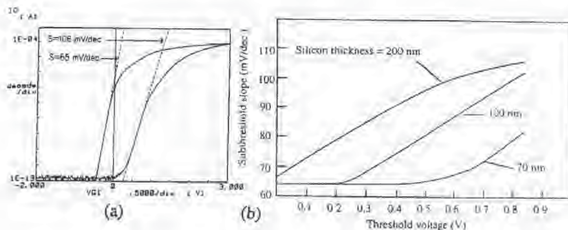
Fig. 11-12 a) Log-plot of drain-current I_D versus gate-voltage in SOI-MOSFETs made with two different silicon film thicknesses: 90-nm (left curve) and 450-nm (right curve). The inverse-subthreshold-slope, S_t (in millivolts per decade) is indicated. V_{DS} = 1 V; b) S_t as a function of threshold voltage for various SOI film thicknesses ( n -channel device).
