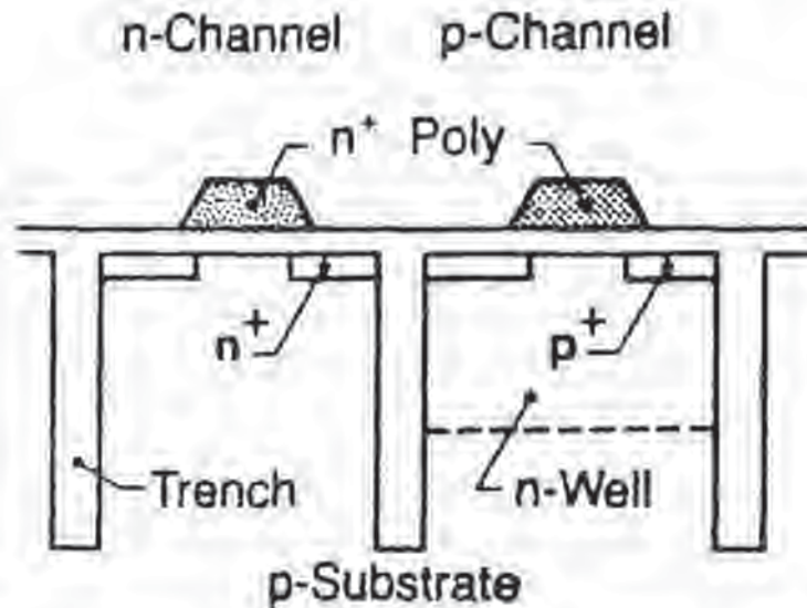
Fig. 9-5 Schematic of an n -well CMOS with deep trench isolation. 11 (© 1986 IEEE).
