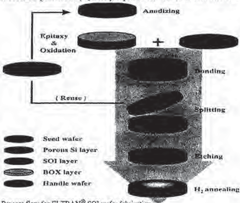
Fig. 11-28 Process flow for ELTRAN® SOI wafer fabrication.
