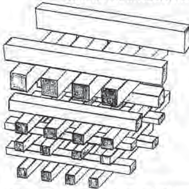
Fig. 12-14 Schematic showing the orthogonal architecture of multilevel interconnect lines.
