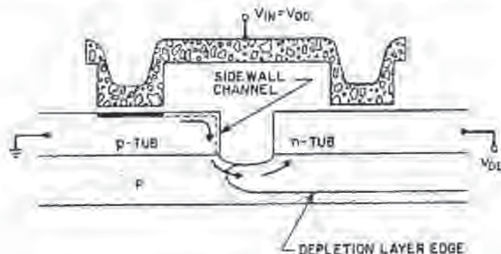
Fig. 9-7 A trench-isolated p -well and n -well with a parasitic vertical-sidewall-MOSFET (with the n -well as the gate) and a parasitic-horizontal-MOSFET (with the V_{in} poly-line as the gate). 14 From S.M. Sze Ed., High-Speed Semiconductor Devices , Copyright 1990 by John Wiley & Sons, Reprinted with permission.
