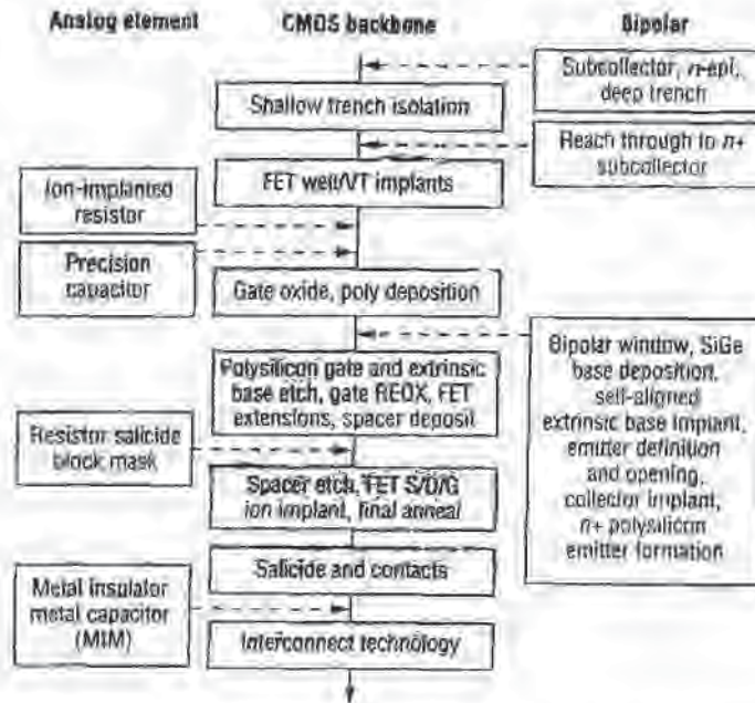
Fig. 10-8 CMOS process flow for fabricating Base-During-Gate Si:Ge BiCMOS structure. 29 used, including the use of titanium salicide. The metallization is planarized Al-Cu metal, patterned by RIE, with tungsten interlevel plugs. Fig. 10-10 shows a schematic cross-section of this BiCMOS structure.
