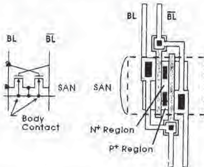
Fig. 11-11 Layout of a SOI-NMOSFET DRAM sense amplifier incorporating a body contact.
