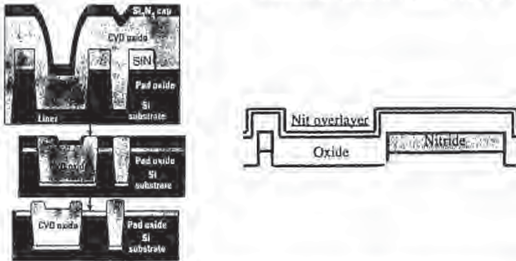
Fig. 9-27 Nitride cap approach to minimize dishing during CMP of the trench-fill oxide.
