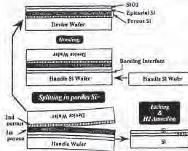
Fig. 11-29 The ELTRAN process flow for device wafer re-use. Bonded pairs are split within the porous-Si layer. The device wafer sides are used as a starting device wafer. The handle sides result in ELTRAN wafers after etching the porous-Si and H 2 -annealing.
