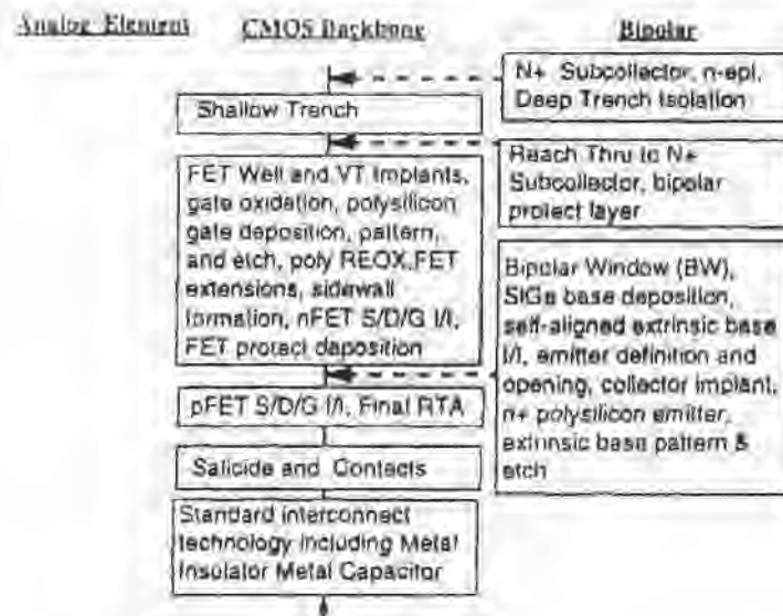
Fig. 10-9 CMOS process flow for fabricating base-after-gate Si:Ge BiCMOS structures. 29
