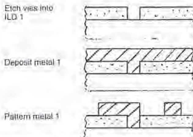
Fig. 12-2 Schematic of process steps used to produce a single-level-metal interconnect.
