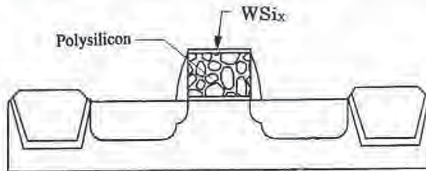
Fig. 13-1 Schematic cross-section of a polycide gate on a MOSFET.
