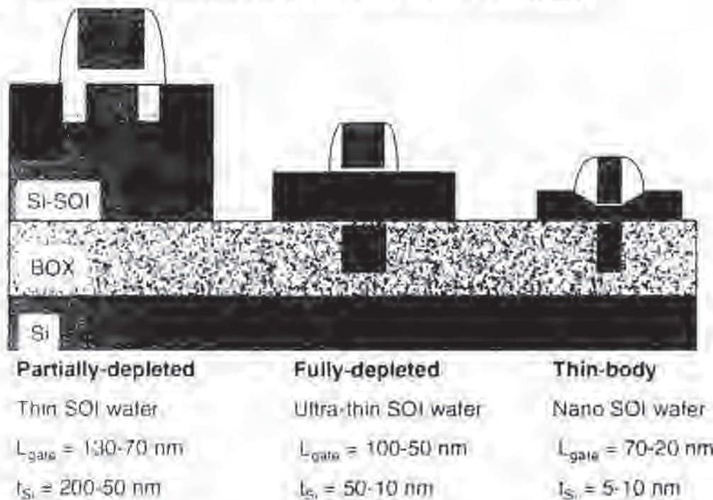
Fig. 11-13 Schematics of partially-, fully-depleted, and “thin-body” (double gate) SOI MOSFETs.
