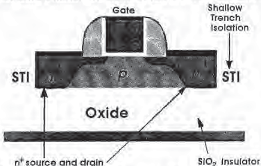
Fig. 11-1 Cross-section of a MOSFET fabricated on an SOI wafer.
