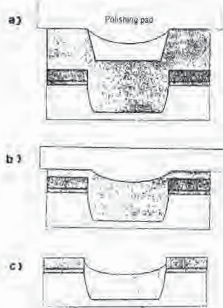
Fig. 9-23 Origin of the dishing effect in CMP: (a) polishing pad flexes into the trench opening; (b) formation of a concave surface; (c) trench area remains "dished" after planarization. Reprinted with permission of Solid State Technology. Published by PennWell.
