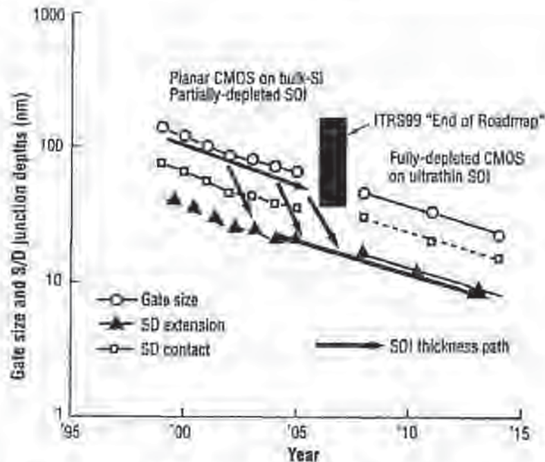
Fig. 11-7 Timeline of Si-SOI layer thickness linked to junction depth and gate size predictions from ITRS-2001.
