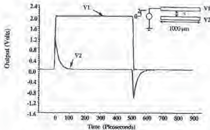
Fig. 12-24 Electrical modeling result showing the crosstalk voltage induced from a driven interconnect-line (V1) into an undriven line (V2) seeing a 20-psec waveform-edge. The lines were spaced at s = 1000\text{-nm} with a common length of 1-mm. 10
