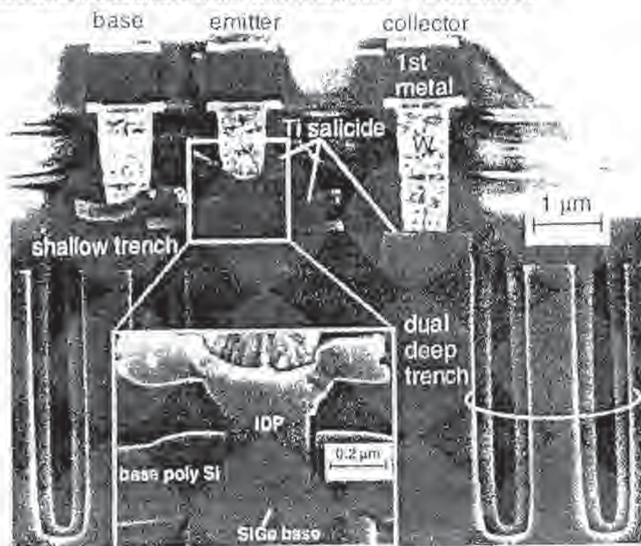
Fig. 10-1 SEM cross-sectional view of a 0.2- \mu\text{m} Si:Ge-HBT. 5
