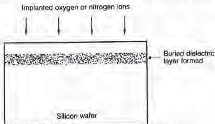
Fig. 11-18 Implanted oxygen ion process for the formation of a SIMOX wafer.
