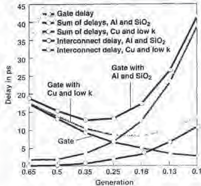
Fig. 12-1 RC-delay as a function of feature size. 1 (© IEEE 1997)
