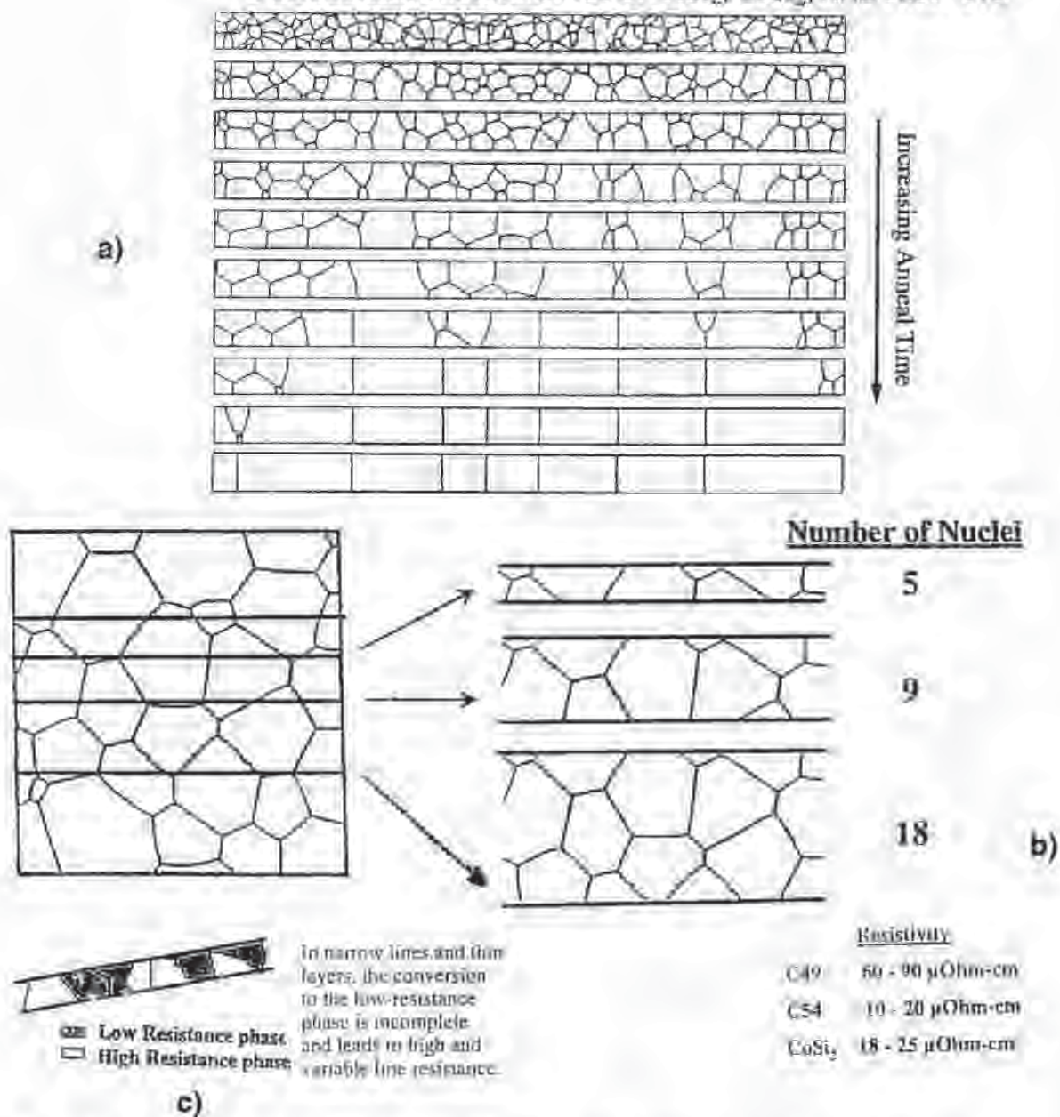
Fig. 13-7 a) Simulation of grain-growth within a line with increasing annealing time, starting with small grains; b) When the as-deposited grains are already large (relative to the line width) few nucleation sites for the C-54 phase exist. In fact, the narrower the line, the fewer the number of nuclei; c) Thus, the conversion to C-54-phase from C-49-phase is incomplete, and the final \text{TiSi}_2 sheet-resistance is a combination of low and high resistance phases, and is therefore higher (and variable).
