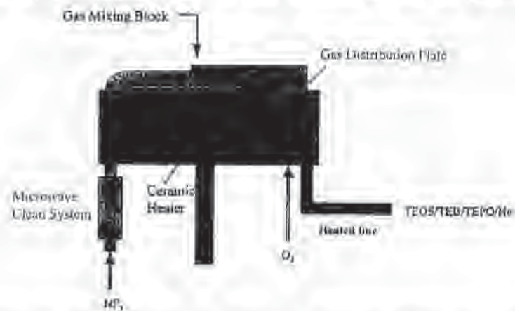
Fig. 9-19 Schematic of Applied Materials SACVD Giga-Fill BPSG chamber, equipped with a high-temperature heater and remote microwave system for predeposition cleaning. 34
