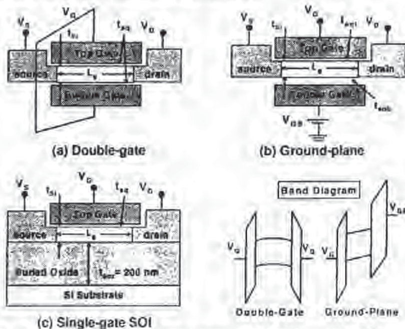
Fig. 11-37 a) Double-gate; b) Ground-plane; c) Single-gated SOI-MOSFET. Gate material work-function is set at the mid-gap of the silicon band gap. On-chip biasing of the ground plane is assumed. The source/drain junction is abrupt. The channel length ( L_g ) is the metallurgical channel length. (© 1998 IEEE). 57
