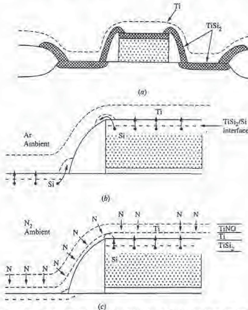
Fig. 13-5 “Bridging” during the formation of Ti salicide: a) \text{TiSi}_2 bridges over sidewall spacer and a short circuit is formed between the source-and-gate and the drain-and-gate; b) During \text{TiSi}_2 formation, Si diffuses into the Ti to form \text{TiSi}_2 . Under favorable conditions, Ti can diffuse a long distance and form \text{TiSi}_2 on the sidewall spacer; c) In a nitrogen ambient, nitrogen diffuses into the Ti and blocks the diffusion of Si, reducing or eliminating bridging. TiN and/or Ti-O-N are formed on top of the \text{TiSi}_2 .
