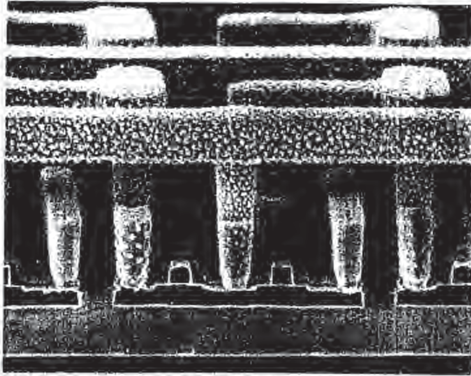
Fig. 11-16 SEM of completely fabricated SOI-MOSFET.
