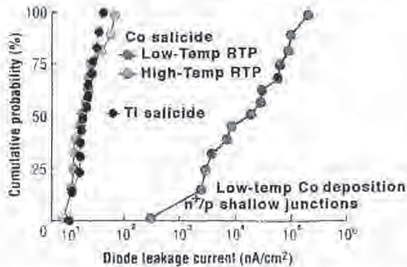
Fig. 13-11 High-temperature RTP is effective in improving diode-leakage in MOSFETs fabricated with \text{CoSi}_2 by eliminating high-leakage outliers.
