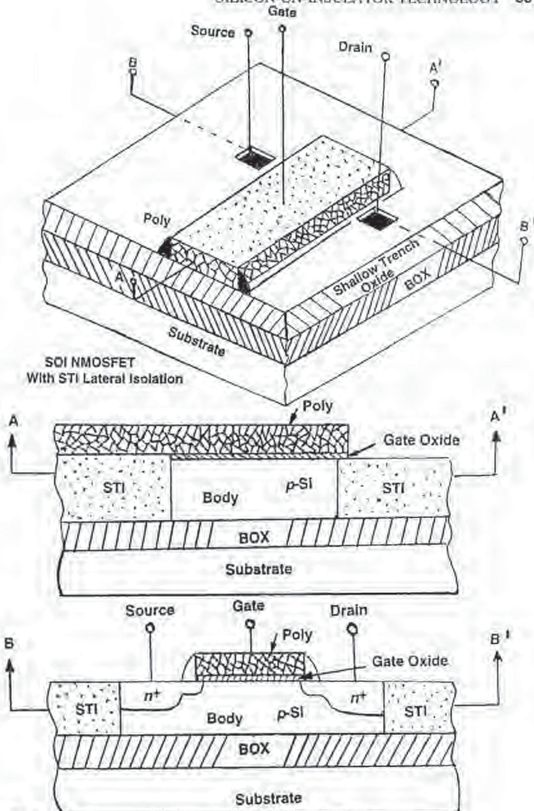
Fig. 11-33 Shallow-trench isolation (STI) lateral isolation SOI MOSFET.
