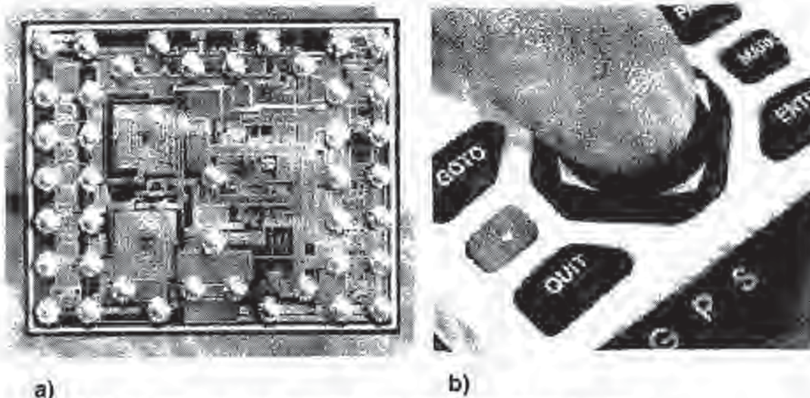
Fig. 10-11 a) Single-chip GPS Receiver; b) Relative size of GPS Receiver. 8
