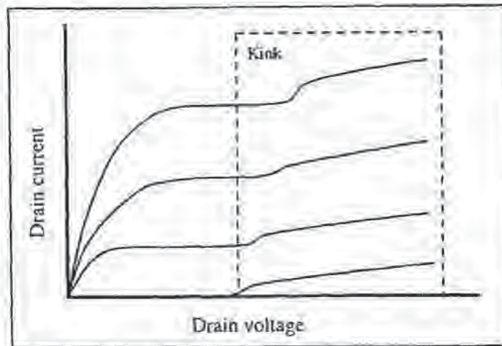
Fig. 11-34 Illustration of the kink-effect in the output characteristics of a partially-depleted SOI-MOSFET.
