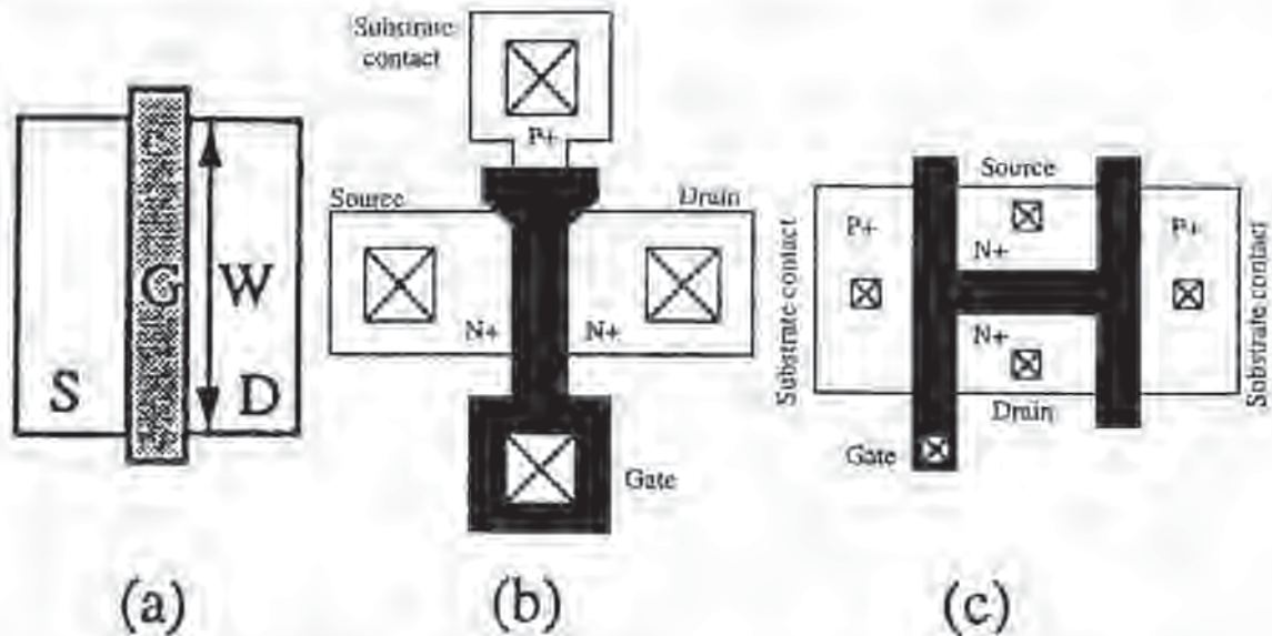
Fig. 11-9 a) Top-down view of an SOI-MOSFET in which no provision is made for contacting the body. Unless a contact to some circuit potential is explicitly provided, the potential of the SOI-body is floating; b) MOSFET with body-contact made on one side of the MOSFET channel; c) An "H-gate" SOI-MOSFET (i.e., a body-contact is made on each side of the MOSFET channel).
