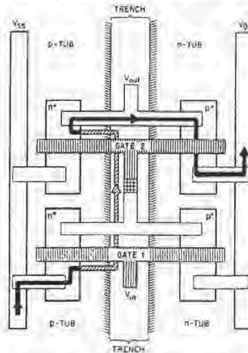
Fig. 9-8 A dc leakage path through two inverter stages in series. The solid black path is a good conducting route and the shaded path is a parasitic route. The parasitic consists of a field oxide corner under Gate-1 (cf. Fig. 9-7), a sidewall path along the trench (cf. Fig. 9-6a), and a corner path under the V_{out} strap. 15 From S.M. Sze Ed., High-Speed Semiconductor Devices , Copyright 1990 John Wiley & Sons, Reprinted by permission.
