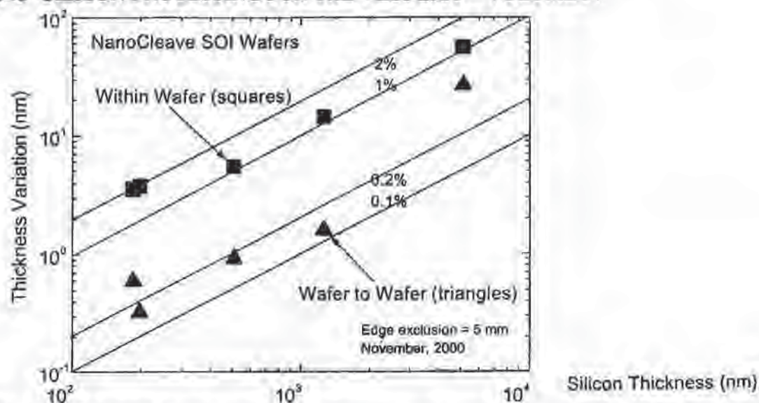
Fig. 11-27 Si-SOI layer-thickness-uniformity and average layer-thickness-control for post-cleave thickening of as-cleaved SOI-wafers with cleaved 200-nm Si-SOI-layers. 63
