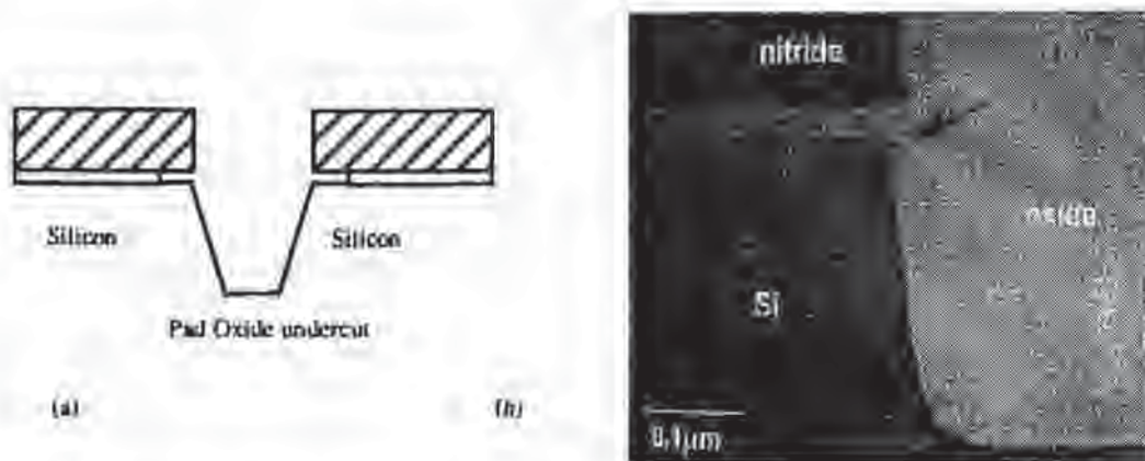
Fig. 9-12 a) Pad-oxide trench-undercut in the STI-baseline process. b) TEM of an as-etched trench profile showing the sharp corner of the active Si region at the top of the trench.
