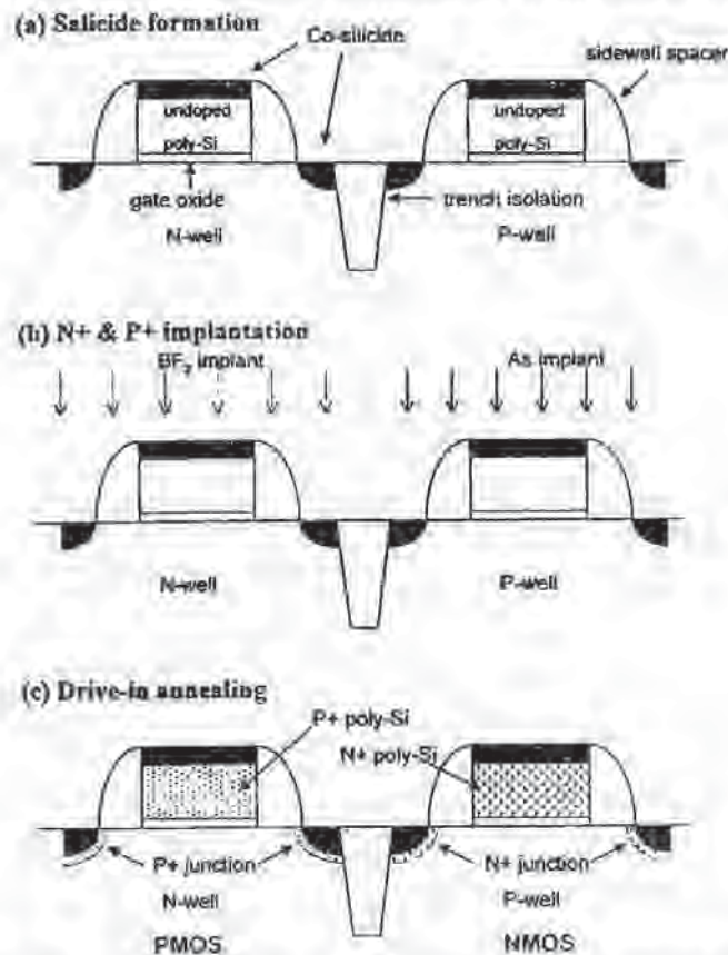
Fig. 13-14 Schematic of a process flow of 0.18\text{-}\mu\text{m} salicided dual-doped-gate CMOS using Co-silicide as the doping source.
