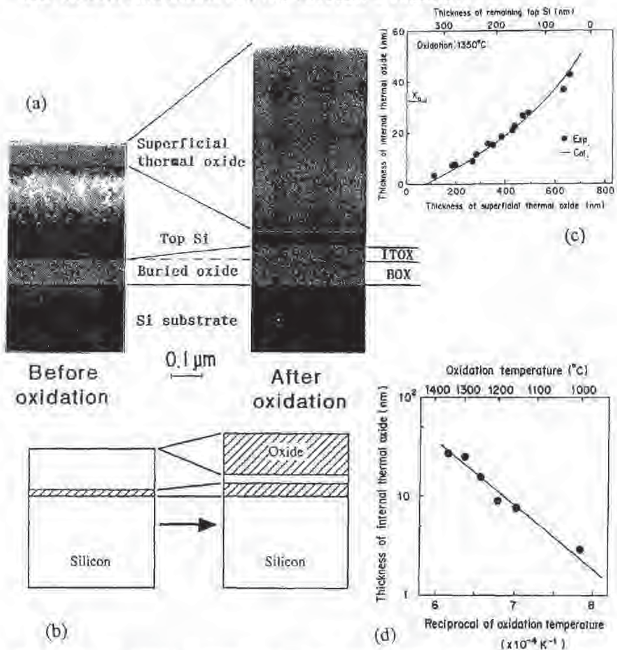
Fig. 11-19 a) An XTEM of SIMOX wafers before and after high-temperature-oxidation at 1350°C; b) A schematic drawing of SIMOX wafers before and after high-temperature oxidation at 1350°C; c) Relationship between the thickness of the ITOX layer and the superficial thermal-oxide-layer formed by high-temperature-oxidation at 1350°C; d) Relationship between the thickness of the ITOX-layer and the reciprocal of the oxidation-temperature.
