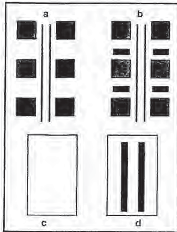
Fig. 9-26 Dummy (b) and dishing support features of small (a) and large wafer (c) features can prevent dishing. 50 Reprinted by permission of Semiconductor International.
