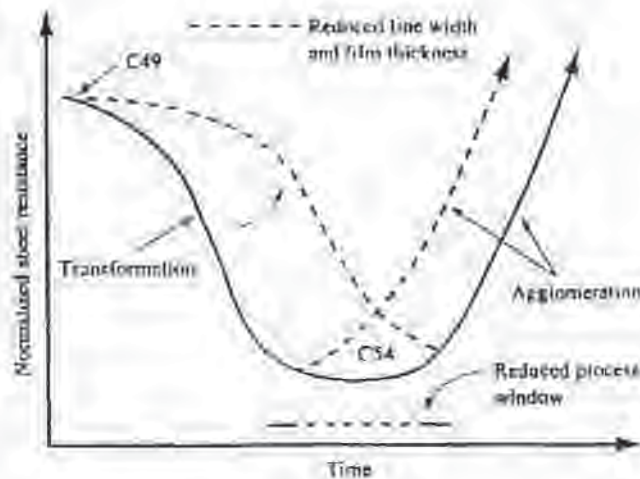
Fig. 13-8 For a thinner polysilicon line, the time required to transform the C-49-phase to the C-54-phase increases (i.e., at some chosen, constant temperature), but the time it takes for the \text{TiSi}_2 film on the line to undergo agglomeration decreases as the line width is decreased. Hence, the process-window for forming C-54-phase on thinner lines eventually closes.
