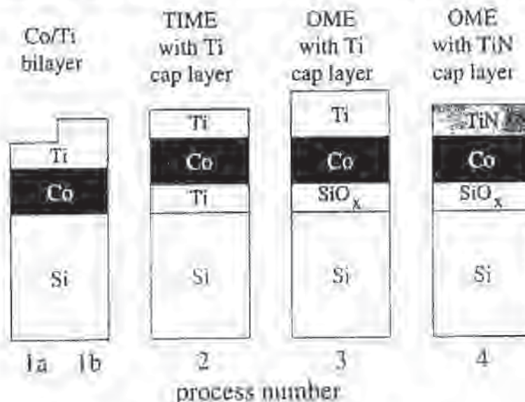
Fig. 13-13 Different silicide techniques; thicknesses are not scaled.
