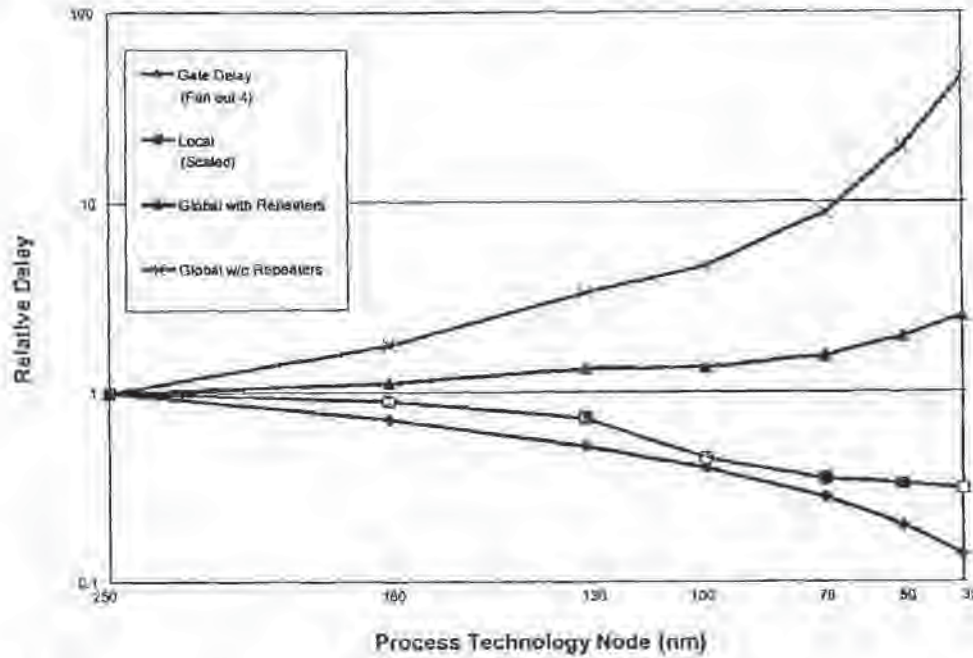
Fig. 12-20 Interconnect versus delay, from ITRS99. 3
