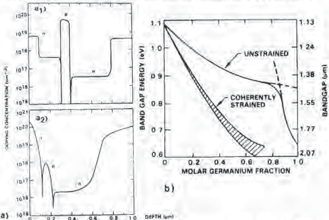
Fig. 10-3 a) Representative doping profiles for npn heterojunction bipolar transistors. 9 (© 1989 IEEE); b) Band-gap energy versus alloy composition for Si:Ge alloys. 19 (after People and Bean Copyright 1986 AIOP)
