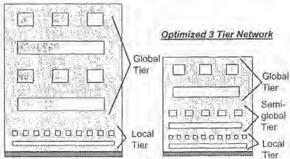
Fig. 12-18 The architecture of interconnects also utilizes a hierarchy of tiers.
