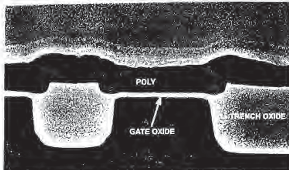
Fig. 9-14 SEM showing polysilicon crossing the region at the edge of the active device region and the trench in an STI structure.
