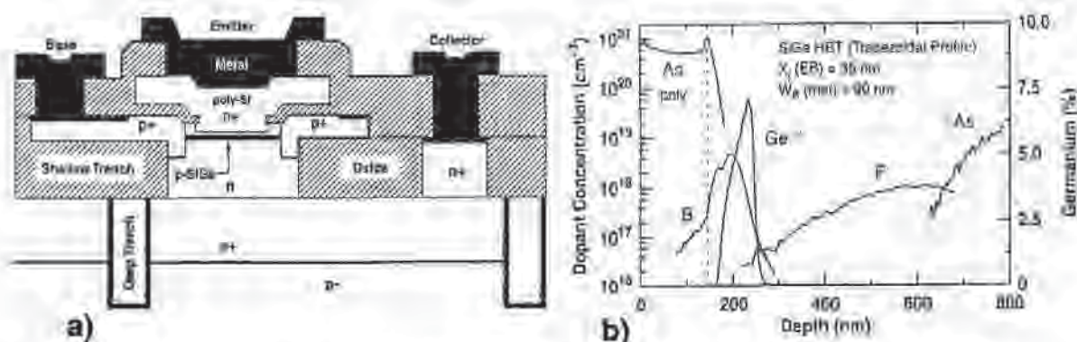
Fig. 10-12 a) Schematic cross-section of deep-submicron Si:Ge HBT; b) SIMS doping profiles of the deep-submicron Si:Ge HBT. 41 (© 2002 IEEE)
