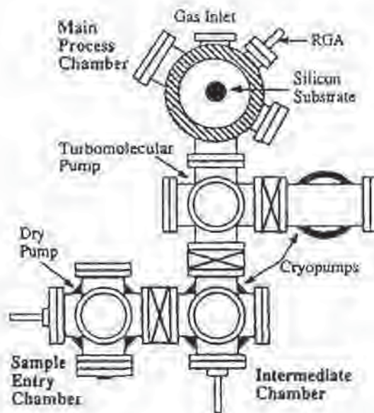
Fig. 10-6 Schematic of a UHV/RTCVD epitaxial system. 22 Reprinted with permission of the American Physical Society.
