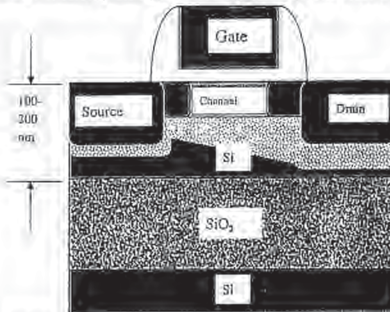
Fig. 11-8 Partially-depleted transistor in a Si layer over an isolation layer.
