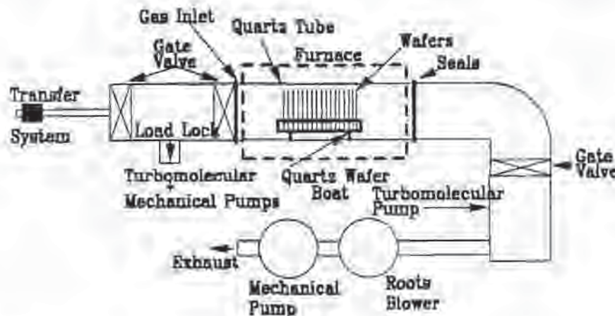
Fig. 10-4 Cross-section schematic of a UHV/CVD reactor. 15
