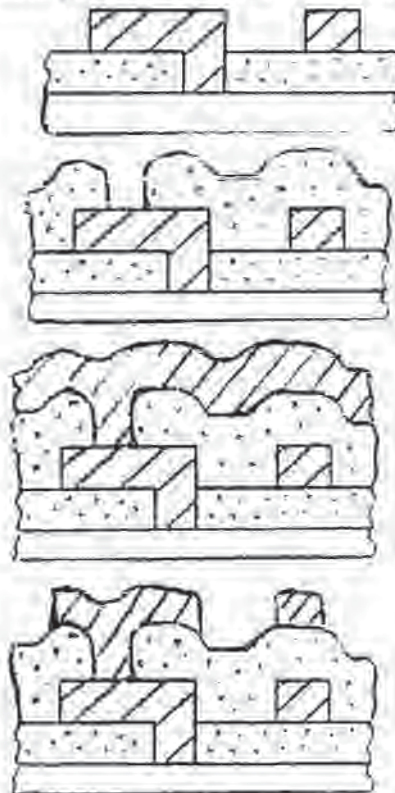
Fig. 12-5 Schematic drawing of the sequence of process steps used to produce a double-level-metal interconnect structure as shown in Fig. 12-4.
