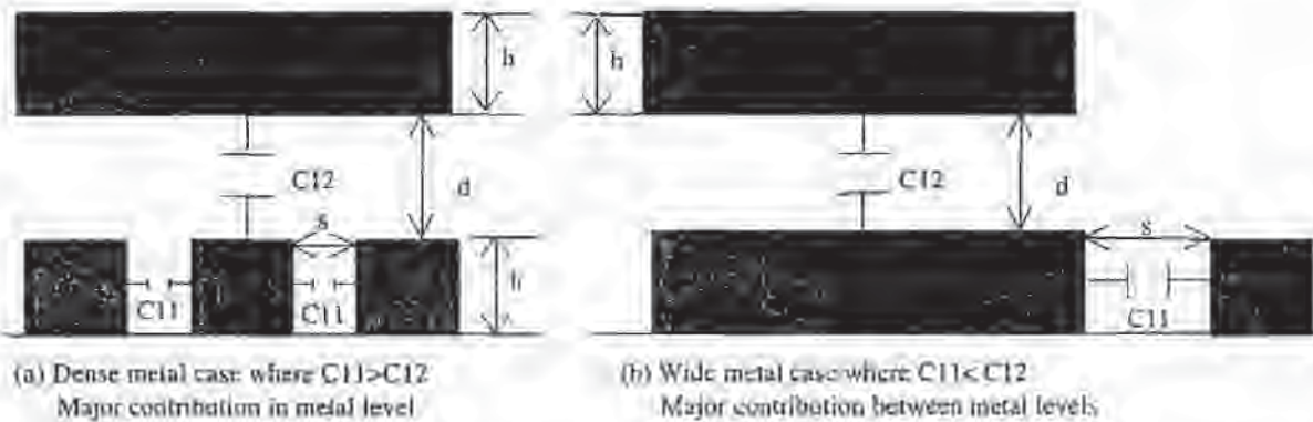
Fig. 12-21 Capacitance coupling contributions for interconnect systems: a) Dense interconnect case where major coupling is between minimum-spaced lines; and b) Wide interconnect lines where the major coupling is between metal-levels.
