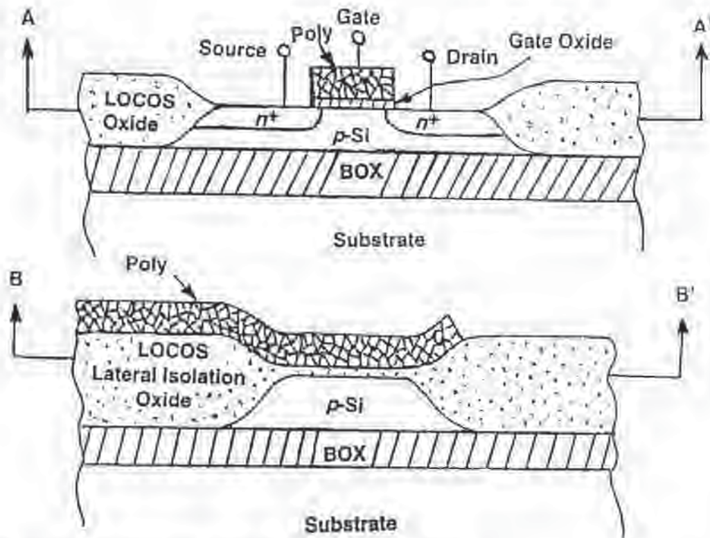
Fig. 11-32 SOI-MOSFET that uses LOCOS lateral isolation.
