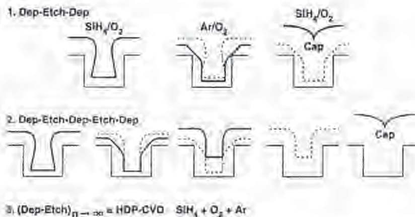
Fig. 9-20 High-density plasma CVD achieves good gap filling through simultaneous deposition and etching. The deposition-to-etch-ratio is usually kept between 0.14 and 0.33. 43 Reprinted with permission of Semiconductor International.
