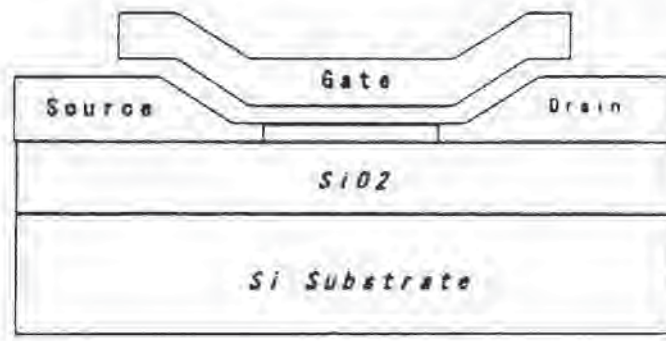
Fig. 11-15 Cross-section of a LOCOS-thinned "thin-body" SOI MOSFET.
