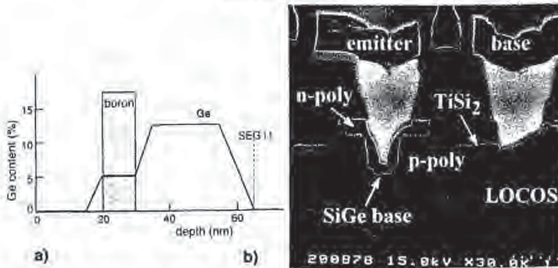
Fig. 10-7 a) Schematic of the Ge profile in the Si/SiGe layer of a SiGe-HBT. 27 b) SEM cross-section of the emitter-base complex of a 0.2- \mu\text{m} SiGe-HBT. 26
