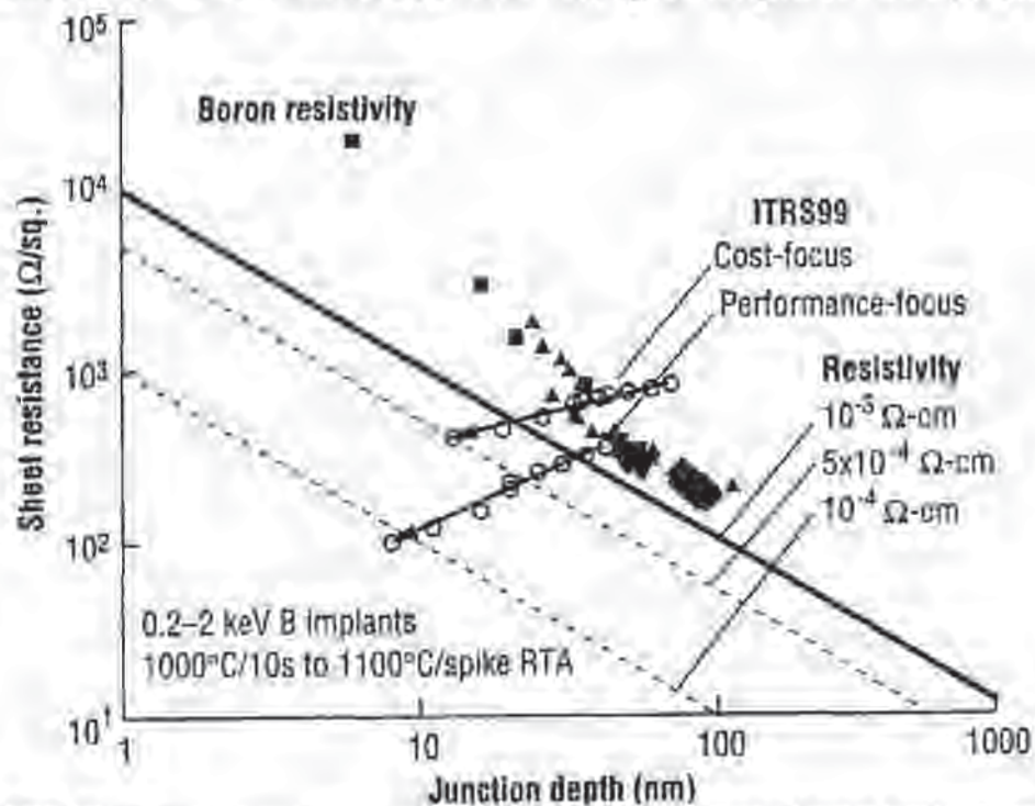
Fig. 11-3 Sheet-resistance and junction-depths for low-energy boron implants and spike-implant anneals, and industry expectations for S/D extension junctions (starting with 140-nm gates to 22-nm gates at the head of the arrows) for cost-focus and performance focus devices. The dopant resistivity for sub-keV boron implant and spike-RTP process (in CZ-Si) is limited by a "wall" at about 10^{-3} \Omega\text{-cm} .
