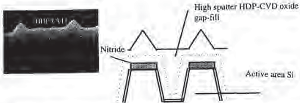
Fig. 9-21 The surface topography of a dielectric film deposited by HDP-CVD showing the sharp spikes that remain as a result of the dep-etch nature of the HDP-CVD process.
