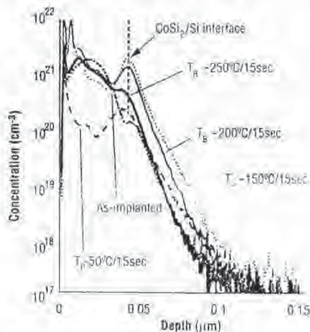
Fig. 13-15 Shallow junctions obtained using \text{CoSi}_2 as a diffusion source (SADS) process.
