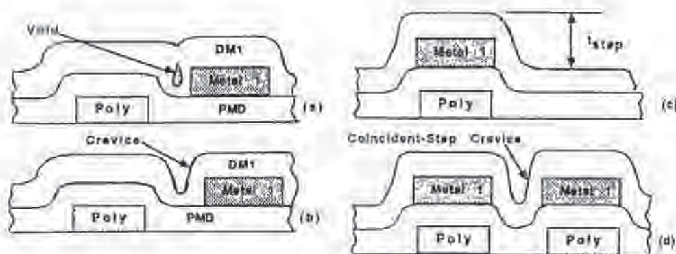
Fig. 12-6 Topography conditions that arise in MOSFETs that make it difficult to fabricate a double-level-metal structure without some kind of planarization method.
