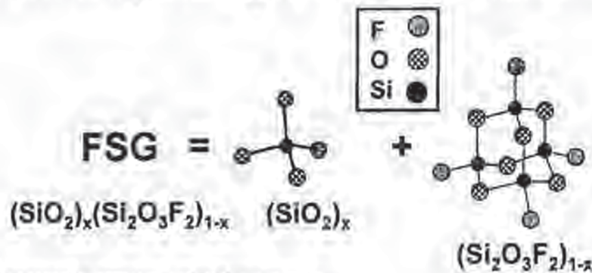
Fig. 14-6 Molecular structure of FSG materials.
