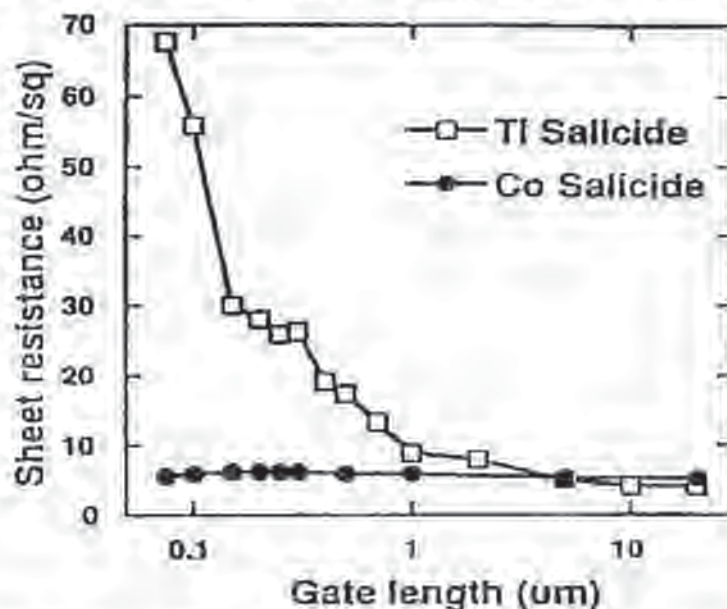
Fig. 13-6 The \text{TiSi}_2 narrow-width effect: As the polysilicon lines onto which the \text{TiSi}_2 is formed are made smaller (i.e., < 1\text{ }\mu\text{m} ), the sheet resistivity of the \text{TiSi}_2 increases.
