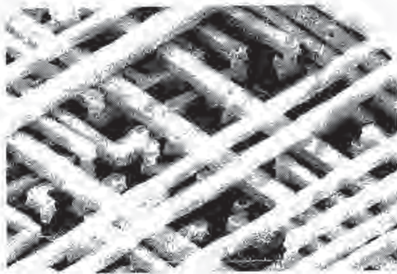
Fig. 12-15 SEM of orthogonal architecture of metal lines in a W-plug/Al interconnect.. that contains a third, semi-global tier , as shown in Fig. 12-18b).
