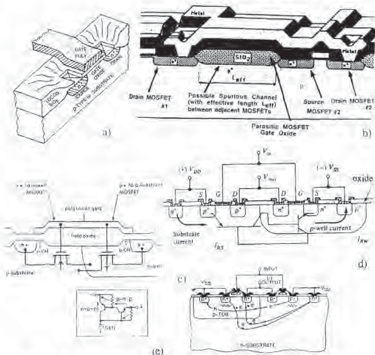
Fig. 11-2 a) A single MOSFET built in a bulk-silicon substrate, with various device structures and regions defined; b) Two MOSFETs (e.g., both NMOSFETs) built in a substrate having one type of doping (i.e., on a p -doped substrate), together with the parasitic transistor that exists in the field-region separating these MOSFETs. Semirecessed-LOCOS is used to produce the field-oxide (which is part of the device structure employed to maintain electrical isolation among such MOSFETs); c) An n -well CMOS structure fabricated in a p -type bulk-silicon wafer. Also shown in the figure are the parasitic MOSFETs that are associated with that structure, as well as the pn junction that separates the n -wells from the p -substrate; d) A cross-section of a CMOS-IC-structure is depicted, together with a schematic depiction of the parasitic-bipolar-transistors and associated lateral currents; e) The parasitic bipolar transistors that exist in CMOS structures can be turned on , which can cause the CMOS IC to go into a latchup state.
