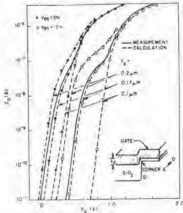
Fig. 9-3 Measured and simulated drain current versus gate potential for devices having a downward step in the field oxide ( t_d ). 9 (© 1981 IEEE)
