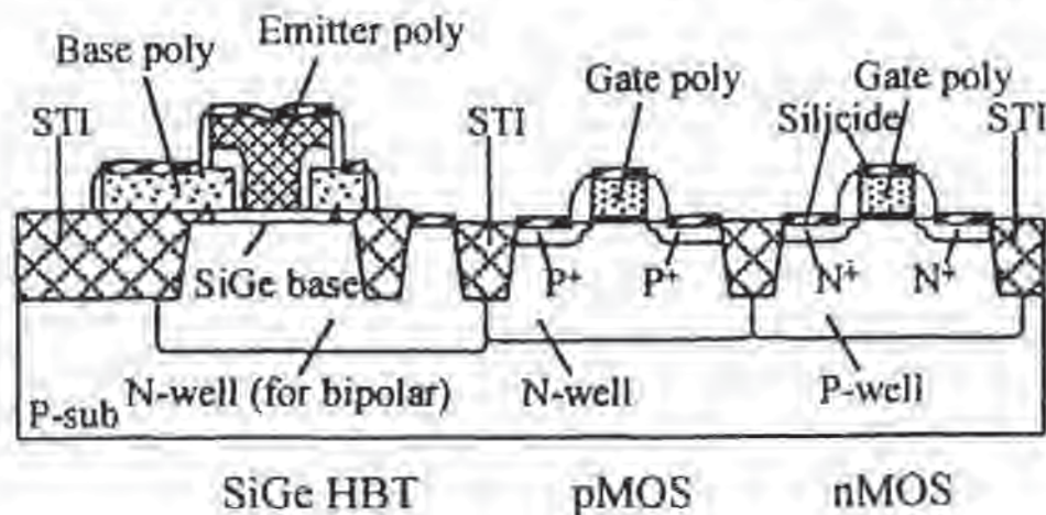
Fig. 10-10 Schematic cross-sectional view of the Si:Ge BiCMOS. The Si:Ge HBT has a self-aligned structure. 16
