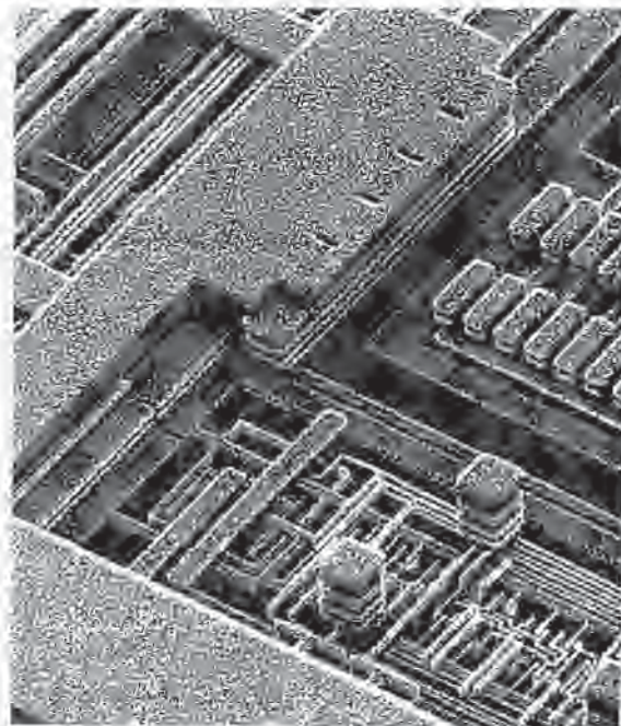
Fig. 12-16 SEM of orthogonal architecture of metal lines in a Cu interconnect.
