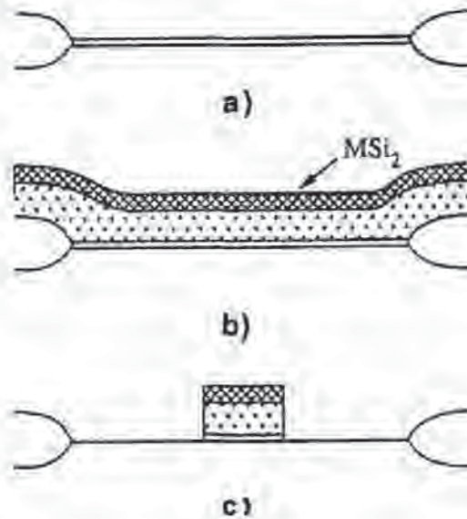
Fig. 13-2 Process sequence for producing a \text{WSi}_x -polycide-structure: a) Gate oxide growth; b) Polysilicon and \text{WSi}_x deposition by CVD; c) Patterning the polycide.
