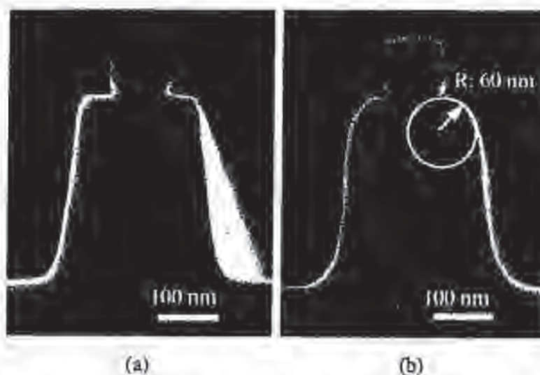
Fig. 9-18 Cross-sectional SEM of before (a) and after (b) H_2 -annealing. Annealing condition was 950°C, 380 torr, 60 sec. Silicon migration phenomenon can round out STI's top-corner-rounding-radius up to 60-nm. 32 (© IEEE 1998)
