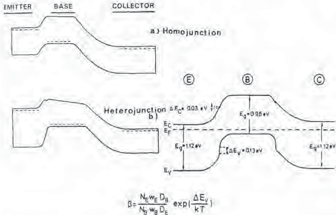
Fig. 10-2 Band diagrams of representative npn: a) homojunction, and; b) heterojunction bipolar transistors. 9 (© 1989 IEEE)
