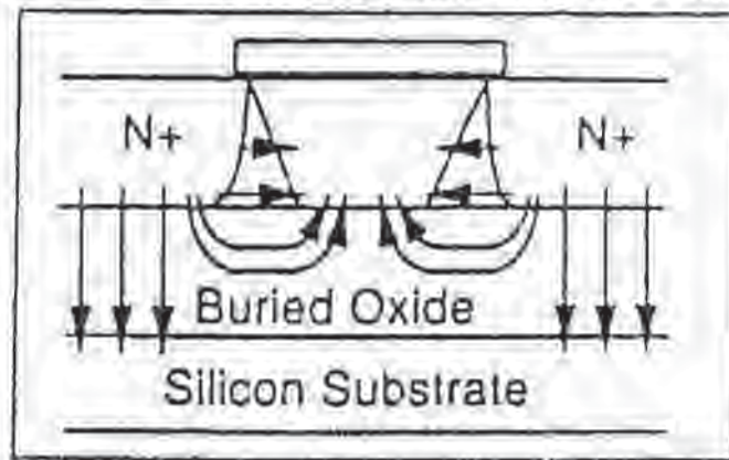
Fig. 11-36 Electric-field lines in the source/drain and body pn -junctions in a short-channel SOI-MOSFET. Some of these lines terminate in the substrate beneath the buried-oxide (BOX), while others terminate in the body, producing fringing-electric-fields. 55
