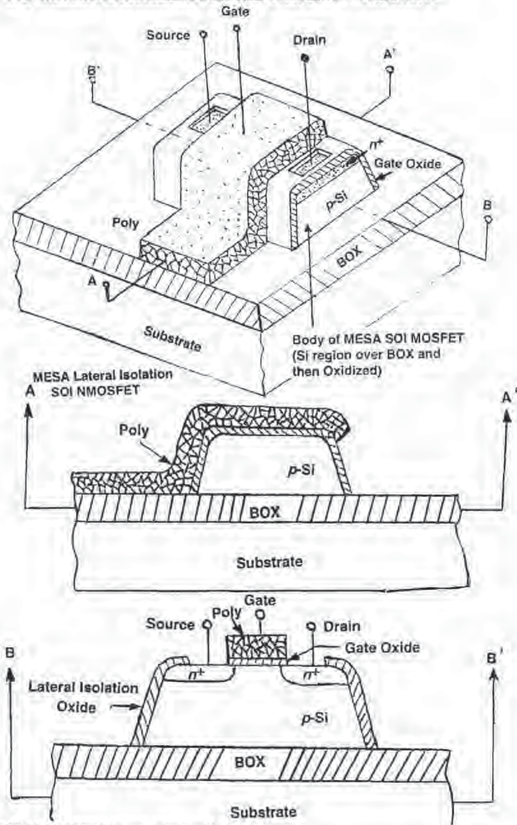
Fig. 11-30 MESA lateral isolation SOI NMOSFET.
