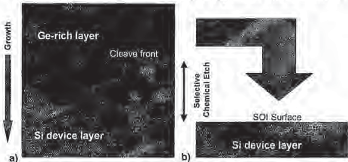
Fig. 11-26 a) HR-TEM image of the boundary area of a Ge-rich, epitaxial strain-layer and a crystalline-Si-device-layer in a state prior to atomic-layer-cleaving; b) The residual Ge-rich layer on the as-cleaved-wafers are subsequently removed through a selective etch step.
