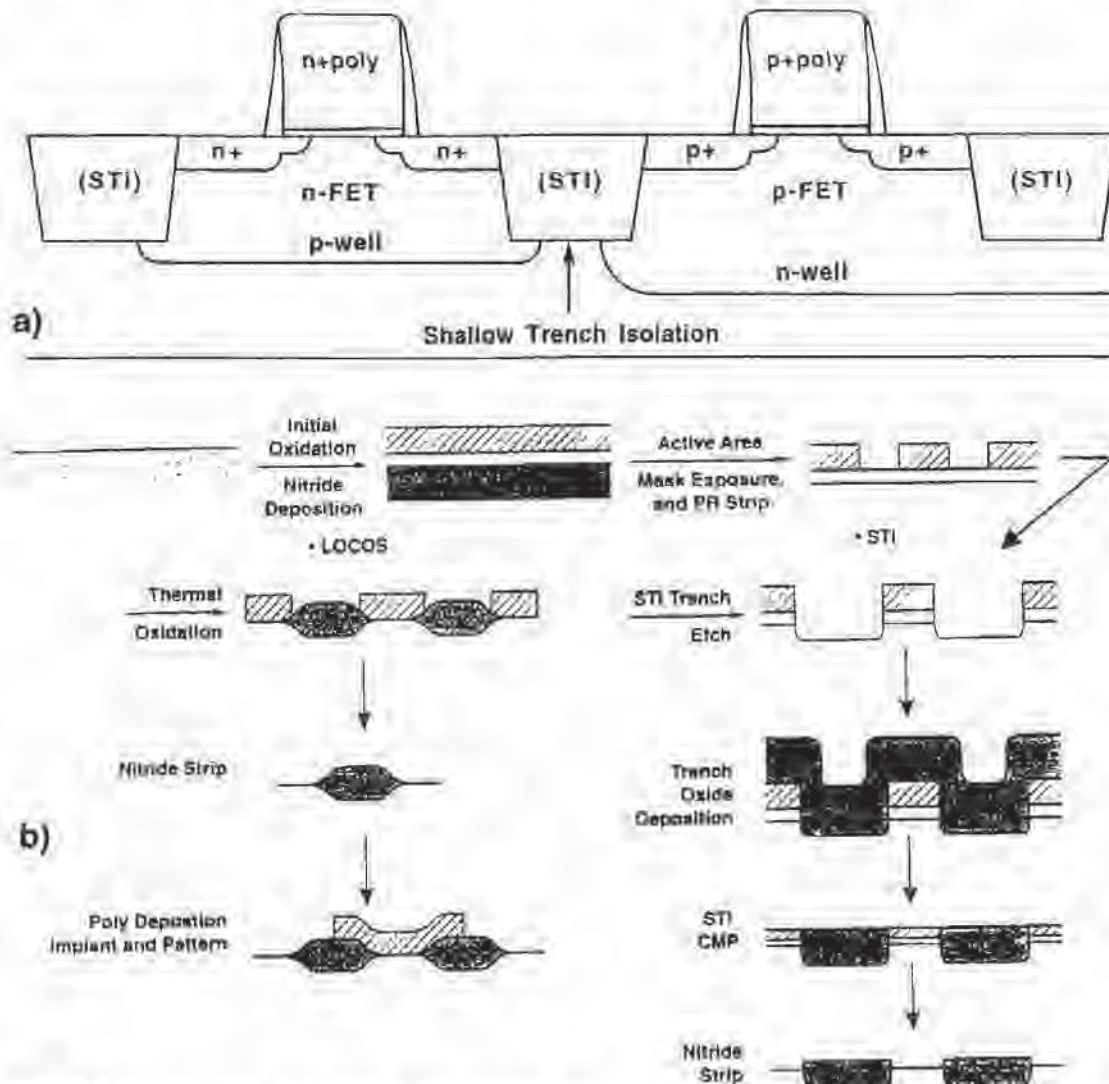
Fig. 9-1 a) Schematic of STI in a CMOS structure. b) LOCOS vs. STI process flow, indicating that STI requires more steps.
