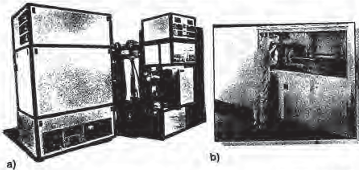
Fig. 10-5 a) Commercial UHV/CVD Si-Ge deposition system. Courtesy of CVD Systems; b) Commercial Low-energy plasma-enhanced CVD system for Si-Ge deposition. Courtesy of Unaxis Ltd.
