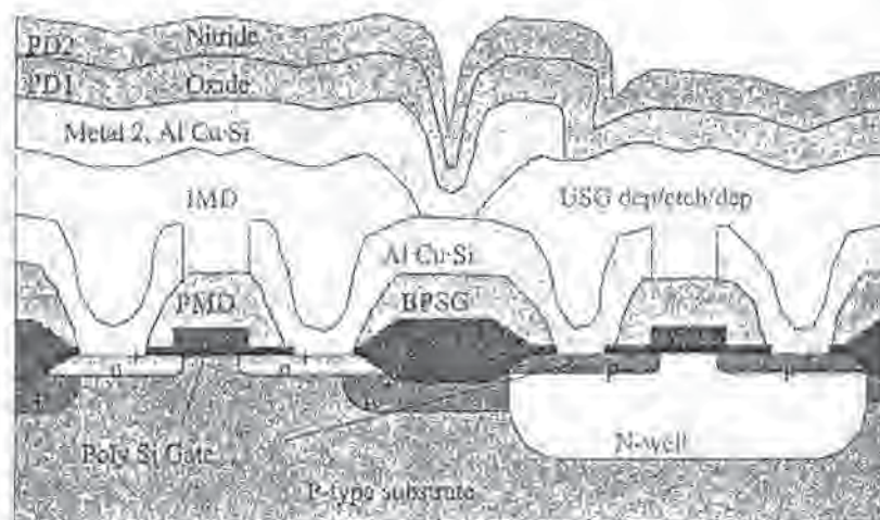
Fig. 12-8 Schematic of a double-level-metal structure in CMOS with partial-planarization.
