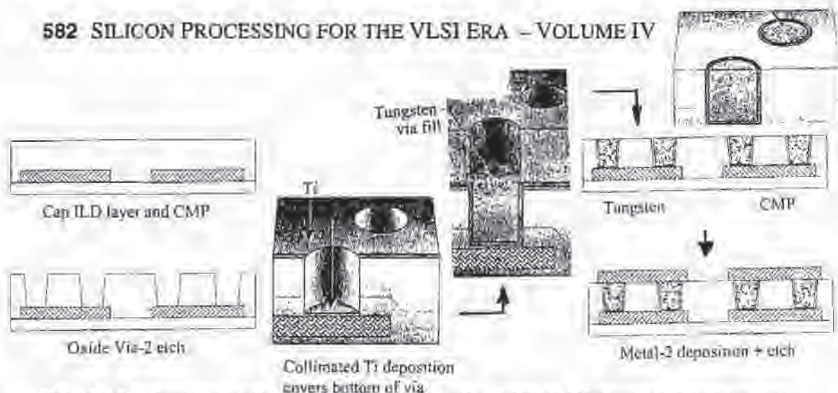
Fig. 12-12 Schematic of the process used to form the "hybrid" W-plug/Al-alloy structure.
