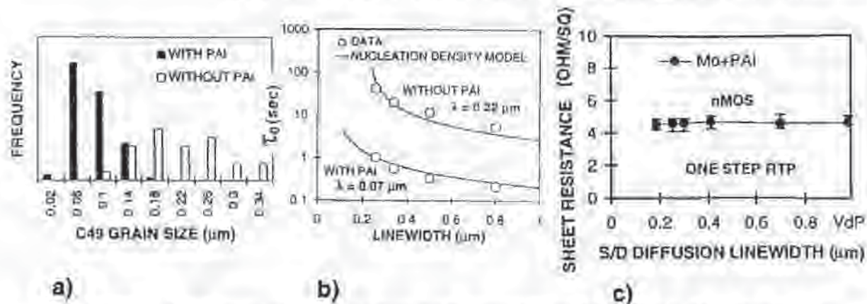
Fig. 13-10 a) C-49 grain size distribution with and without PAI. The C-49-grain size is significantly reduced by PAI, making it possible to achieve low sheet-resistance on 0.1- \mu\text{m} gates. b) Results and predictions of the nucleation-density-model for n^+ gates with and without PAL. The difference in C-49 grain size ( \lambda ) accounts for the large increase in transformation times. Transformation times \tau_0 increase dramatically as the linewidth approaches \lambda , making the process without PAI incompatible with linewidths below 0.2- \mu\text{m} . c) Mo + PAI allows low-sheet resistance (4- \Omega -sq) to be obtained for 0.2- \mu\text{m} -wide lines.
