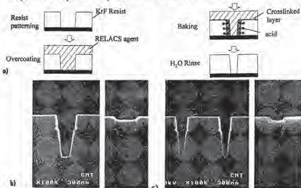
Fig. 9-32 a) Process flow of RELACS. (b & c) Top corner rounding provided during etch in a TCP system. An in-situ hard mask/rounding/trench etch scheme was used. The top corner is rounded to \sim 15 \text{ nm} radius. b) 180-nm-wide trenches as etched and after fill and CMP; c) 100-nm-wide trenches as etched and after fill and CMP. 54
