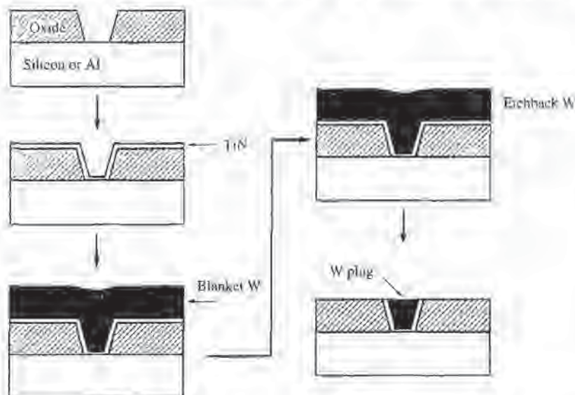
Fig. 12-11 Schematic of the process used to form W-plugs with CVD-W and etchback.
