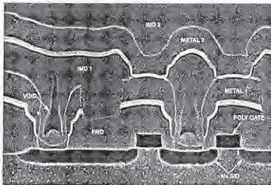
Fig. 12-9 SEM of an actual double-level-metal structure in CMOS with partial planarization.
