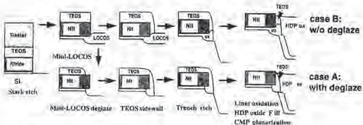
Fig. 9-17 Process sequence of STI using mini-LOCOS edge. 29 (© IERE 1997)
