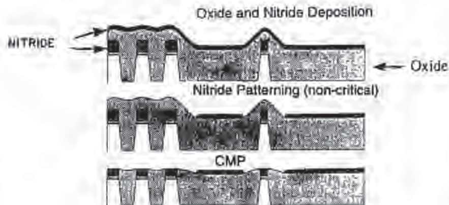
Fig. 9-28 Patterned second-nitride layer approach to minimize dishing during CMP of trench-fill oxide.
