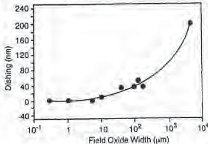
Fig. 9-24 Dishing versus field-oxide-region width for a specific oxide CMP process 36 (©1993 IEEE).
