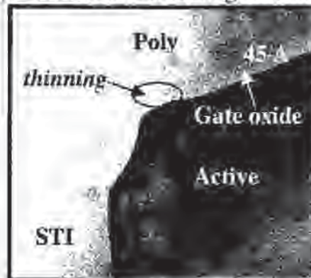
Fig. 9-15 TEM showing thinning of the gate oxide near the edge of an active region in an STI structure due to the Kooi effect. 23
