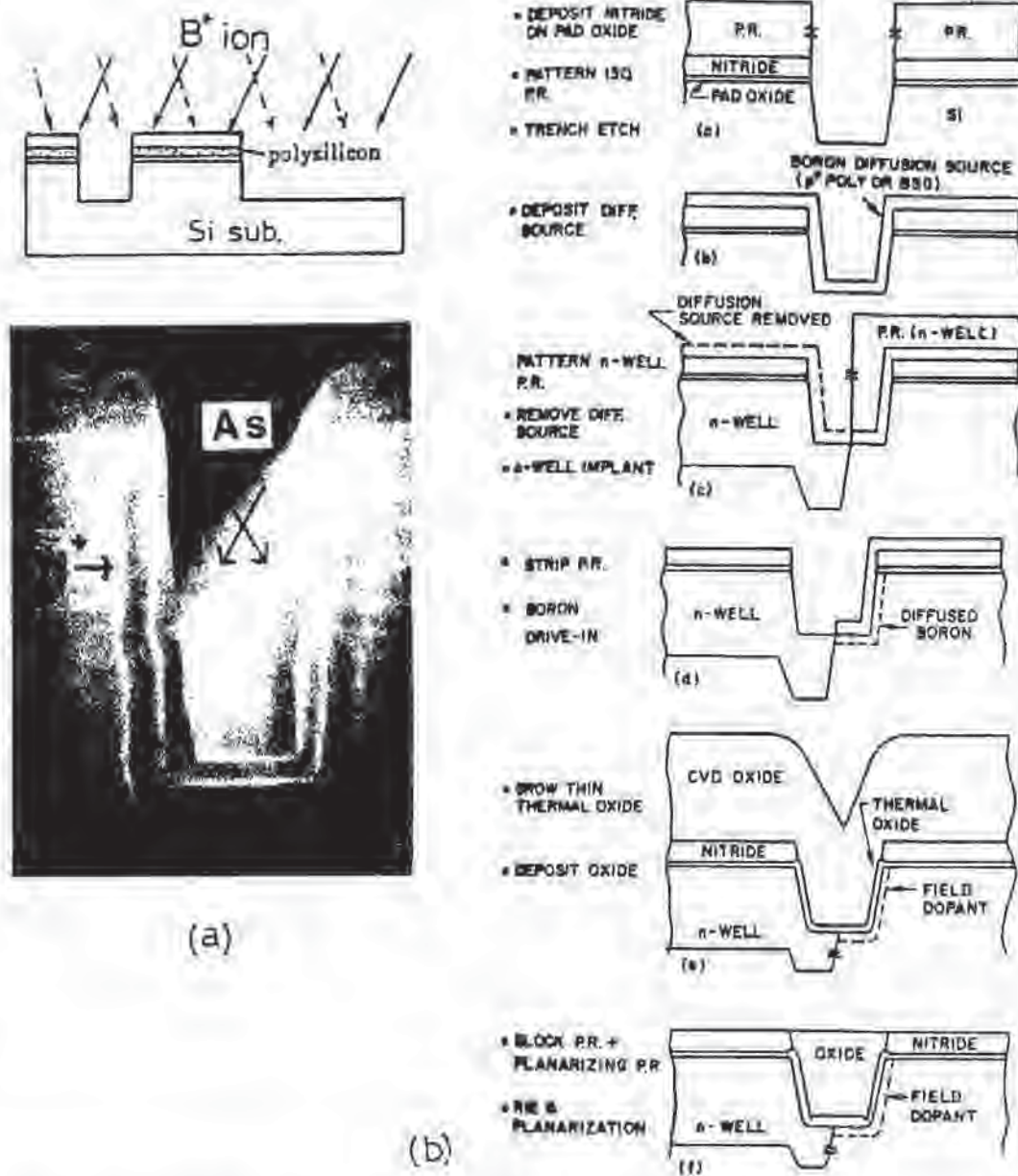
Fig. 9-9 a) Schematic of oblique ion implantation and SEM cross section result of this procedure. 16 (© 1987 IEEE) b) Shallow trench isolation process flow using a doped oxide as diffusion source of trench sidewall doping. 17 (© 1988 IEEE)
