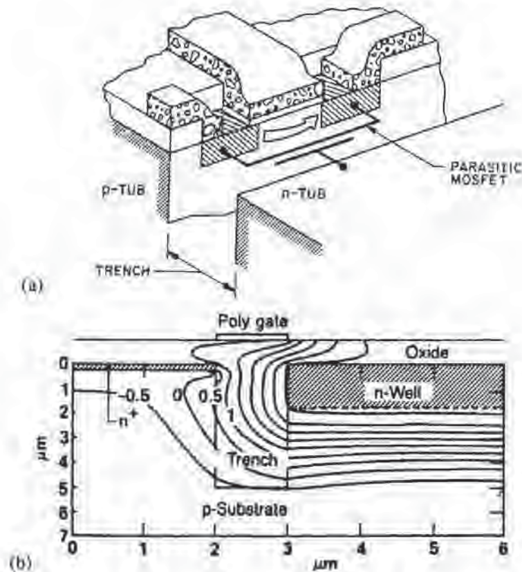
Fig. 9-6 a) A parasitic-sidewall-MOSFET with the n -well as the gate and the trench serving as the gate oxide. 12 From S.M. Sze Ed., High-Speed Semiconductor Devices , Copyright 1990 by John Wiley & Sons. Reprinted with permission. b) Cross-sectional view of a simulation of the 2-D equipotential contours in an n -well CMOS with trench isolation. The simulation is done at Q_{fc} = 5 \times 10^{10} \text{ cm}^{-2} , N_A = 9 \times 10^{14} \text{ cm}^{-3} , V_{\text{well}} = 3 \text{ V} , V_{GS} = 0 \text{ V} , V_{\text{sub}} = -1 \text{ V} . 13 (© 1983 IEEE)
