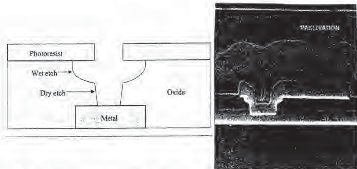
Fig. 12-7 a) Schematic of a via with a "champagne-glass" shape; b) SEM of actual via.
