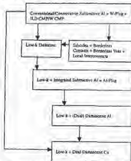
Fig. 12-26 Schematic illustrating an interconnect migration. 15
