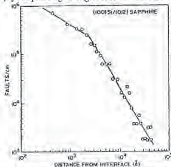
Fig. 11-17 Stacking-fault-density as a function of the distance from the silicon/sapphire interface in an MOS structure. 21 Reprinted by permission of the American Physical Soc.
