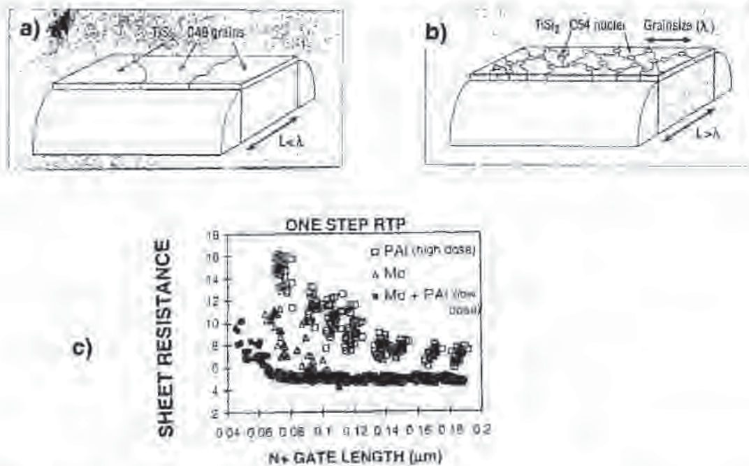
Fig. 13-9 The \text{TiSi}_2 C-49 (high resistivity) to C-54 (low resistivity) transformation-rate depends on the density of nucleation sites: a) Without a pre-amorphization implant (PAI) there are few nucleation sites on narrow polysilicon-lines; b) PAI reduces the C-49 grain size, increasing the number of triple-grain-boundaries and C-54 sites; c) By using PAI + MO the sheet-resistance of \text{TiSi}_2 lines remains low for narrower lines than when only PAI is used.
