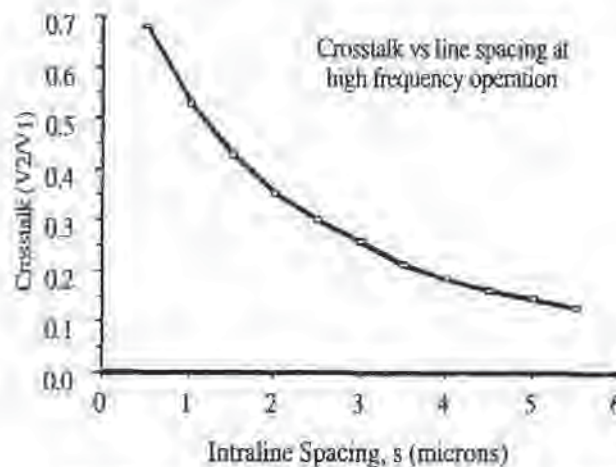
Fig. 12-25 Simulation results showing that the magnitude of the crosstalk between 2 interconnects separated by different line spacings, s . 10 Conditions described in Fig. 12-24.
