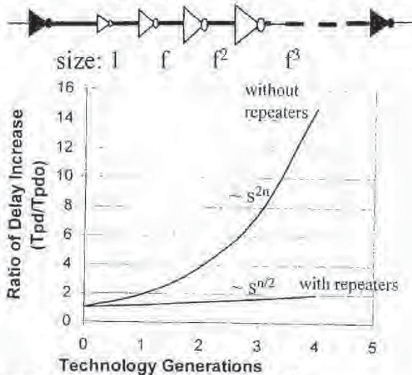
Fig. 12-22 Impact of repeaters on global propagation delay. 5
