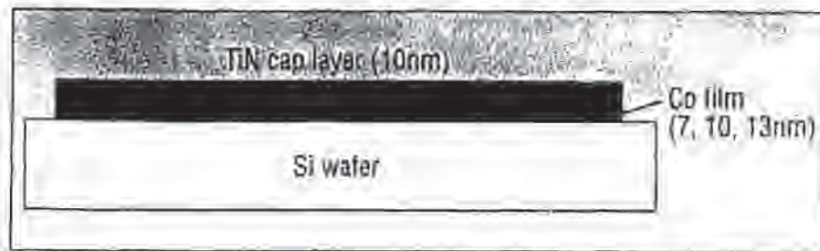
Fig. 13-12 Schematic cross-section of a \text{CoSi}_2 film with a TiN capping layer on a Si wafer.
