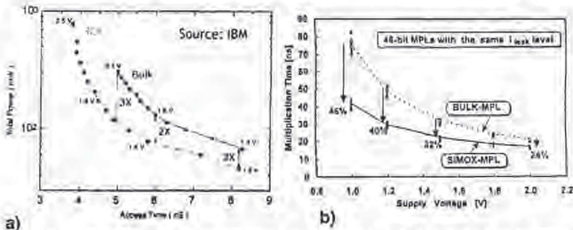
Fig. 11-6 a) Power drain and access time for bulk and SOI CMOS for drive voltages ranging from 1.2 V; b) Comparison of 48-bit-multiplier performance between bulk and SOI using a 0.25- \mu\text{m} CMOS technology.
