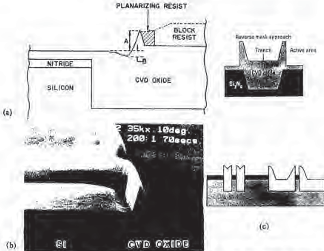
Fig. 9-25 Spikes in the dielectric layer after the RIE step of the RIE/CMP process: a) Simulated cross-section after RIE; b) SEM cross-section after RIE and resist strip, showing dielectric spikes; c) Schematics of the dielectric spikes after RIE and resist strip.
