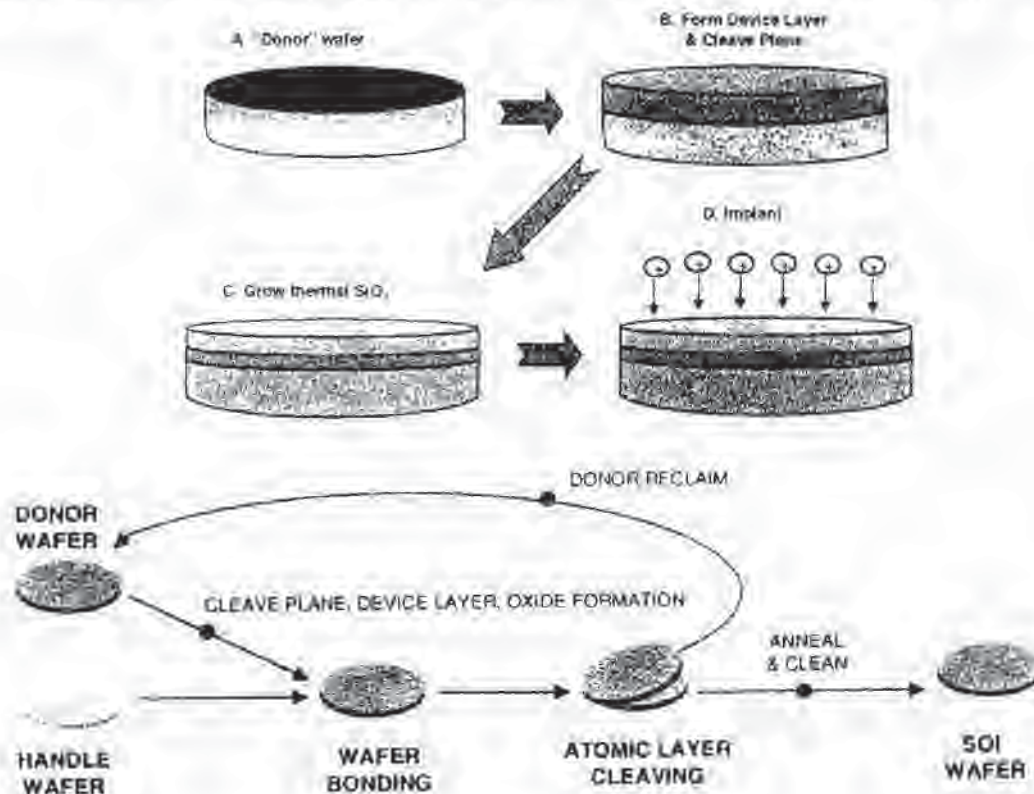
Fig. 11-25 Process flow of the Nanocleave® SOI technology.
