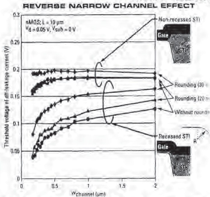
Fig. 9-31 Corner rounding helps eliminate the reverse narrow channel effect that causes subthreshold leakage. Recess of the isolation region below the silicon surface exacerbates the problem. 26 Reprinted with permission of Semiconductor International.
