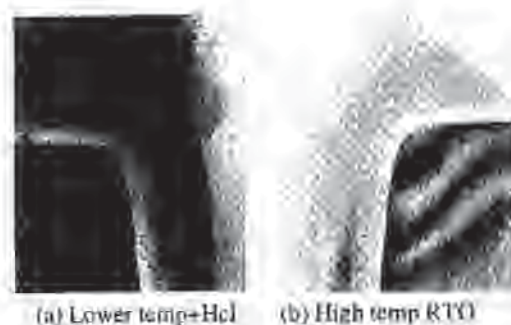
Fig. 9-13 Cross-sectional TEM of the top trench corner after pad oxide undercut & liner oxidation: HCl in the ambient (a); and higher-temp RTP-oxidation (b) improve corner rounding.
