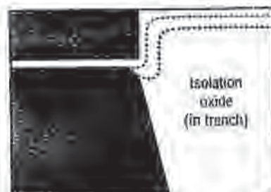
Fig. 9-16 Topography of the top corner of the Si active region and the oxide surface in the trench. The dotted lines represent the removal of oxide that occurs during the wet HF dips before the sacrificial oxide and gate oxide growth steps.
