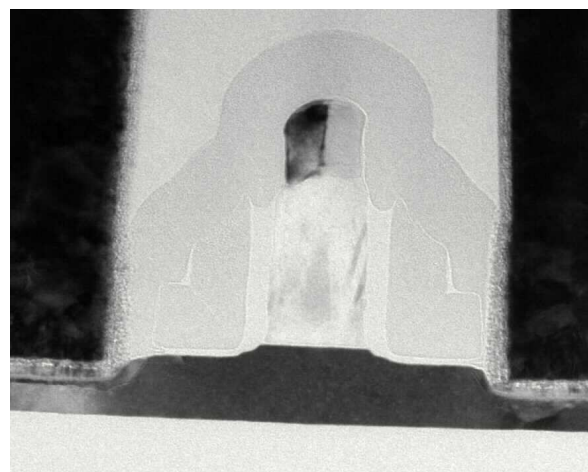
Figure 9. PMOS Transistor in IBM PPC970FX
