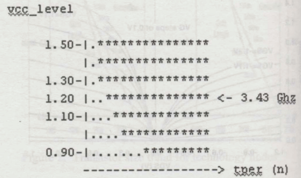
Figure 14: Shmoo plot for SRAM Fmax and Vcc
