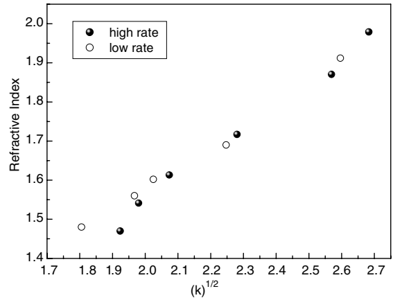
Fig. 5. Refractive Index ( n ) as function of the square root of the dielectric constant ( k ) 1/2 .
