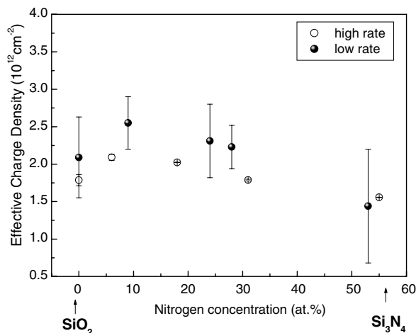
Fig. 2. Effective charge density ( N_{eff} ) as function of dielectric nitrogen concentration.
