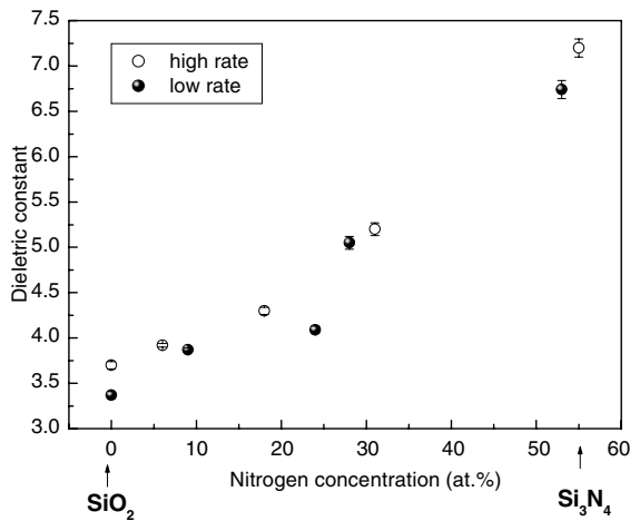
Fig. 4. Dielectric constant ( k ) as function of the dielectric nitrogen concentration.
