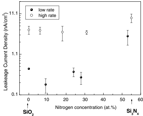
Fig. 3. Leakage current density ( I_q ) as function of dielectric nitrogen concentration.
