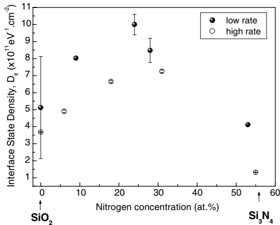
Fig. 1. Interface state density ( D_{it} ) as function of dielectric nitrogen concentration.
