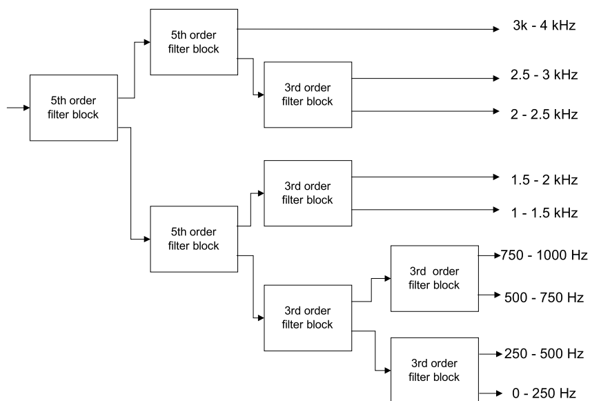
Figure 3.2: Filter bank
