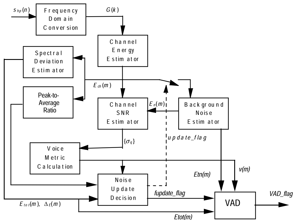
Figure 4.1: Block Diagram of the VAD algorithm: Option 2
