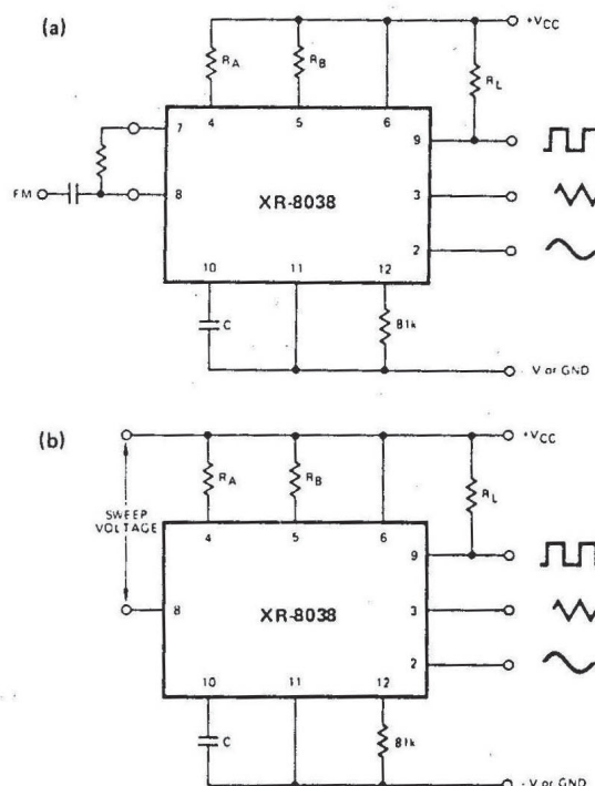
Figure 4. Connections for Frequency Modulation (a) and Sweep (b).
