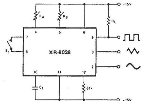
Figure 1. Generalized Test Circuit
