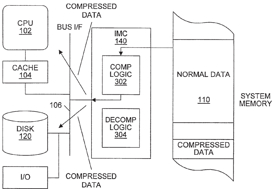
Compression from memory to CPU or Disk
