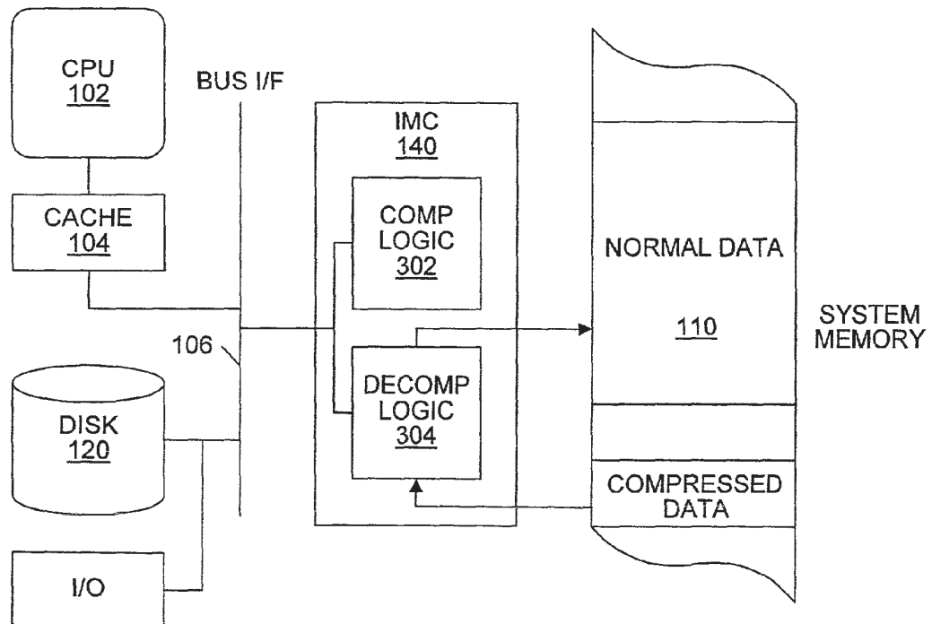
Memory to memory decompression
