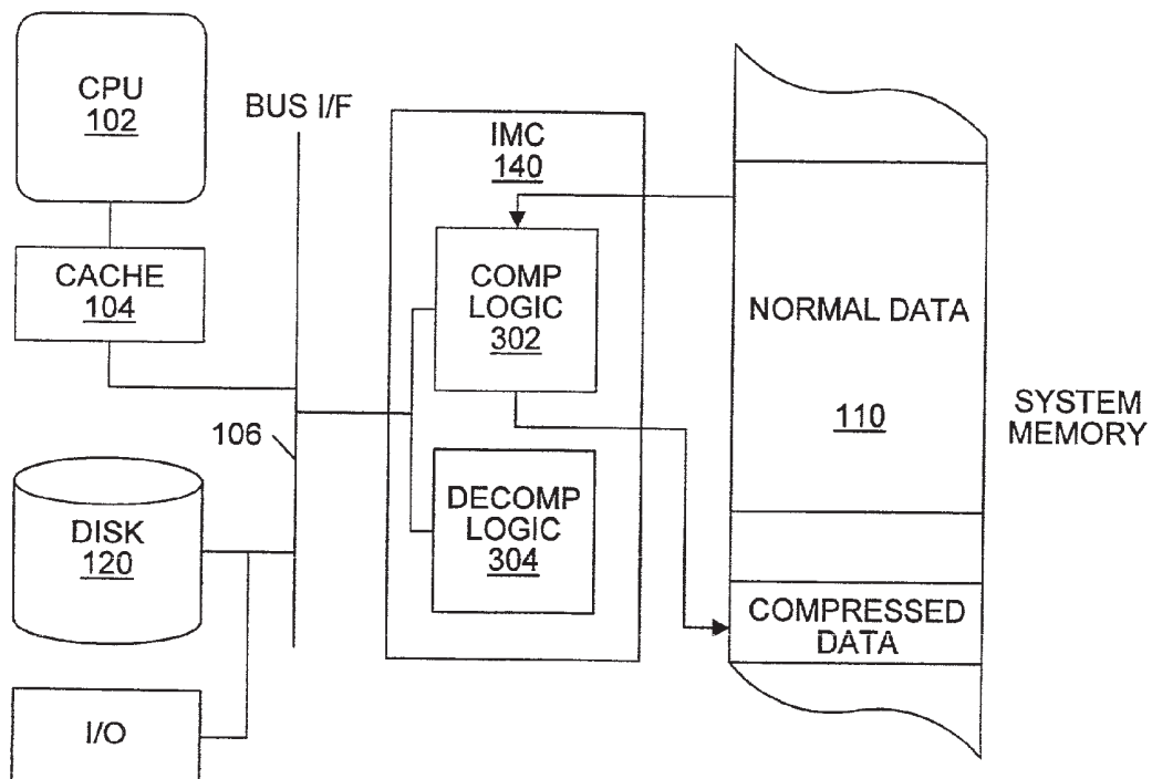
Memory to memory Compression
