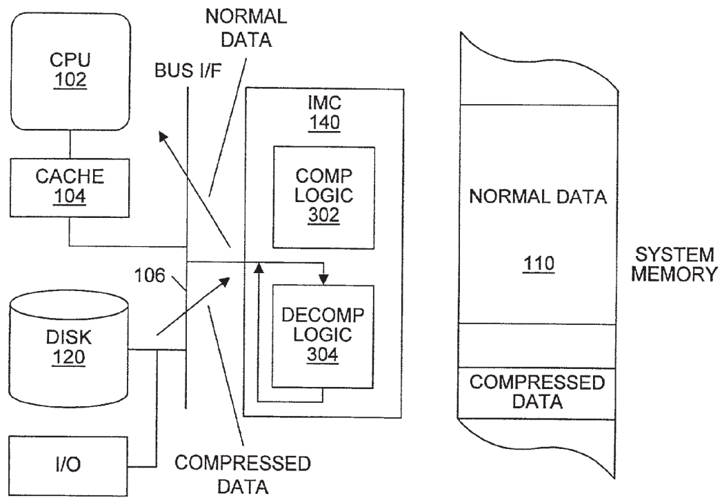
Decompression of disk to CPU
