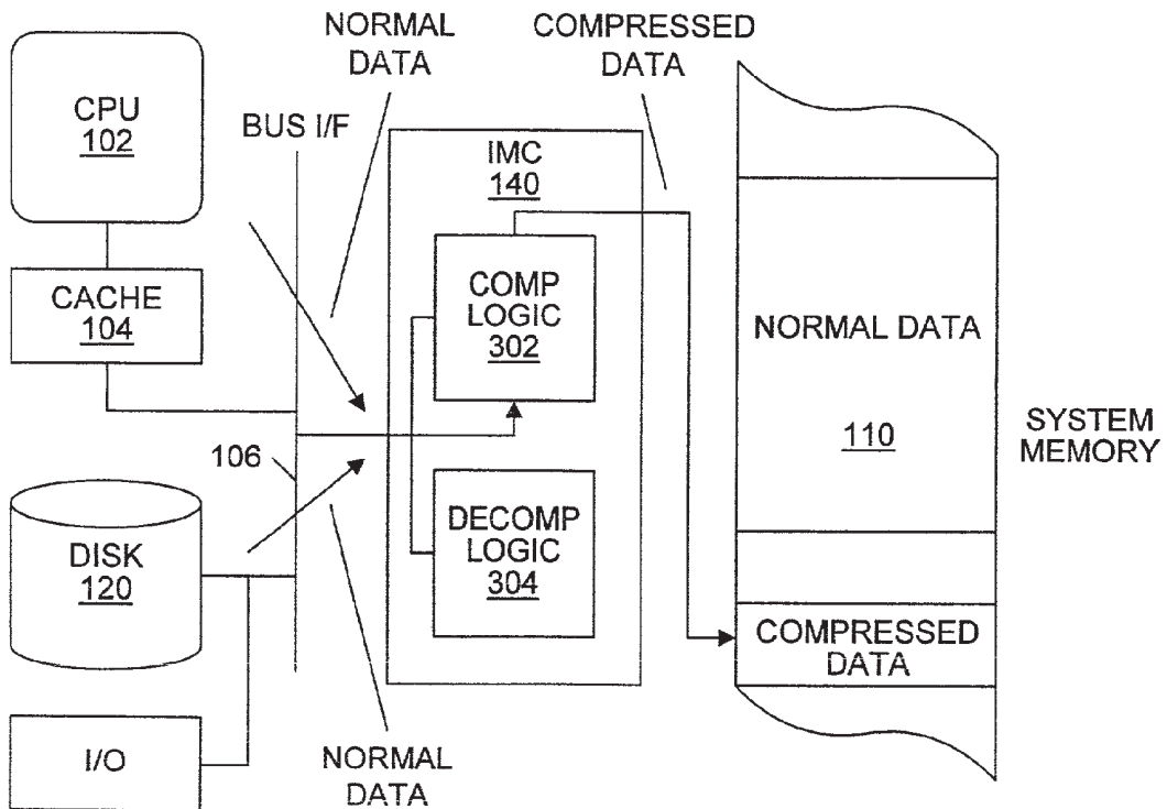
Compression from CPU or disk to memory
