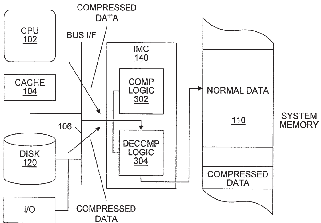
Decompression from Disk or CPU to memory
