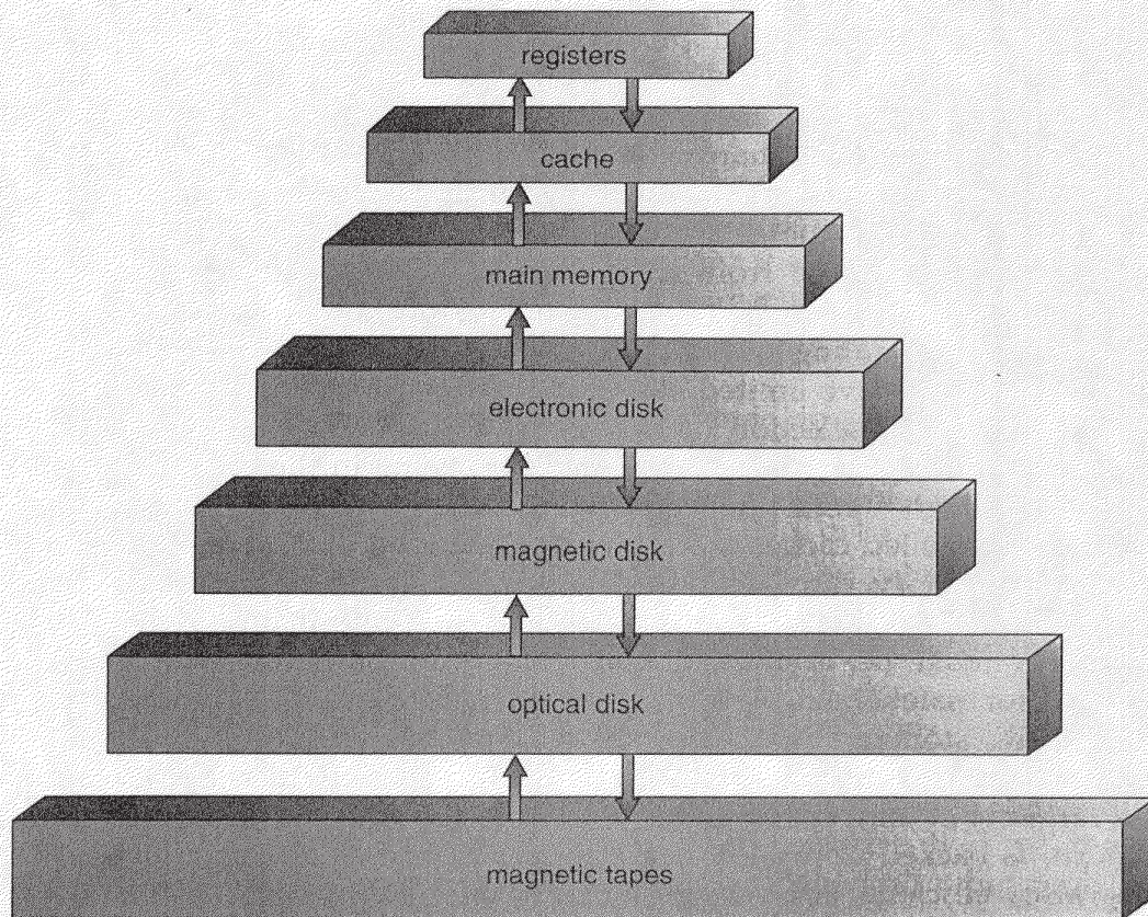
Figure 2.6 Storage-device hierarchy.
