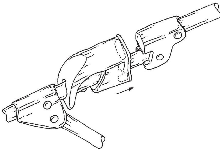
FIG. 2C PRIOR ART
