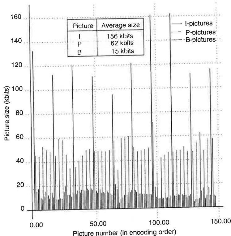
Figure 6.4 Example of bit distribution among I-, P-, and B-pictures in an MPEG-1 coded bit stream. Pictures are coded in IPBBPBBPBBPBBPBB sequence.
