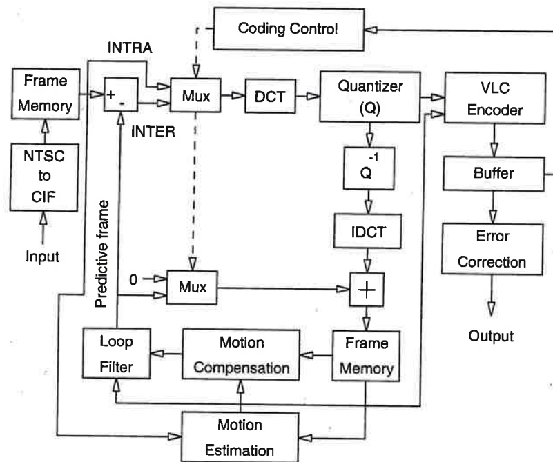
Figure 7.2 Block diagram of an H.261 video encoder.
