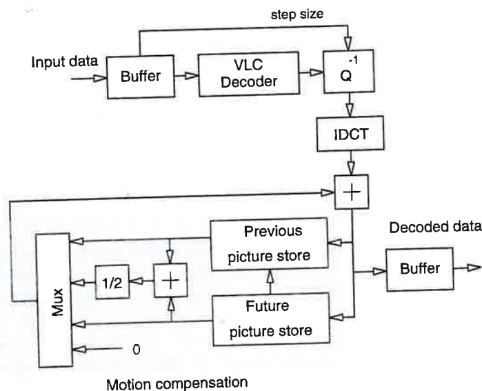
Figure 6.8 Block diagram of an MPEG decoder.
