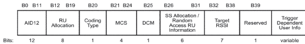
(c) User Info field of Trigger frame
