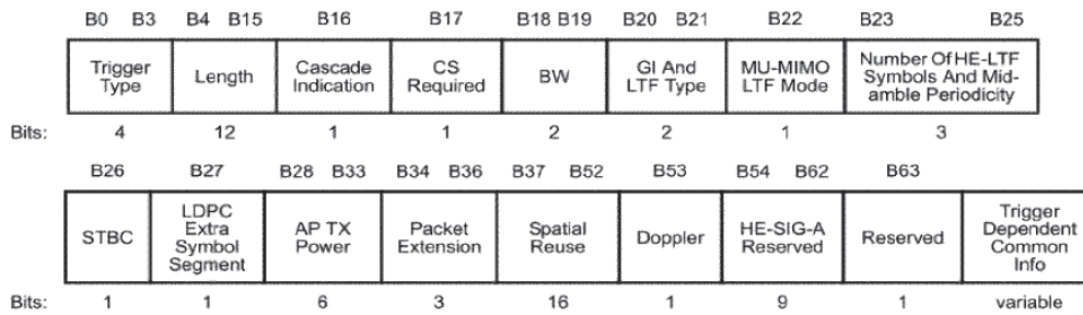
(b) Common Info field of Trigger frame
