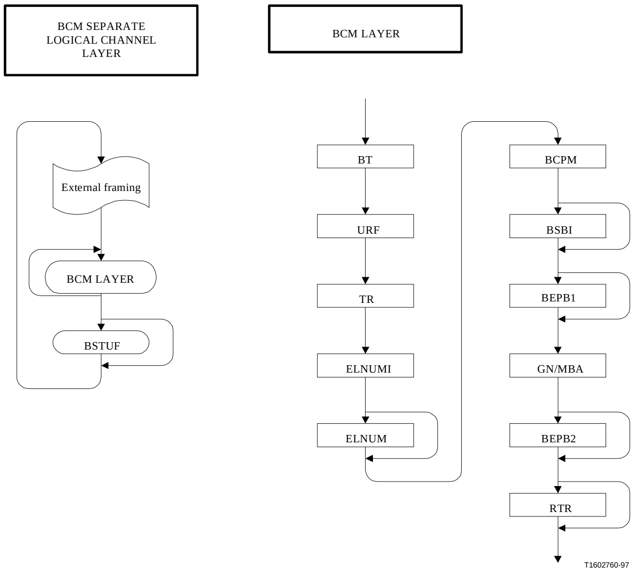
Figure 6/H.263 (part 5 of 7) – Syntax diagram for the video bitstream
