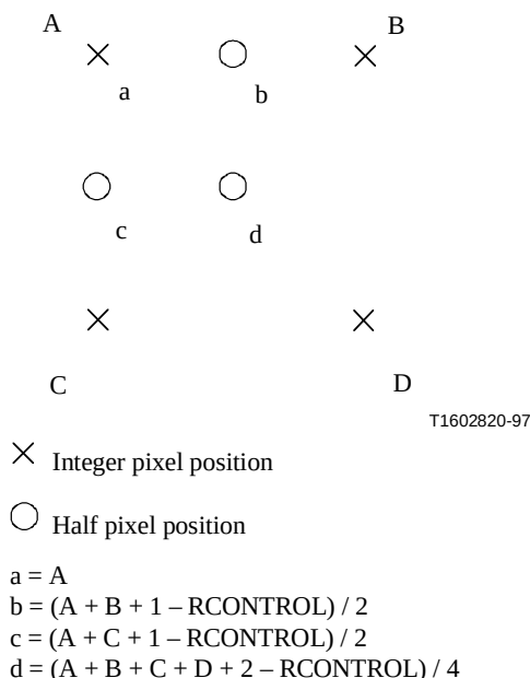
Figure 13/H.263 – Half-pixel prediction by bilinear interpolation
