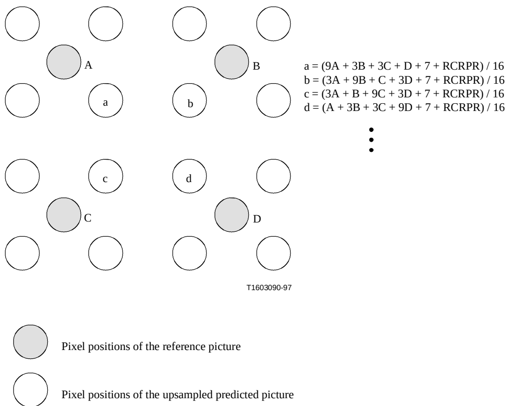
Figure P.4/H.263 – Factor-of-4 upsampling for pixels inside the picture
