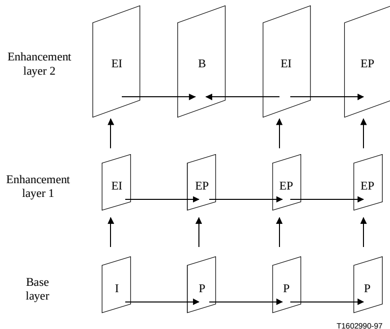
Figure O.4/H.263 – Illustration of multilayer scalability
