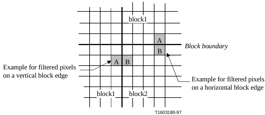
Figure Q.10/H.263 – Default block boundary filter
