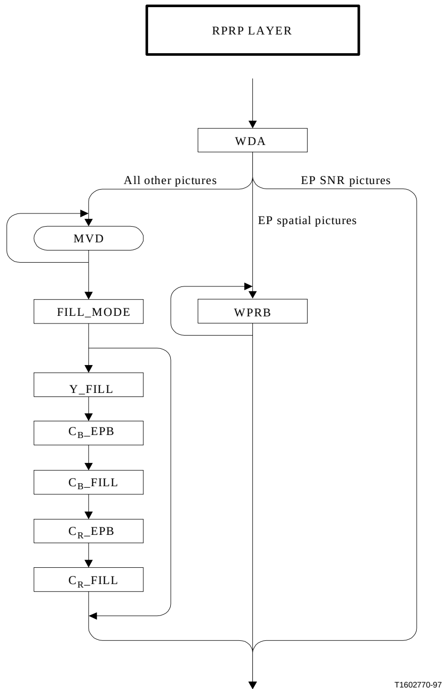
Figure 6/H.263 (part 6 of 7) – Syntax diagram for the video bitstream
