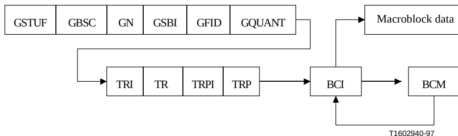
Figure N.2/H.263 – Structure of GOB layer for NEWPRED
