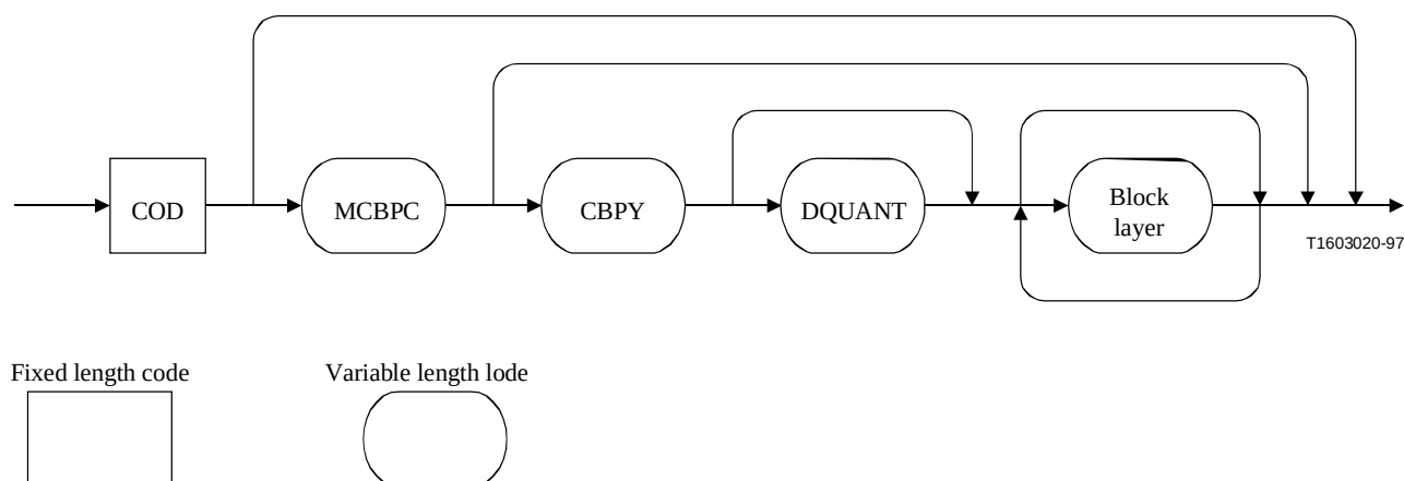
Figure O.7/H.263 – Macroblock syntax for EI-pictures
