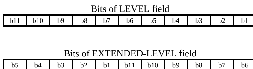
Figure T.1/H.263 – Cyclic rotation of coefficient representation
