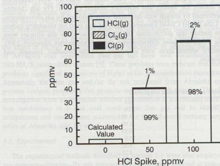
Fig. 6. Chlorine speciation results for the 50- and 100-ppmv HCl(g) injections during Absaloka coal combustion tests.
