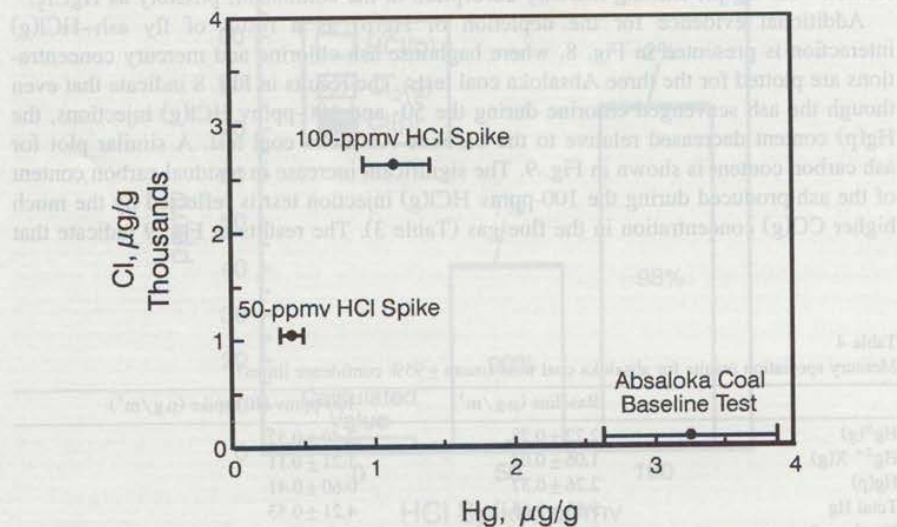
Fig. 8. Chlorine versus mercury concentrations for the Absaloka coal fly ash. Error bars represent 95% confidence limits based on three mercury measurements.
