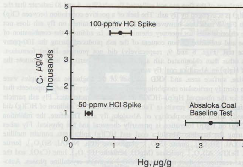
Fig. 9. Carbon versus mercury concentrations for the Absaloka coal fly ash. Error bars represent 95% confidence limits based on three mercury measurements.
