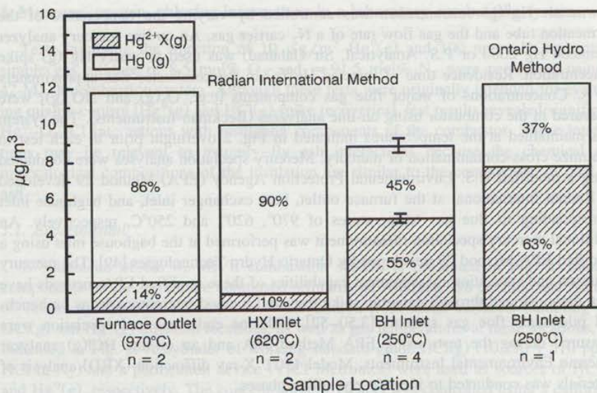
Fig. 3. Mercury speciation results for the 10- \mu\text{g}/\text{m}^3 \text{Hg}^0(\text{g}) baseline spike test. The relative proportions of different mercury species are indicated within each bar as a percent of the total mercury. Error bar represents 95% confidence limits based on four modified (Radian International) EPA Method 29 measurements. Abbreviations: n = number of speciation measurements performed, BH = baghouse, and HX = heat exchanger.
