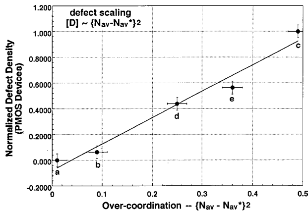
FIG. 6. Plot of normalized defect density as a function of \{N_{av} - N_{av}^*\}^2 , where N_{av}^* is the value for an ideal Si-SiO 2 interface. Data points a, b, and c are from Fig. 1, and d and e from Fig. 2, and the solid line is a linear regression analysis of the data points.
