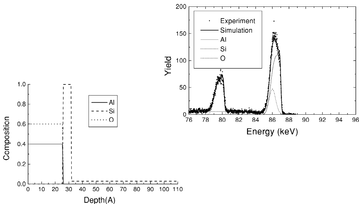
Fig. 9. MEIS spectra of an air exposed \text{Al}_2\text{O}_3 over H-terminated Si.
