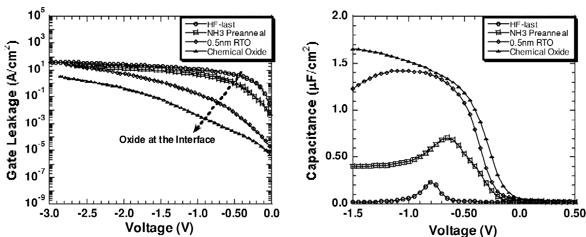
Fig. 13. CV and IV of poly/ZrO 2 /Al 2 O 3 with various interface preparations on p-Si.
