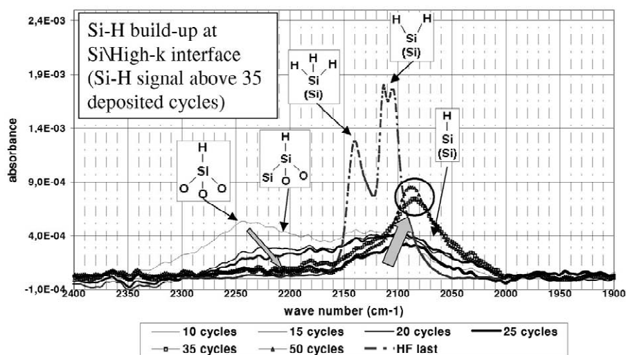
Fig. 8. Si-H stretch region of FTIR on air exposed \text{Al}_2\text{O}_3 /H-terminated interface.
