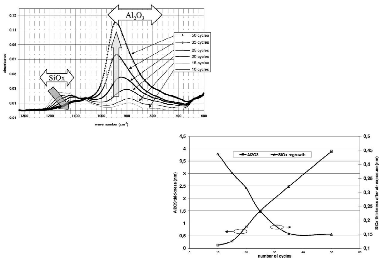
Fig. 7. Oxide modes of FTIR on air exposed \text{Al}_2\text{O}_3 /H-terminated interface.
