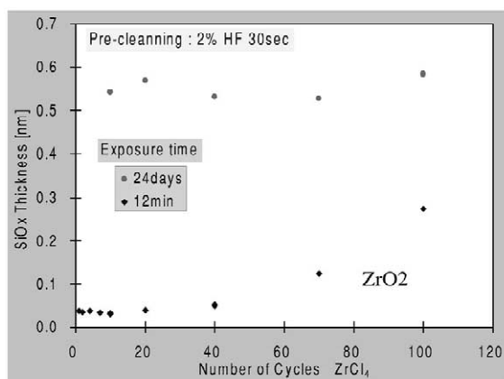
Fig. 6. Interfacial oxide growth of as-deposited and air exposed ZrO 2 over H-terminated Si.
