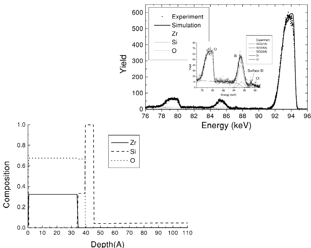
Fig. 10. MEIS spectra of an air exposed \text{ZrO}_2 over H-terminated Si.
