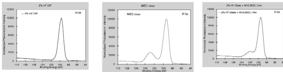
Fig. 1. Si 2p XPS spectra of various interfaces and possible bonding configurations.
