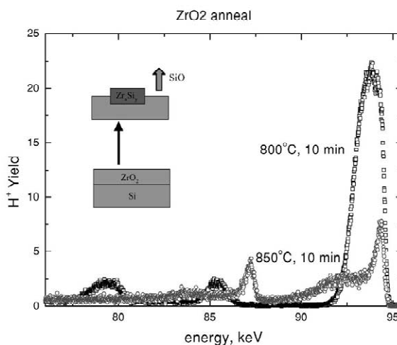
Fig. 14. MEIS spectra of a thermally annealed \text{ZrO}_2 over H-terminated Si.
