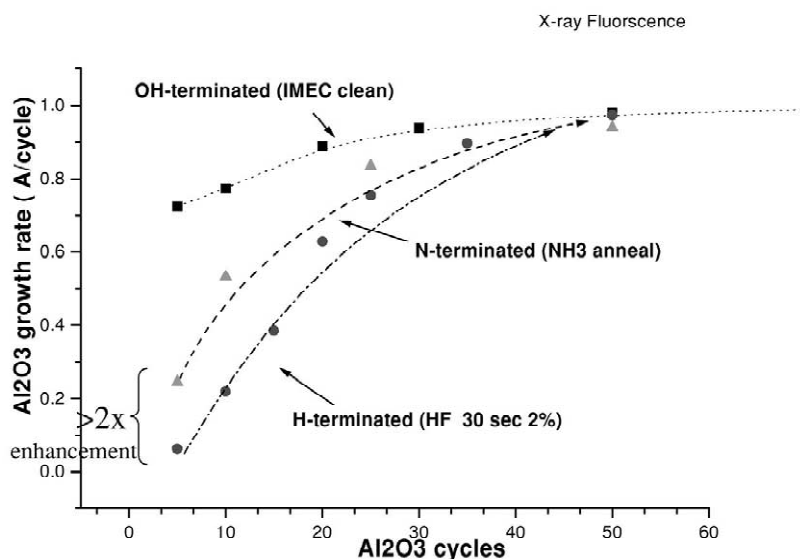
Fig. 2. Effect of interface preparation on ALCVD Al 2 O 3 growth kinetics.
