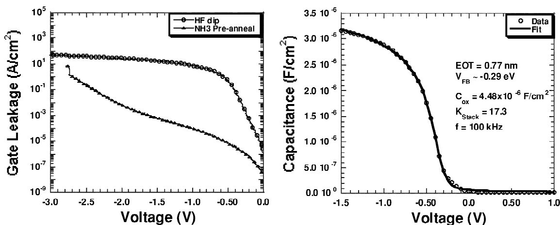
Fig. 12. CV and IV of TiN/ZrO 2 /Al 2 O 3 on H-terminated and N-terminated Si.
