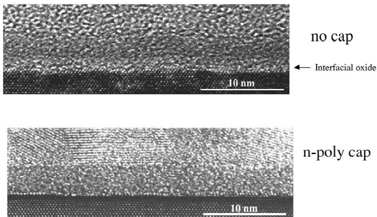
Fig. 11. TEM of a 100-nm polysilicon capped 3-nm Al 2 O 3 /H-terminated Si and a un-capped 3-nm Al 2 O 3 /H-terminated Si.
