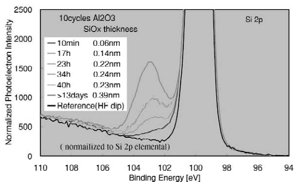
Fig. 3. Effect of air exposure on interfacial oxide growth on ten cycle Al 2 O 3 on H-terminated Si.
