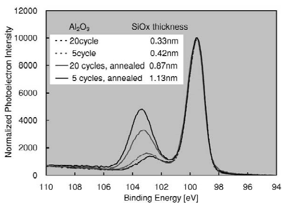
Fig. 4. Effect of thermal anneal in oxygen on five and 20 cycles of Al 2 O 3 on H-terminated Si.
