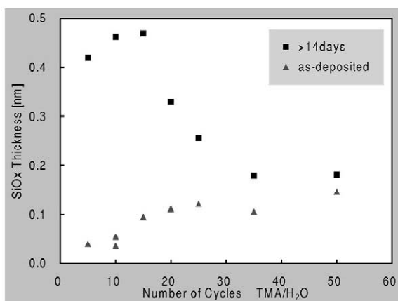
Fig. 5. Interfacial oxide growth of as-deposited and air exposed Al 2 O 3 over H-terminated Si.
