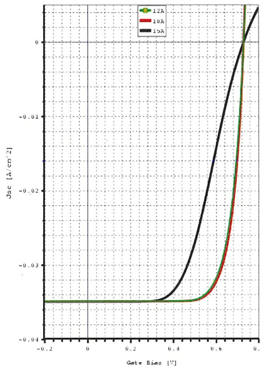
Figure 11: Sentaurus® model of PE structure for tunnel dielectric thicknesses of 10, 12 and 15 Å, showing fill factor degradation with thicker layers.
