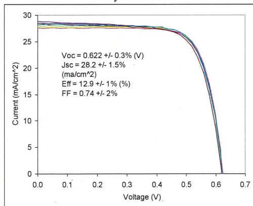
Figure 8: IV curves for seven 2x2 cm isolated PE cells in a 12.5x12.5 cm² area with 400 nm p-type poly on n-Si.
