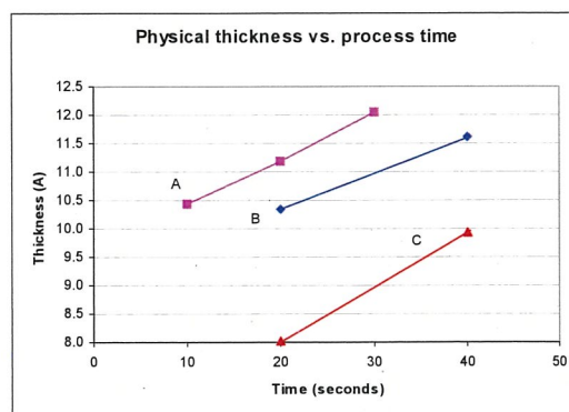
Figure 5: Physical thickness as measured with XPS as a function of growth time for three different tunnel dielectric processes, A, B and C.
