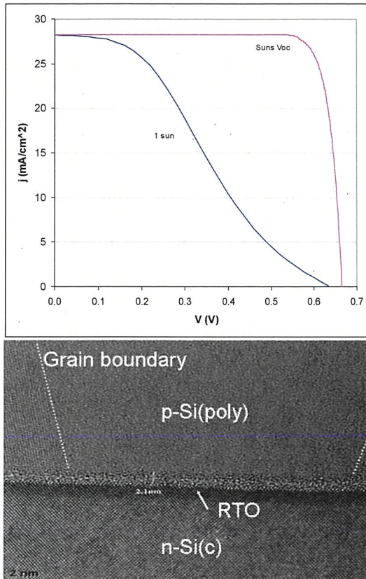
Figure 10: Suns-Voc and measured IV for a cell with a thick tunnel oxide as shown in the TEM of the interface, with poly on top and crystal silicon underneath
