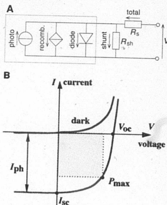
Fig. 2. (A) Electrical equivalent circuit of a PV solar cell (67). The diode is a dark (nonilluminated) p-n or p-i-n diode. Additional recombination (particularly in the i-type layer of p-i-n diodes) is represented by the current source, which counteracts the photogenerated current. R_s and R_{sh} are resistors that represent electrical losses (for example, R_s losses due to contact resistance and R_{sh} losses due to pinholes through the solar cell). (B) Typical I - V characteristics of a solar cell, with the three characteristic parameters: short-circuit current I_{sc} , open-circuit voltage V_{oc} , and fill factor FF = P_{max}/(V_{oc} \times I_{sc}) ; P_{max} is the electrical power delivered by the cell at the maximum power point MPP.
