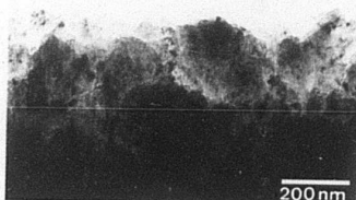
Fig. 4. TEM cross-section micrograph of typical intrinsic microcrystalline silicon layer as deposited by PECVD and used for p-i-n solar cells (26).
