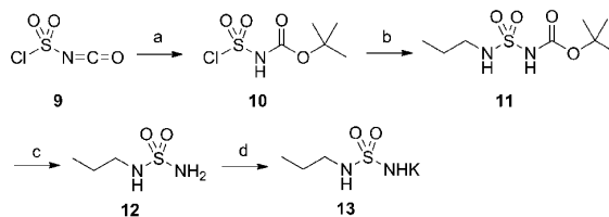
Scheme 2. Synthesis of Sulfamide Potassium Salt Building Blocks a
