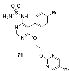
Figure 6. Structure of sulfamide 71, a major metabolite of compound 17 in Wistar rats and Beagle dogs.
