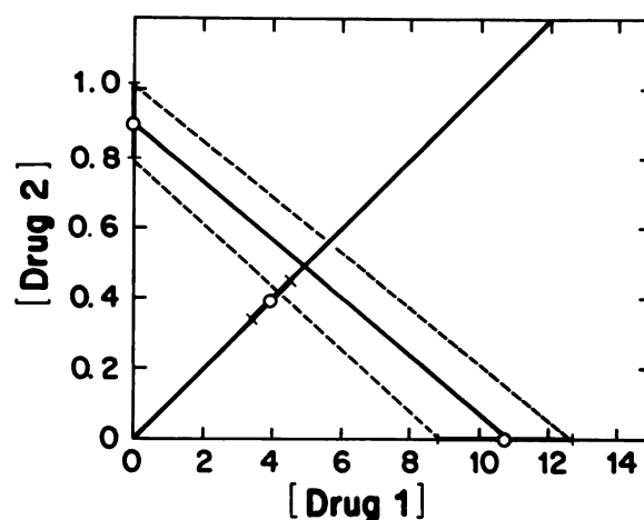
FIG. 28. Further isoblographic analysis of data from figure 27, panels (A), (B), using an interpretation of the approach of Gessner (1974).
