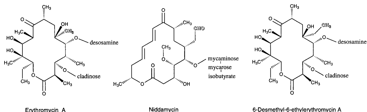
FIG. 1. Structures of Er, Nd, and 6-ethylErA. Shadowed letters represent relevant side groups.
