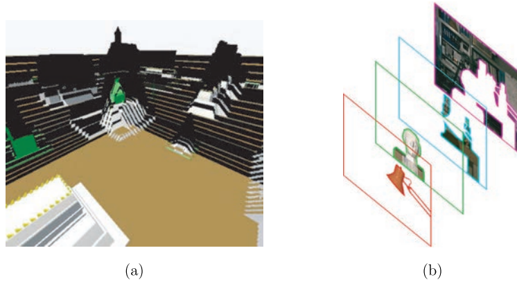
Fig. 7.3 Planar layers to approximate scene geometry. (a) Planar impostors [45] (courtesy of Stefan Jeschke), (b) pop-up light field [96].
