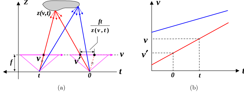
Fig. 4.5 An illustration of 2D light field or EPI. (a) a point is observed by two cameras 0 and t . (b) two lines are formed by stacking pixels captured along the camera path. Each line has a uniform color because of Lambertian assumption on object surfaces.
