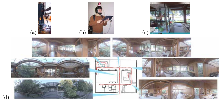
Fig. 4.14 Panoramic video [106]. (a), (b) Two versions of the capture system with Point Grey's Ladybug TM 6-camera system, (c) screen shot of user interface for navigation, and (d) sample panoramas along camera path network.
