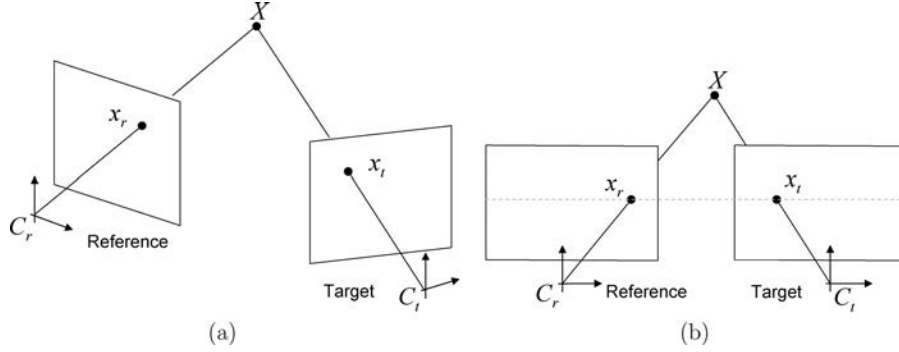
Fig. 6.1 Relationship between 2D points x_r and x_t in the reference and target images, respectively, and 3D point X . On the left shows an arbitrary virtual view while the right shows a lateral motion (with rectified geometry).
