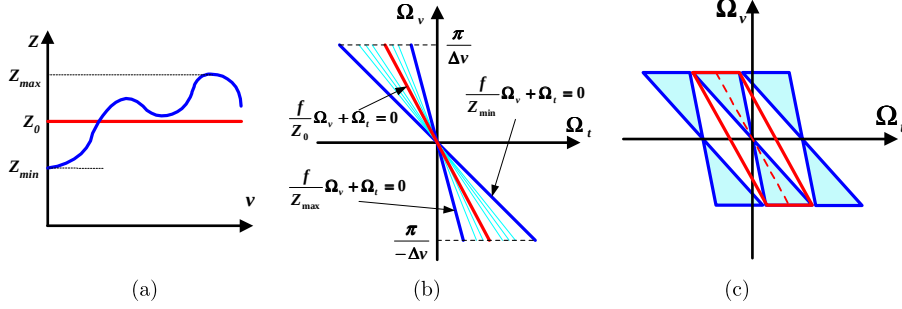
Fig. 4.6 Spectral support for light field signal with spatially varying depths: (a) a local constant depth model bounded by z_{\min} and z_{\max} is augmented with another depth value z_0 ; (b) spectral support is now bounded by two smaller regions, with the introduction of the new line of z_0 ; and (c) optimal depth at z_0 .
