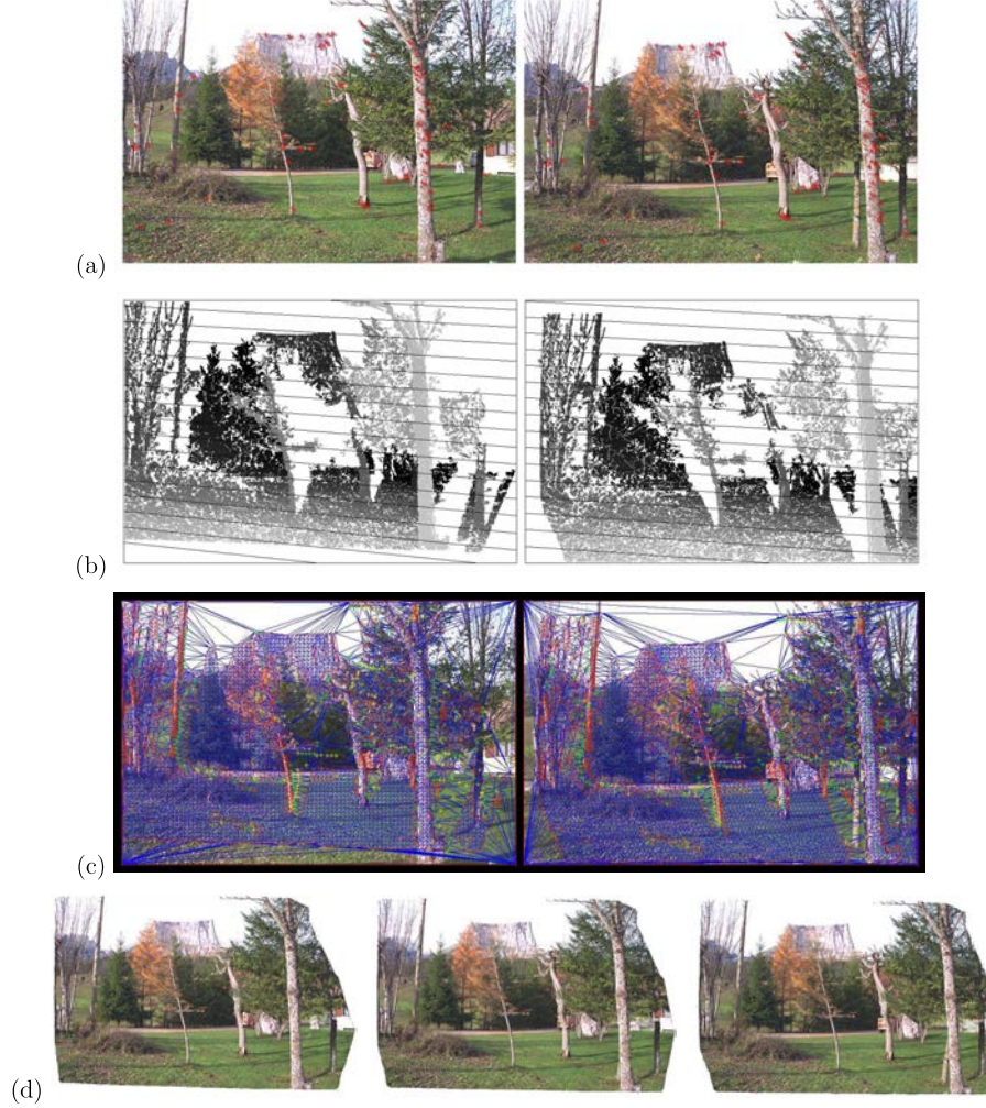
Fig. 5.4 Joint view triangulation. (a) Source views with extracted point matches. (b) Computed disparity at points with correspondence. The darker the pixel, the smaller the disparity. White pixels represent those without any correspondence. Epipolar lines (shown as dark lines) are superimposed. (c) Resulting meshes with constraint edges (in red). (d) Interpolated views. Images courtesy of Maxime Lhuillier.
