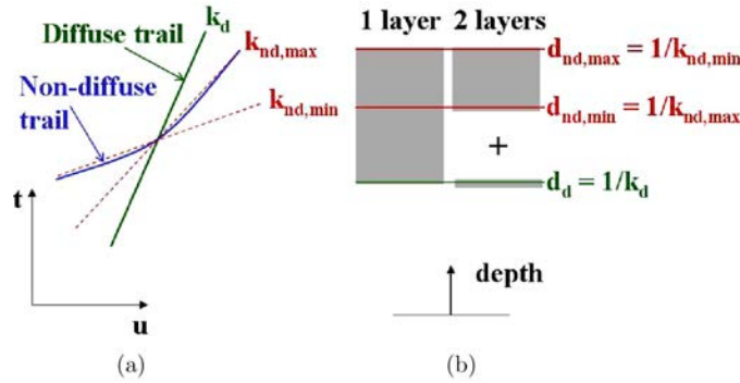
Fig. 9.3 Benefit of using separate layers. (a) Closeup view of vicinity of non-diffuse trail, (b) Depth variation (shaded regions) required to represent both diffuse and non-diffuse component using 1 and 2 layers. The dotted lines in (a) are the bounding slopes for the non-diffuse trail at the point of intersection between the diffuse and non-diffuse trails.
