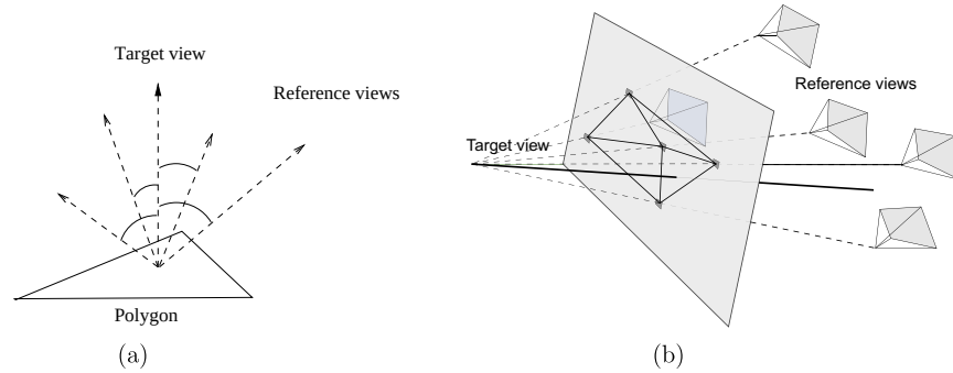
Fig. 8.2 Input view selection strategies. (a) In the work of [24], the weights associated with the input (reference) views are inversely proportional to the angle deviation. (b) In the work of [40], all the input camera centers are first projected to the target image, followed by 2D triangulation. Each triangle is associated with three input viewpoints corresponding to its vertices. These input viewpoints are the “nearest” three cameras for all the pixels that are contained within the triangle.
