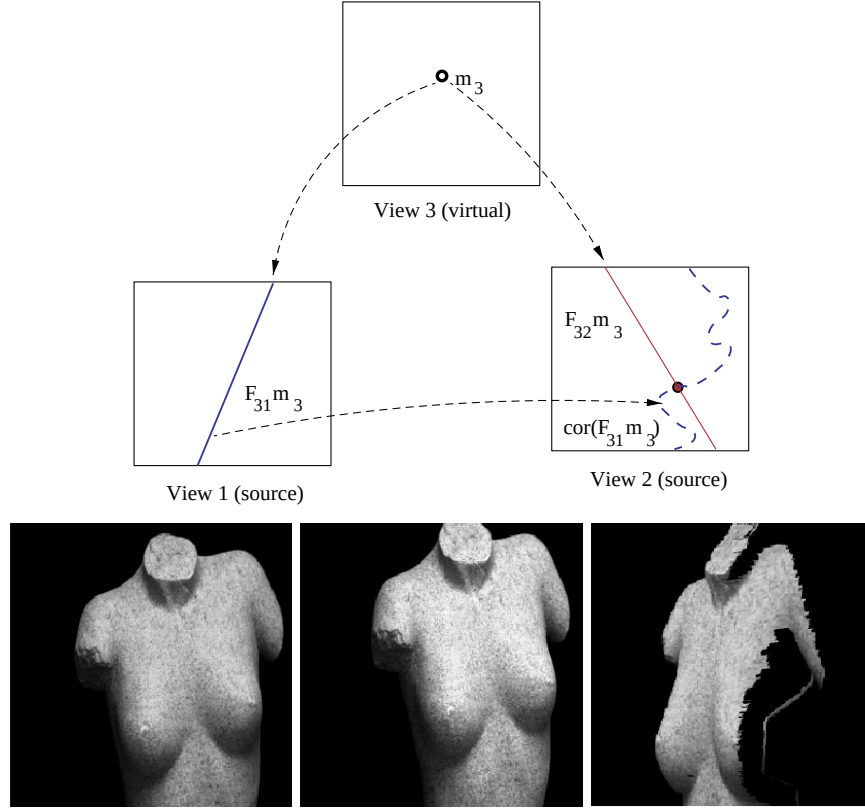
Fig. 5.5 View synthesis using the fundamental matrix [51]. Top: Process of finding the corresponding points in source views 1 and 2 that projects to point \mathbf{m}_3 in virtual view 3. Bottom, from left to right: two source images, and novel oblique view. (Images (courtesy of Stephane Laveau and Olivier Faugeras) are from S. Laveau and O.D. Faugeras, “3-D scene representation as a collection of images,” International Conference on Pattern Recognition, vol. A, pp. 689–691, October 1994. ©1994 IEEE.)
