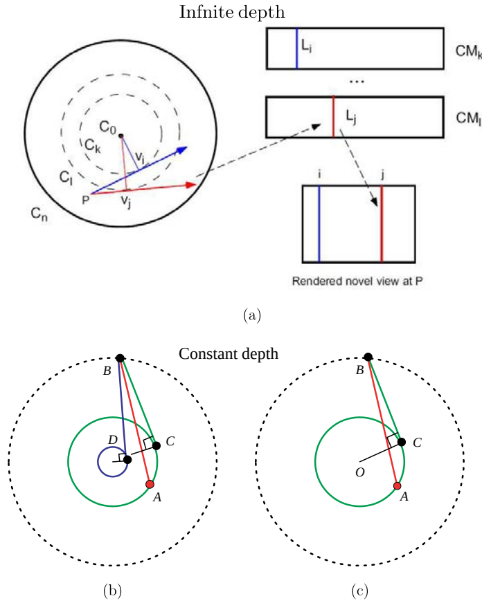
Fig. 4.10 Rendering CMs with (a) infinite depth, and (b,c) constant finite depth. (a) Rebinning: For a given ray in virtual view P (say v_j ), the CM ( CM_l ) that is tangent to it is used. The column of pixels in CM_l that corresponds to the line of tangency with v_j is used to construct part of the new view. (b) View interpolation: A ray from viewpoint A is projected to the constant depth surface (represented as a dotted circle) at B , and interpolated by two rays BC and BD that are retrieved from neighboring CMs. (c) Local warping: A ray from viewpoint A is projected to the constant depth surface at B , and reprojected to the nearest CM by the ray BC .
