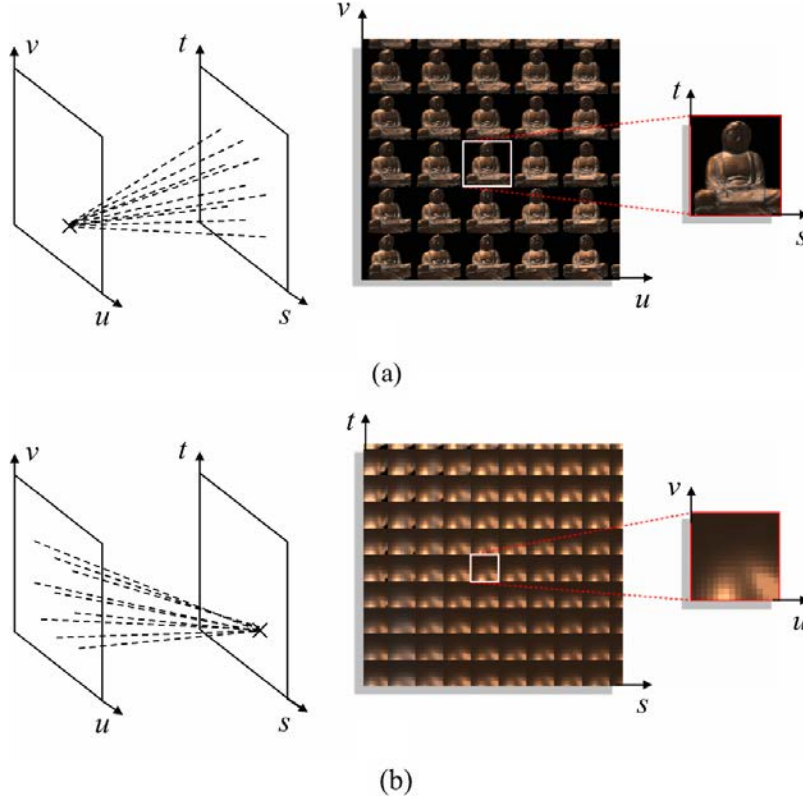
Fig. 4.3 The light field seen from (a) camera plane and (b) focal plane. The boxed subimage is observed from a single point in the parameter plane. (Images courtesy of Marc Levoy; ©1996 ACM, Inc. Included here by permission.)
