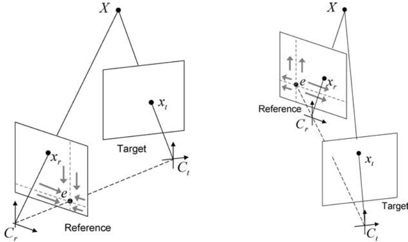
Fig. 6.3 The modified painter's algorithm can be used for forward mapping without requiring the Z -buffer. Left: Target camera is in front of reference (source) camera. Right: Target camera is behind the source camera.
