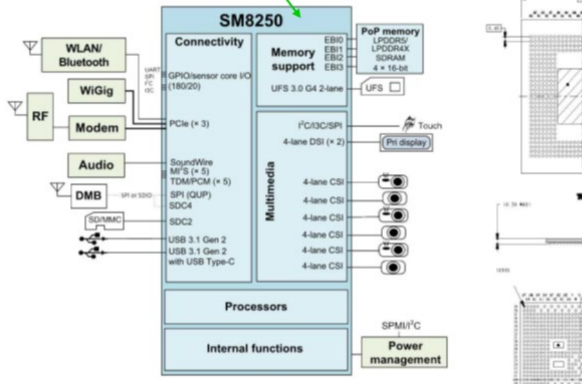
SM8250 high-level block diagram and 1099 (SM8250-LPDDR5) drawing
