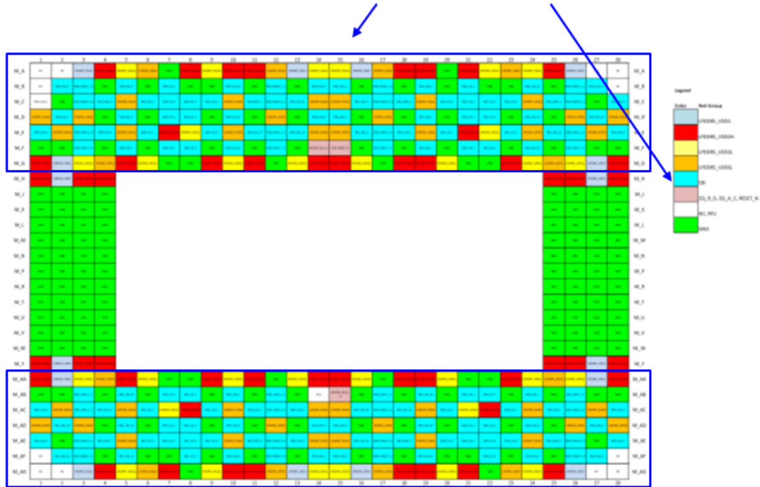
Figure 2-3 SM8450 top pin LPDDR5 assignments (top view)
