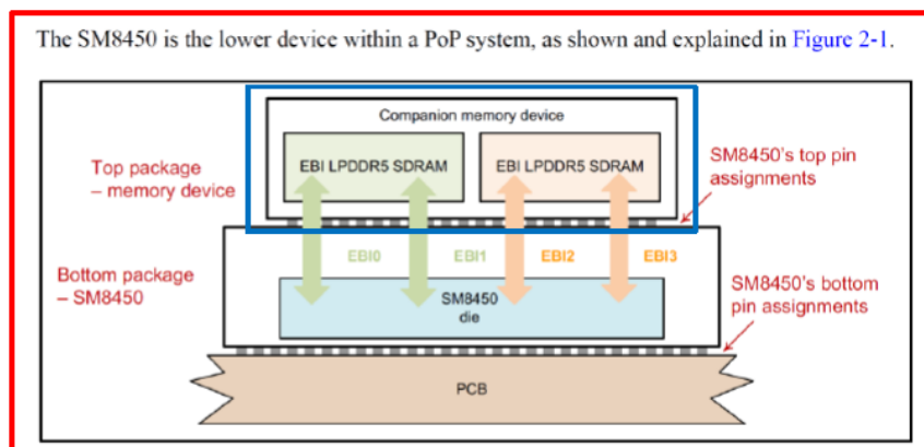
Figure 2-1 PoP system pin assignments
