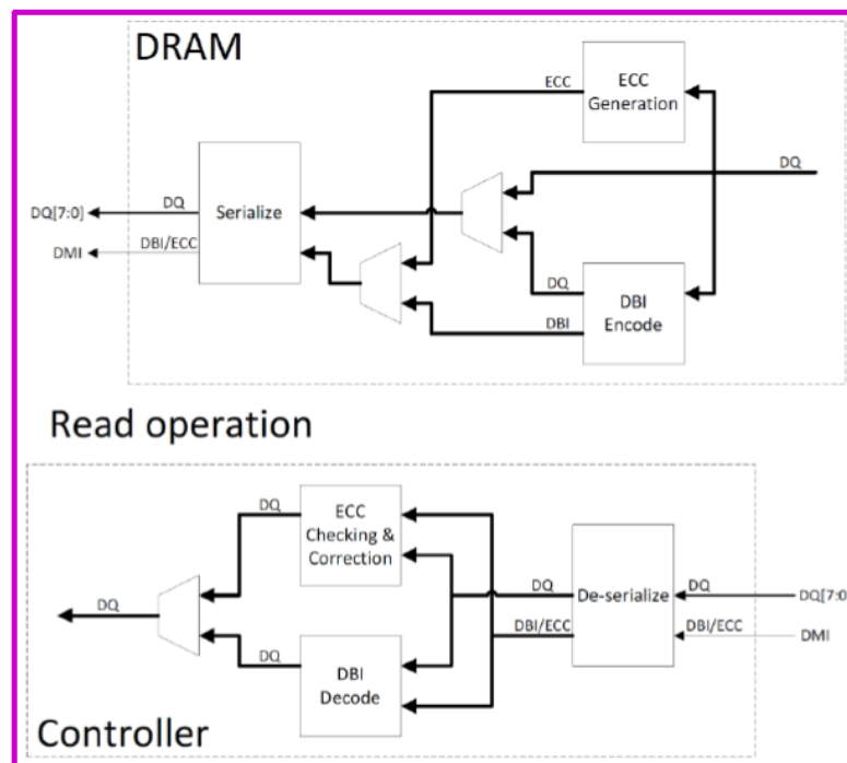
Figure 283 — Data Flow on a Memory Read Operation
