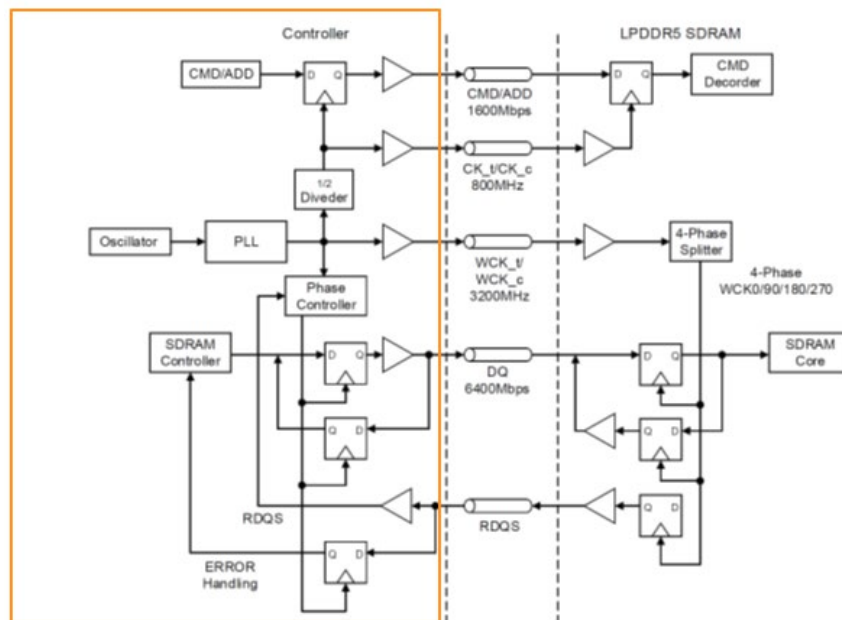
Figure 11 — Block Diagram of an Example System: CKR=4:1
