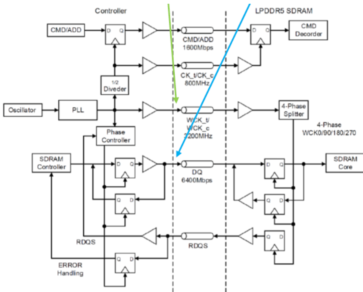
Figure 11 — Block Diagram of an Example System: CKR=4:1
