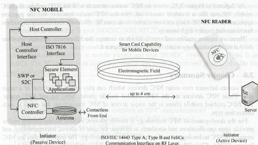
Figure 3.32 Communication architecture of card emulation operating mode.
