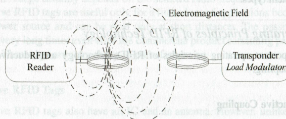
Figure 2.13 Inductive coupling.
