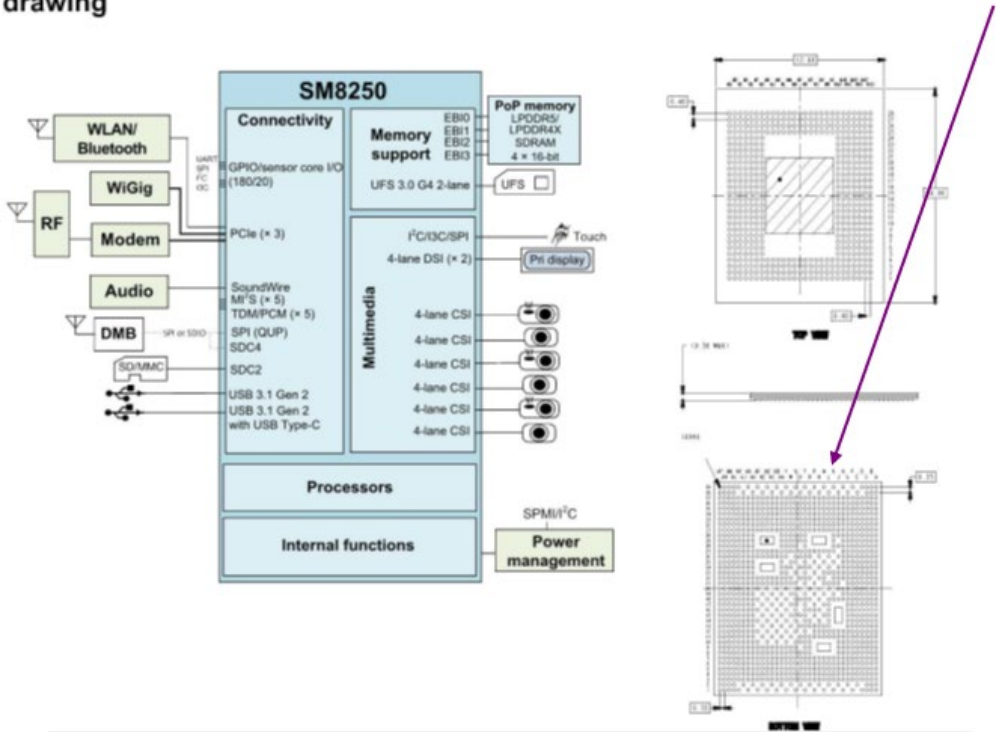
SM8250 high-level block diagram and 1099 (SM8250-LPDDR5)/1017 (SM8250-drawing
