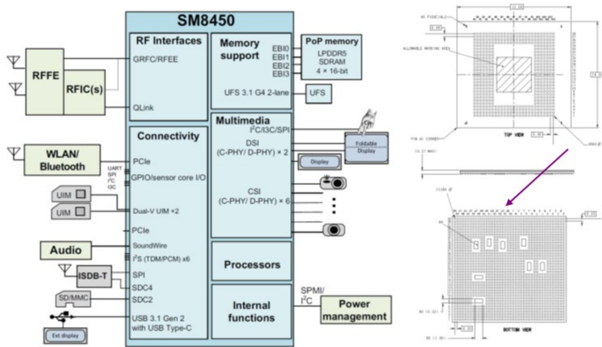
SM8450 high-level block diagram and MPSP1518 outline drawing
