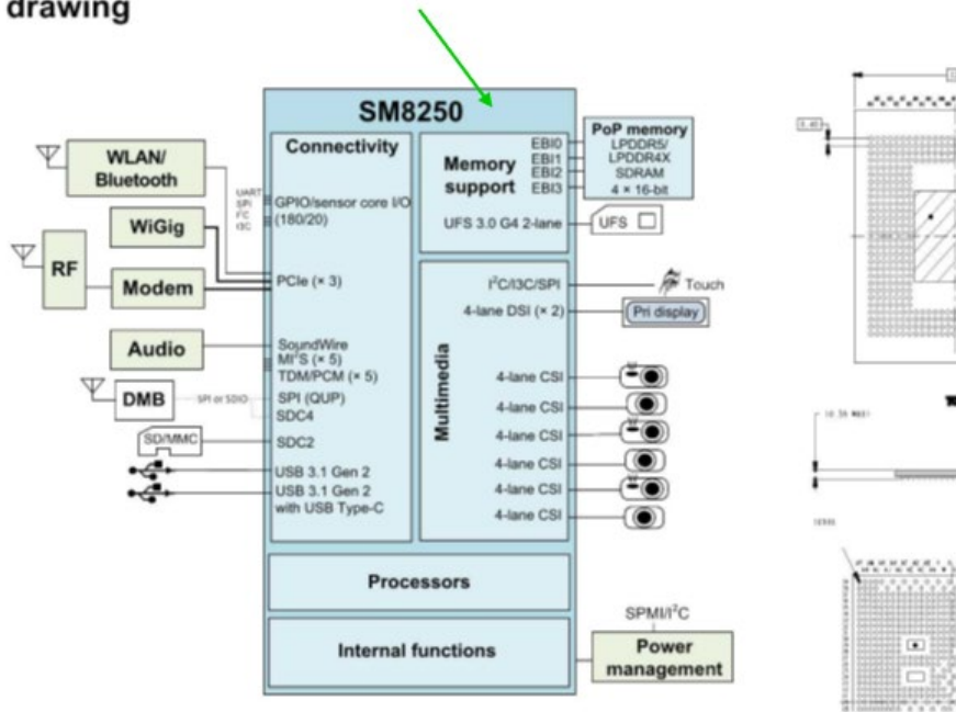
SM8250 high-level block diagram and 1099 (SM8250-LPDDR5) drawing
