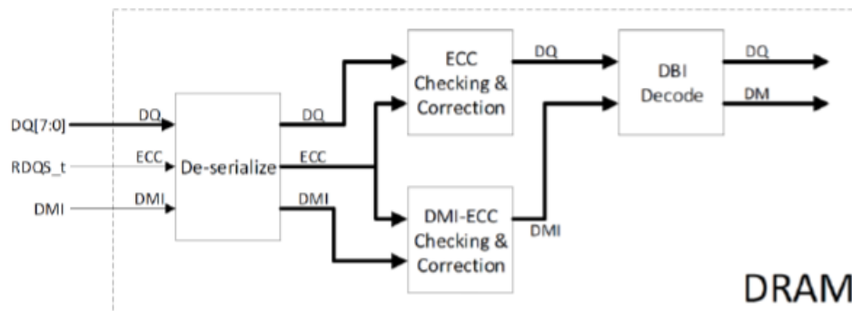
Figure 282 — Data Flow on a Memory Write Operation
