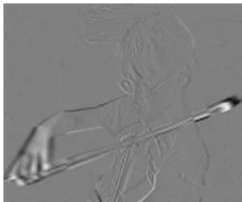
Figure 3.6 Difference
