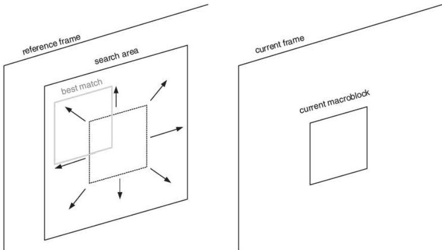
Figure 3.9 Motion estimation
