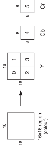
Figure 3.8 Macroblock (4:2:0)
