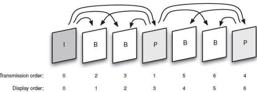
Figure 5.5 Display order: Type 1 example
