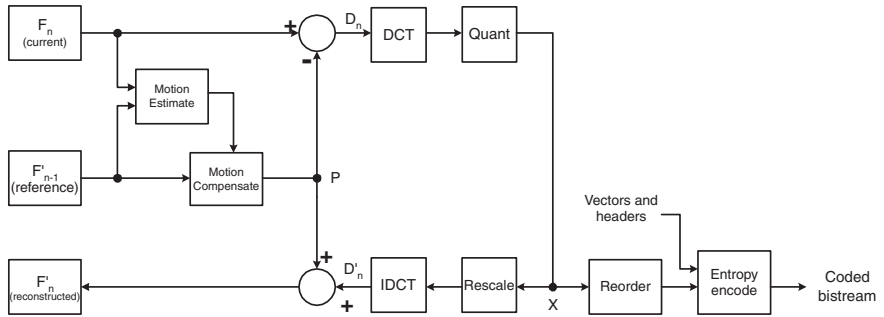
Figure 3.51 DPCM/DCT video encoder
