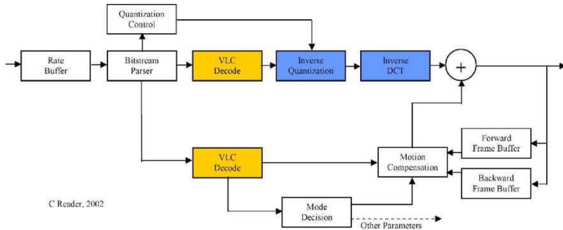
Figure 2b MPEG Video Decoder
