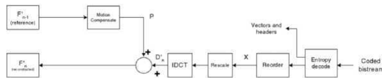
Figure 3.51 DPCM/DCT video decoder
