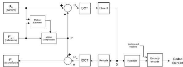
Figure 3.50 DPCM/DCT video encoder
