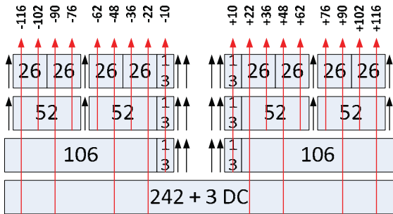
Figure 26-18 - Pilot tone locations for 20 MHz
