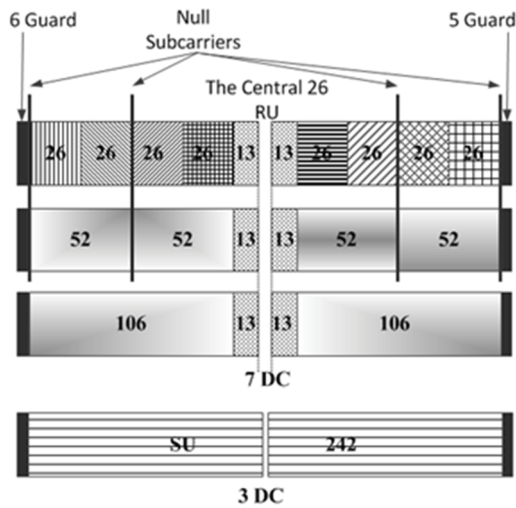
Figure 26-15 - RU locations in a 20 MHz HE PPDU
