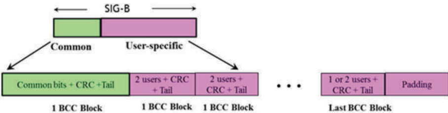
Figure 26-23 – HE-SIG-B field encoding structure in each 20 MHz
