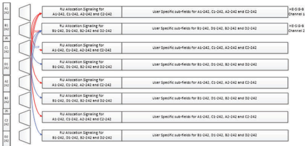
Figure 26-27 - Default mapping of the two HE-SIG-B channels and their duplication in a 160 MHz PPDU
