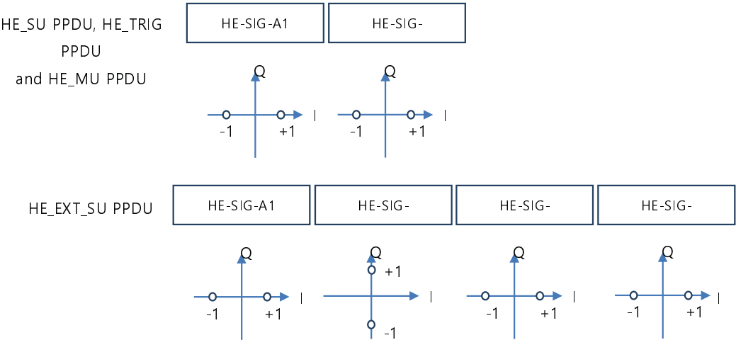
Figure 26-22 - Data tone constellation of HE-SIG-A symbols
