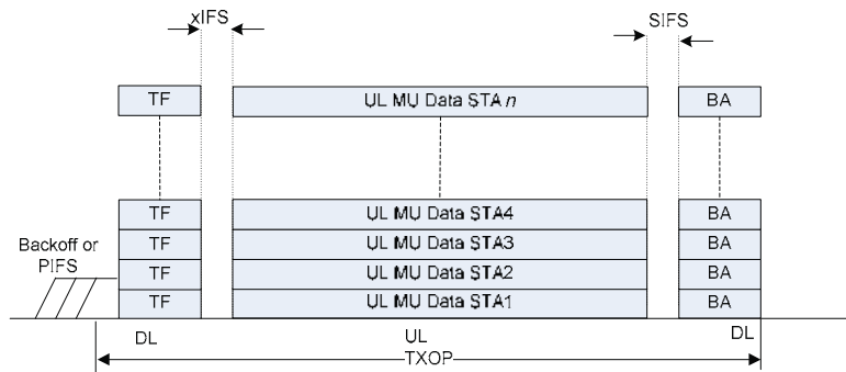
Figure 10-5 - An example of a TXOP containing an UL MU transmission with an immediate DL MU transmission containing unicast BlockAck frames acknowledging the frames received from the respective STAs
