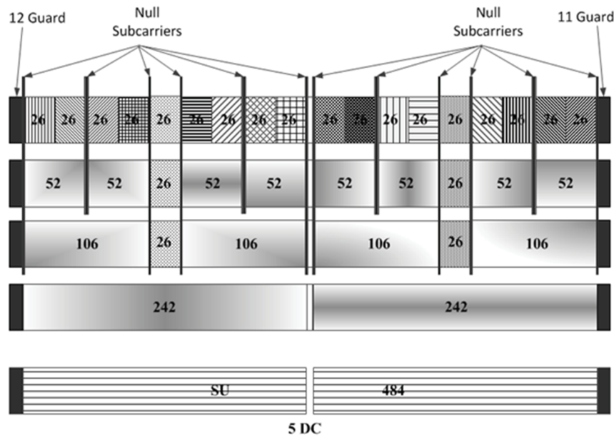
Figure 26-16 - RU locations in a 40 MHz HE PPDU
