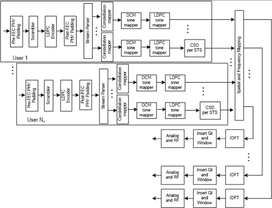
Figure 26-11 - Transmitter block diagram for the Data field of an HE downlink MU-MIMO transmission in 106-, 242-, 484- or 996-RU with LDPC encoding
