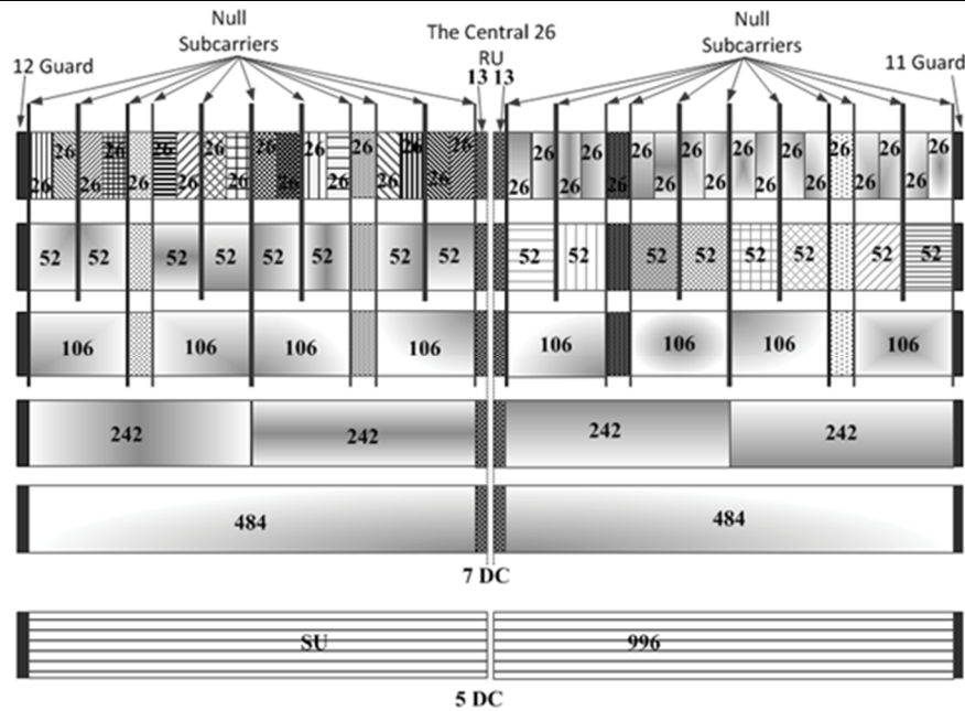
Figure 26-17 - RU locations in an 80 MHz HE PPDU
