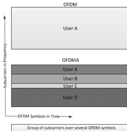
Figure 26-14 - Illustration of OFDM and OFDMA Concepts
