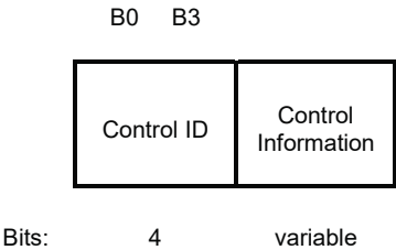
Figure 9-14b - Control subfield format
