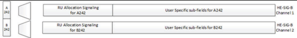
Figure 26-25 - HE-SIG-B content channels for a 40 MHz PPDU
