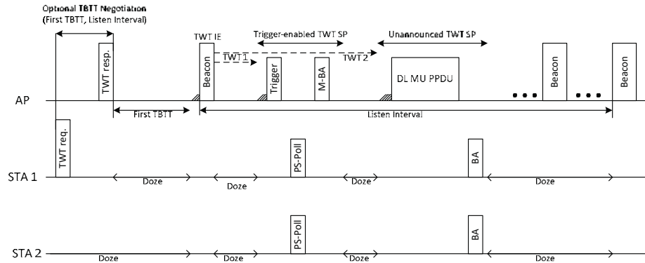
Figure 10-10 - Example of broadcast TWT operation
