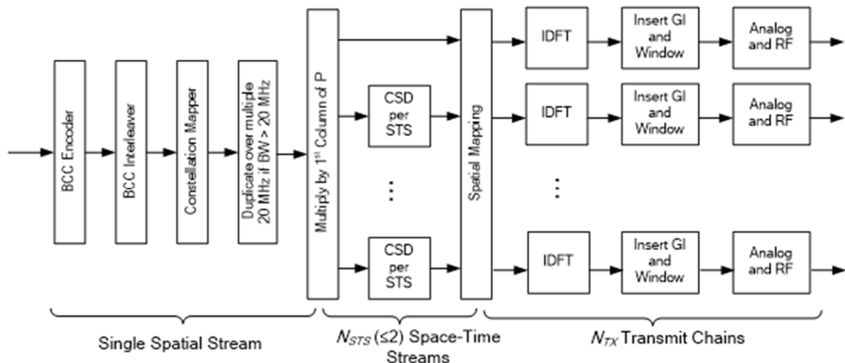
Figure 26-7 – Transmitter block diagram for the L-SIG, RL-SIG and HE-SIG-A fields when the Beam Change field is 0
