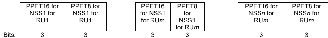
Figure 9-554ae - PPE Threshold Info field format
