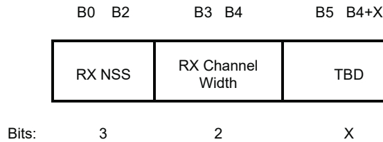
Figure 9-14d - Control Information subfield format when Control ID subfield is 1
