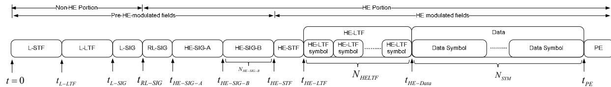
Figure 26-21 - Timing boundaries for HE PPDU fields
