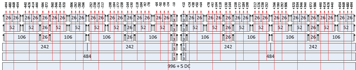
Figure 26-20 - Pilot tone locations for 80 MHz
