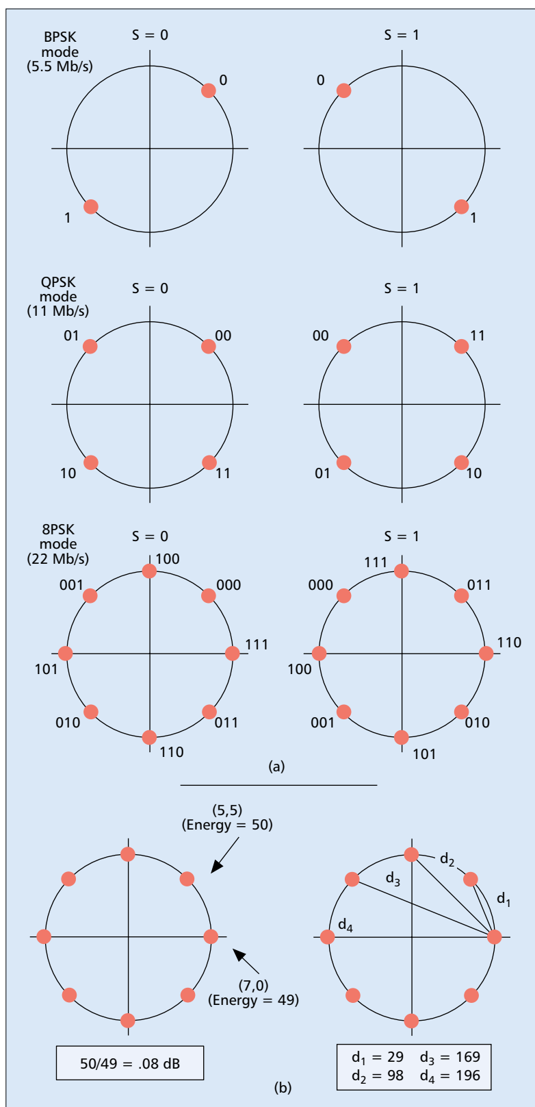
Figure 4. Modulation symbols.
