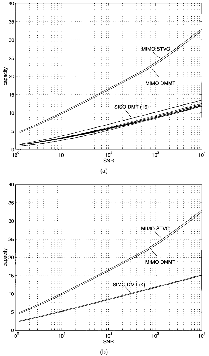
Fig. 6. Channel capacity experimental results for L = 3 .
