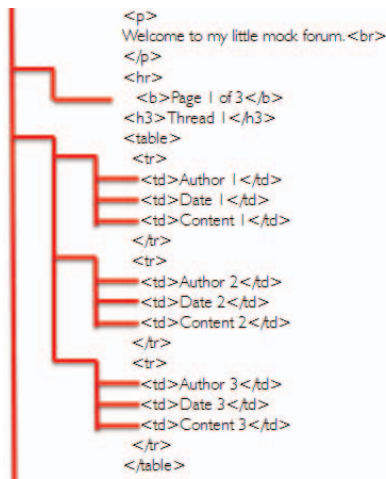
Figure 5 - HTML content as a tree.
