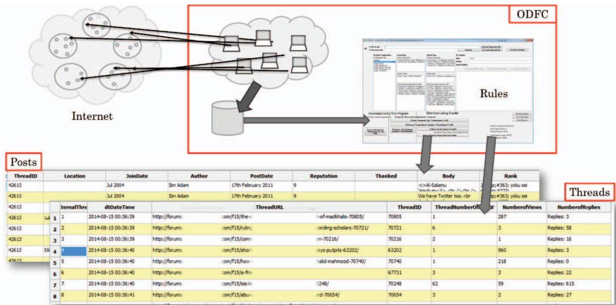
Figure 1 - A summary of the data capture process
