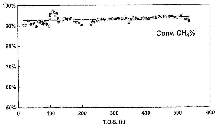
Figure 62 CPO with methane feed and oxygen as oxidant [161]. P=1.5\text{ Mpa} . \text{H}_2\text{O}/\text{CH}_4=0.26 ; \text{CO}_2/\text{CH}_4=0.11 ; \text{O}_2/\text{CH}_4=0.56
