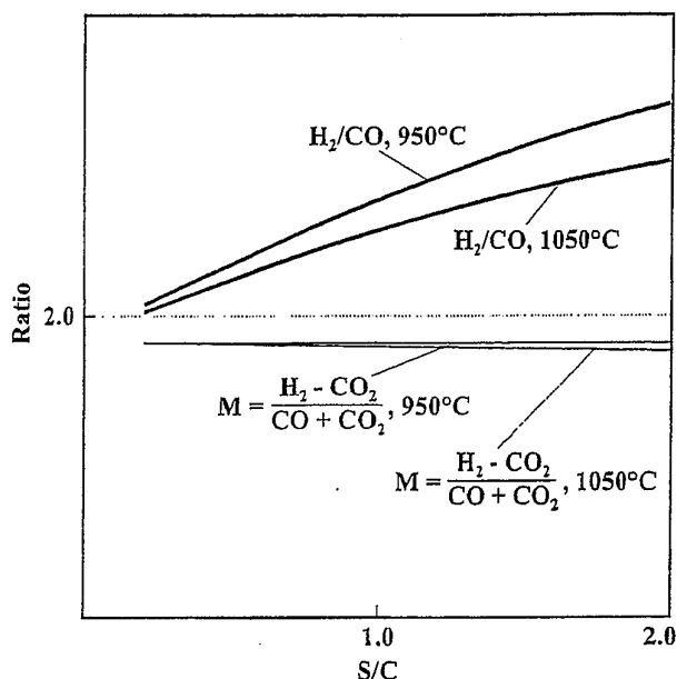
Figure 47 M and H 2 /CO in raw gas from ATR
