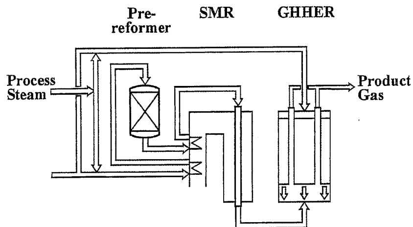
Figure 35 Tubular Reformer (SMR) and Gas Heated Reformer ('two-in, one-out', GHHER) in parallel arrangement
