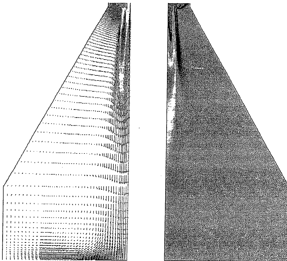
Figure 56 Example of CFD modelling results for the combustion chamber in an ATR reactor. The left part show velocity vectors and the right part show temperatures. [134]
