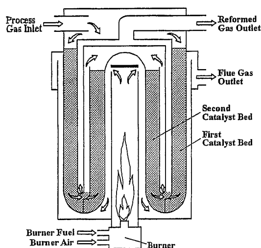
Figure 28 Topsøe Heat Exchange Reformer (HER) [57]
