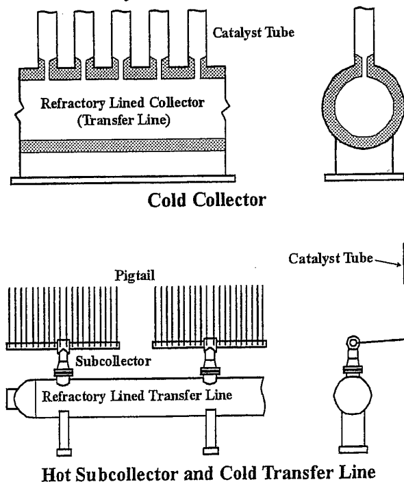
Figure 19 Typical designs of gas outlet systems [4]
