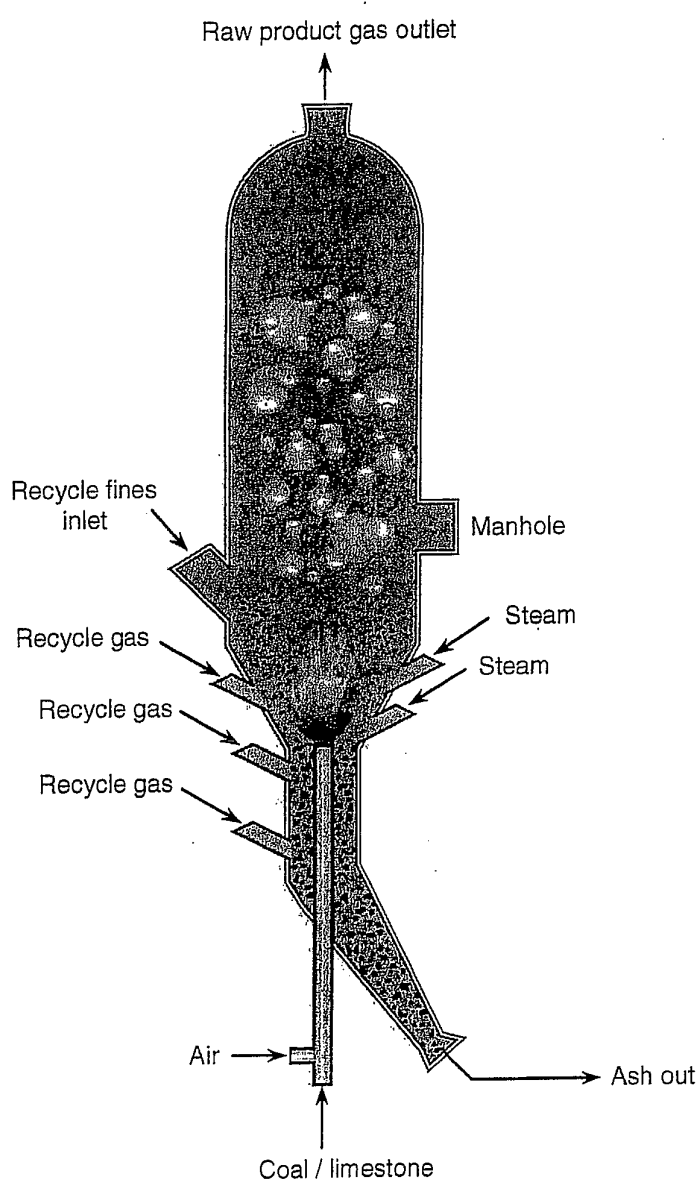
Figure 70 KRW gasifier [192]
