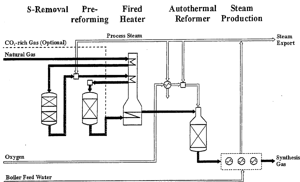
Figure 12 Typical layout of the syngas generation unit with adiabatic prereformer in a GTL plant [26].
