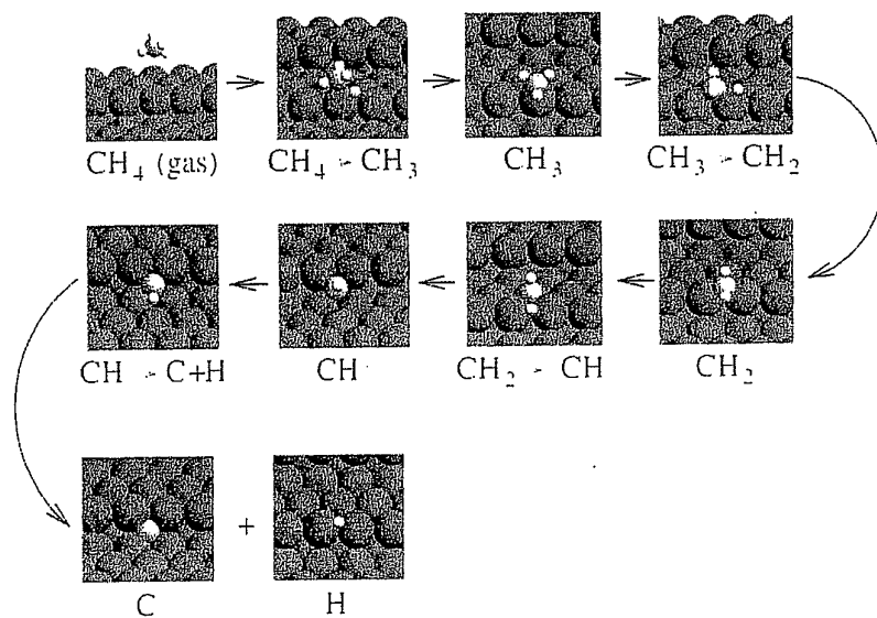
Figure 43 Calculated structures of intermediates and transition states for all elementary processes in the methane activation reactions on the step sites of a Ni(211) surface [89].
