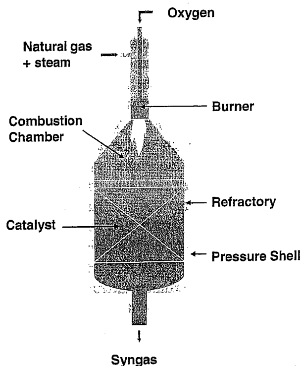
Figure 55 Illustration of an ATR reactor [taken from 132].
