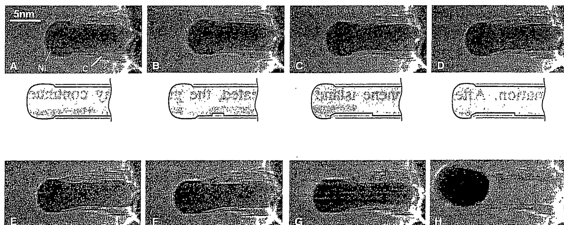
Figure 46 Image sequence of the initial carbon formation on a Ni/MgAl 2 O 4 catalyst. Drawings are included to guide the eye in locating the positions of mono-atomic Ni step edges at the C-Ni interface. The images are acquired in situ with CH 4 :H 2 = 1:1 at a total pressure of 2.1mbar with the sample heated to 536°C.
