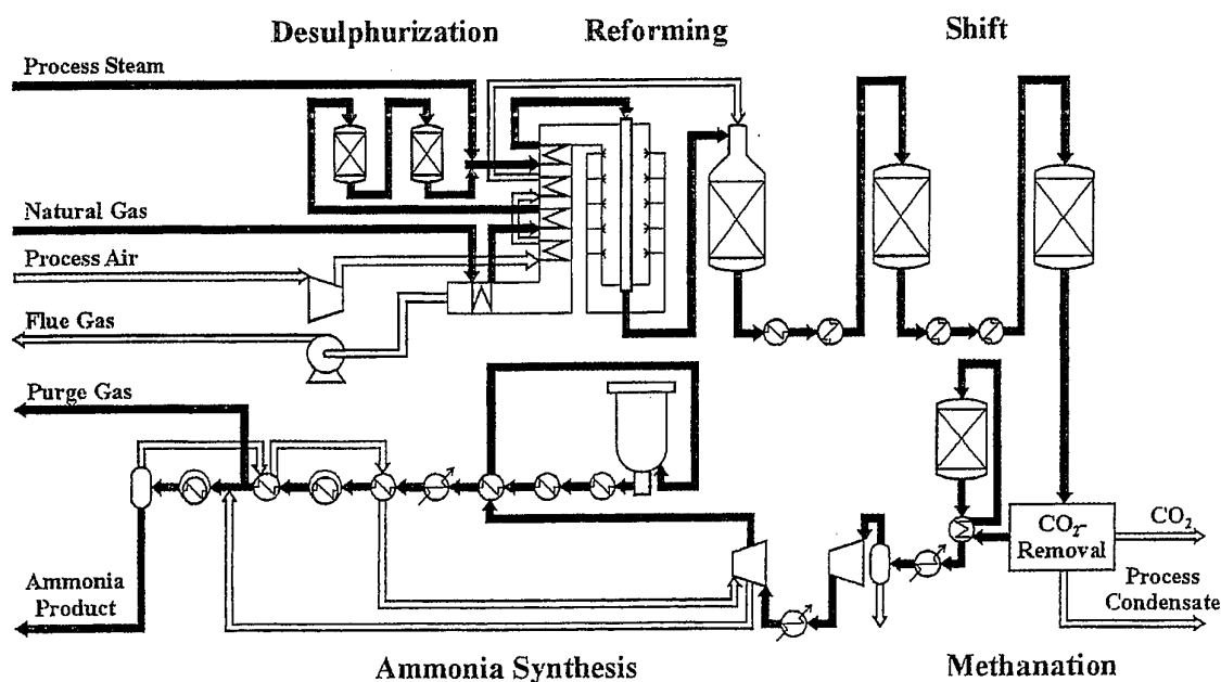
Figure 51 Complete ammonia plant [108]
