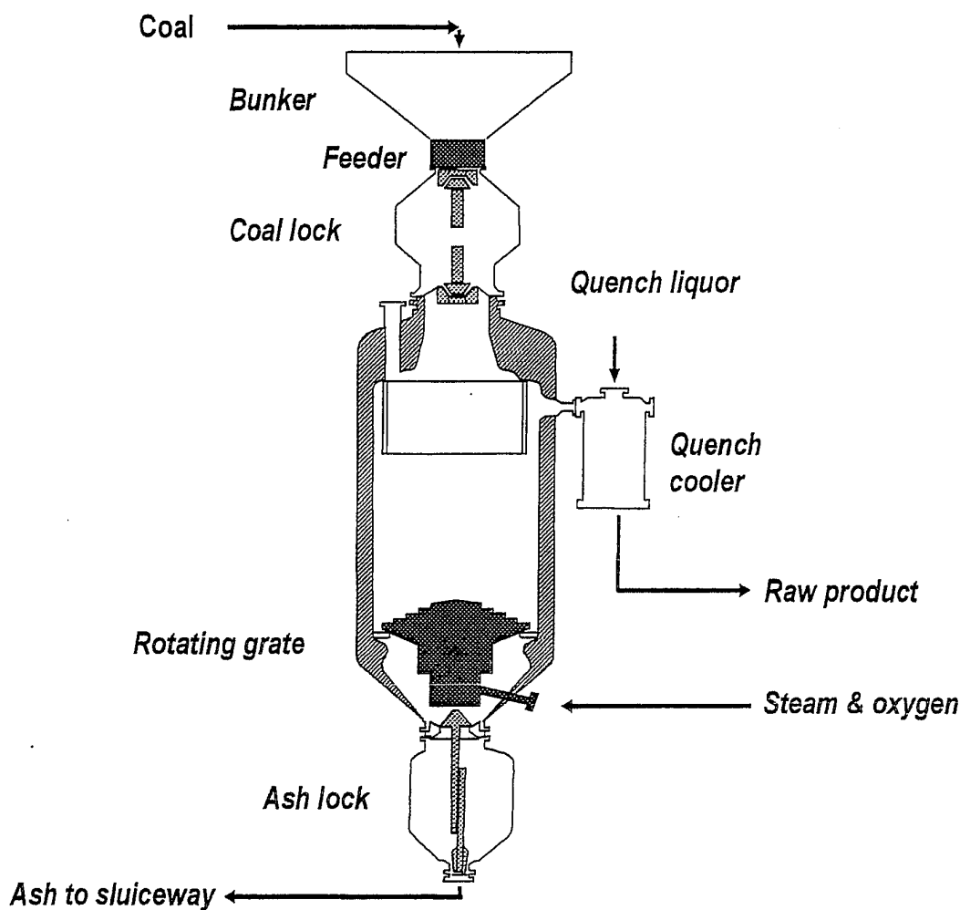
Figure 66 Sasol-Lurgi fixed bed dry bottom gasifier [191]
