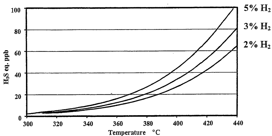
Figure 5 Equilibrium \text{H}_2\text{S} , 5% \text{CO}_2 in natural gas
