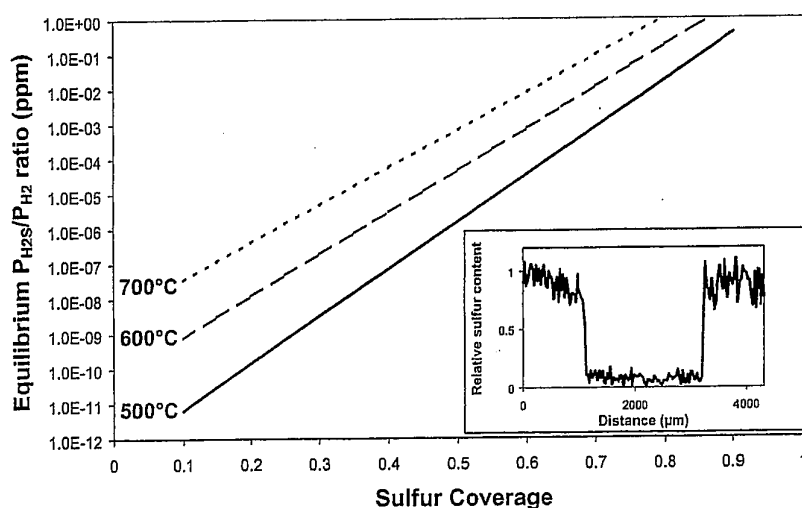
Figure 38 Equilibrium P_{\text{H}_2\text{S}}/P_{\text{H}_2} ratio as a function of the sulphur coverage.
