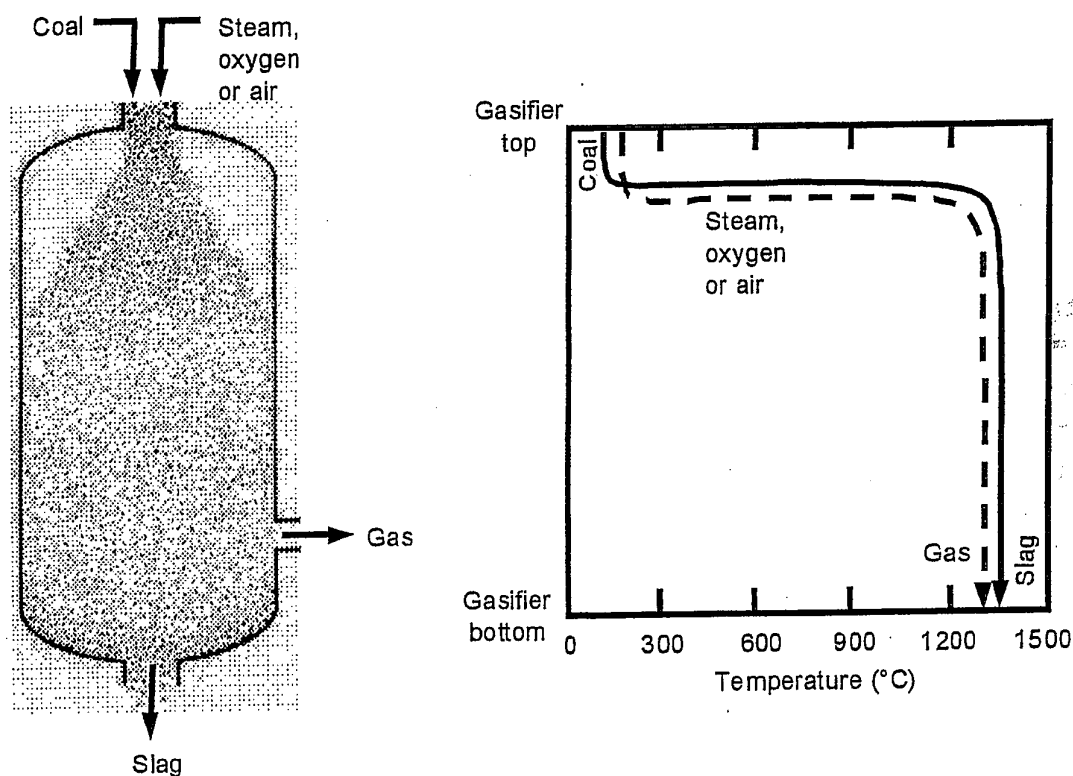
Figure 73 Entrained flow gasifier and typical temperature profile [174].
