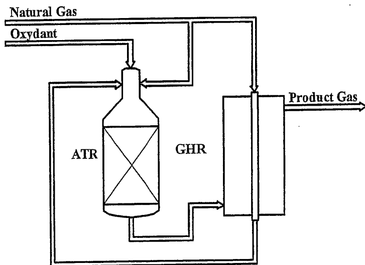
Figure 32 'Combined Reforming with GHR': Autothermal reformer (ATR) and Gas Heated Reformer (GHR) in series arrangement with partial by-pass of feed over the GHR.
