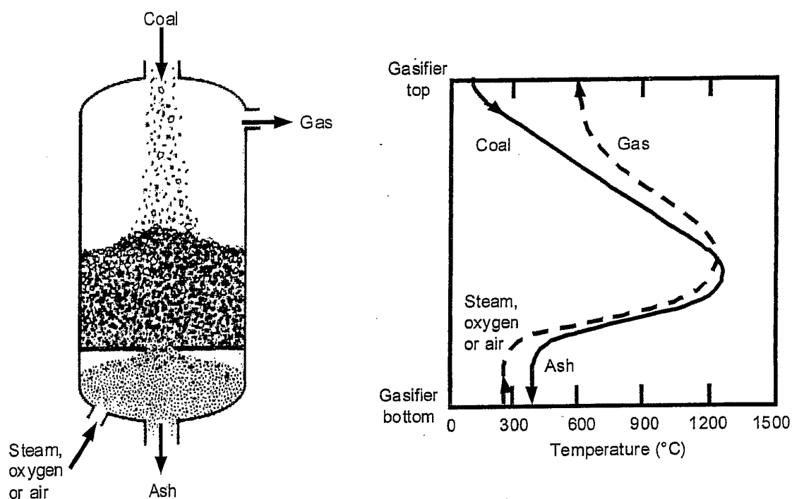
Figure 67 Lurgi dry bottom gasifier and typical temperature profile [174]
