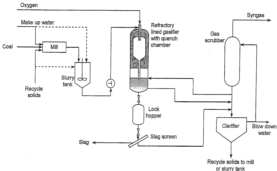
Figure 74 Texaco gasifier with quench cooling[1]
