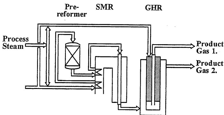
Figure 33 Tubular reformer (SMR) and Gas Heated Reformer ('Two-in, two-out', GHR) in parallel arrangement
