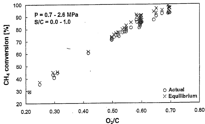
Figure 63 Methane conversion in CPO pilot plant experiments with air as oxidant [167]
