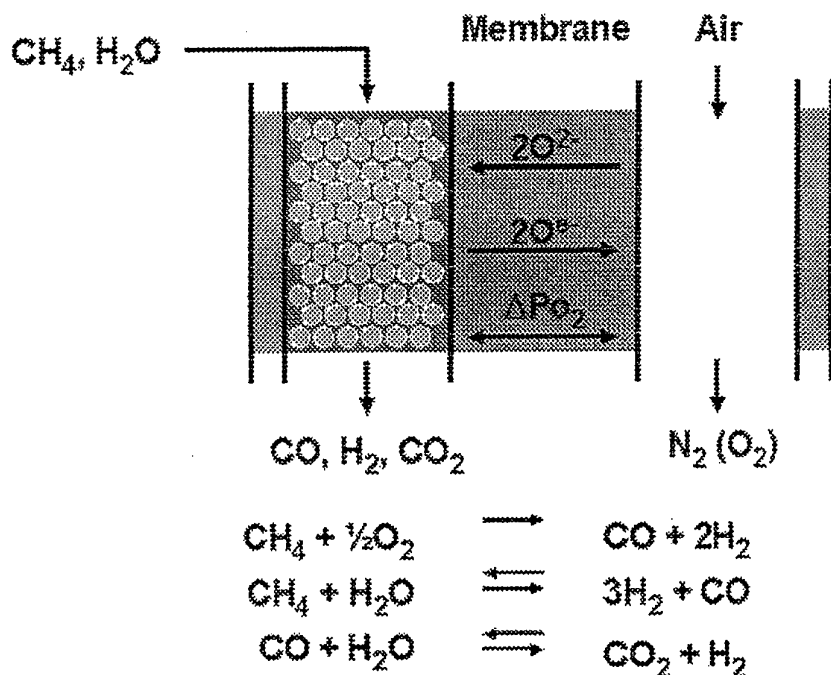
Figure 64 Principle of oxygen membrane reforming
