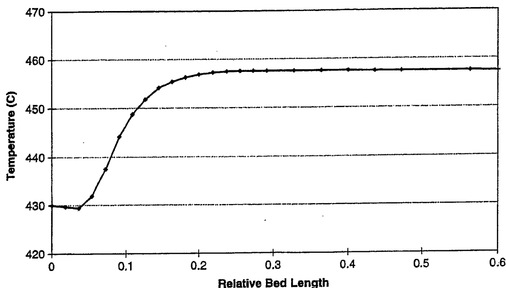
Figure 13 Temperature profile in adiabatic prereformer during pilot plant operation. H_2O/C = 0.4 [26].
