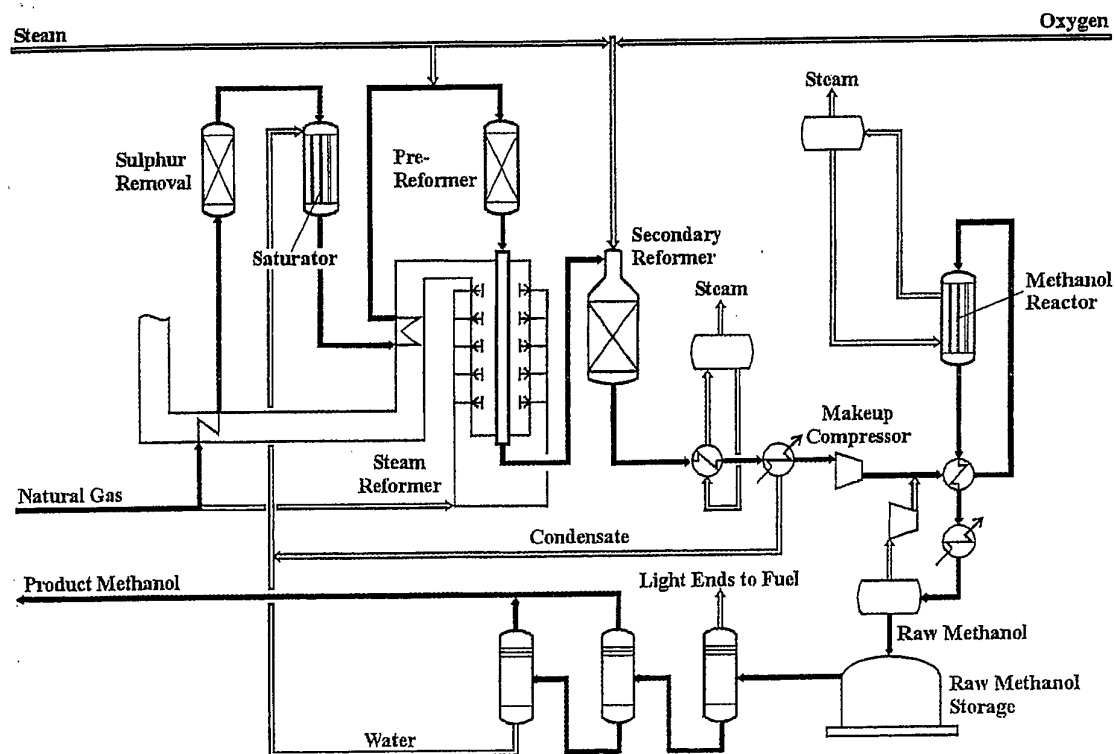
Figure 52 Methanol production by two-step reforming [104].
