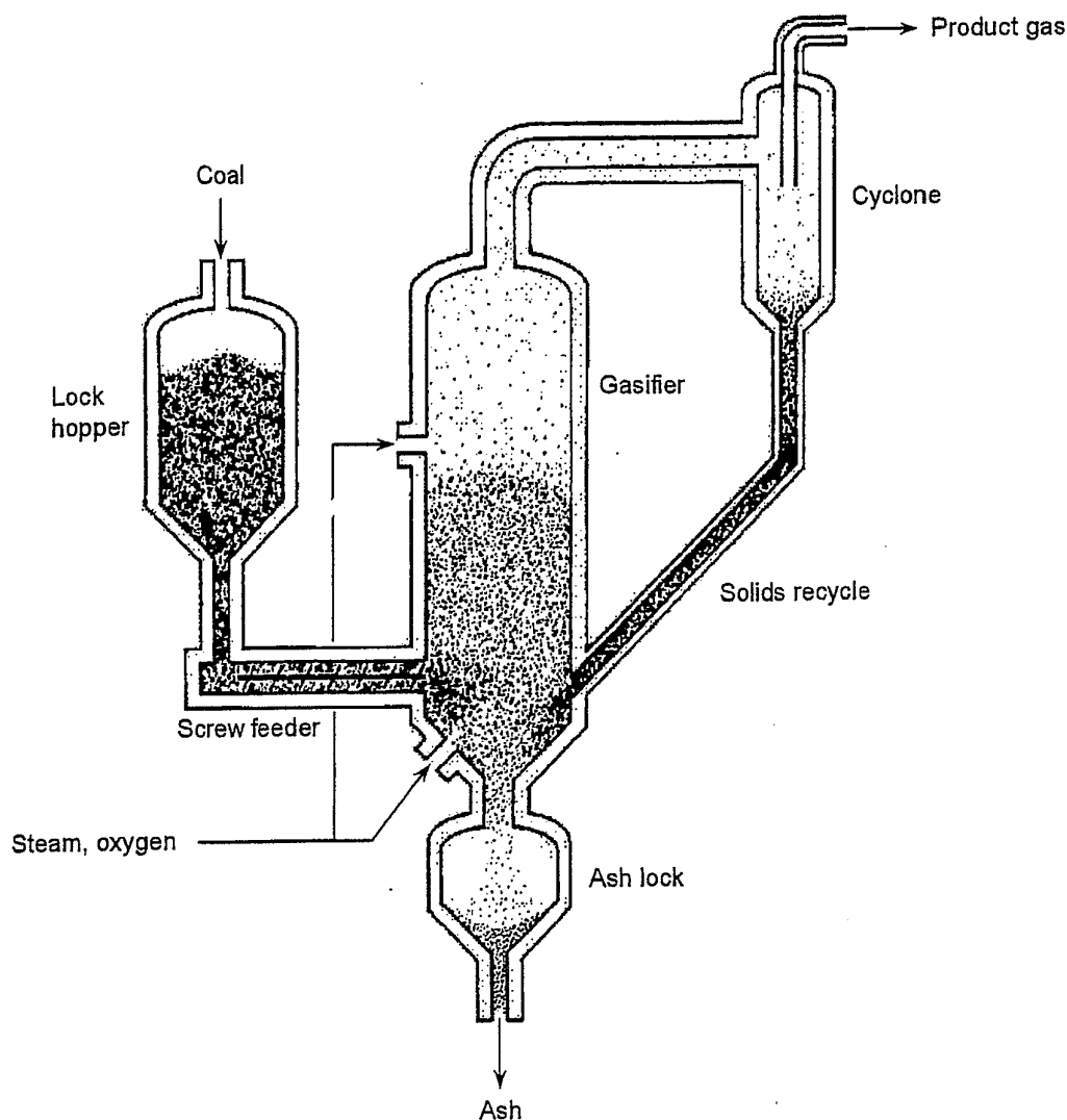
Figure 71 HTW gasifier [174, see also 177]
