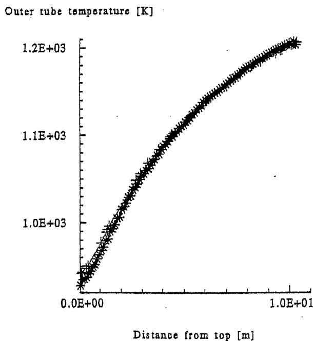
Figure 25 Calculated and measured outer tube wall temperature Measured Outer Tube Wall Temperature [56]
