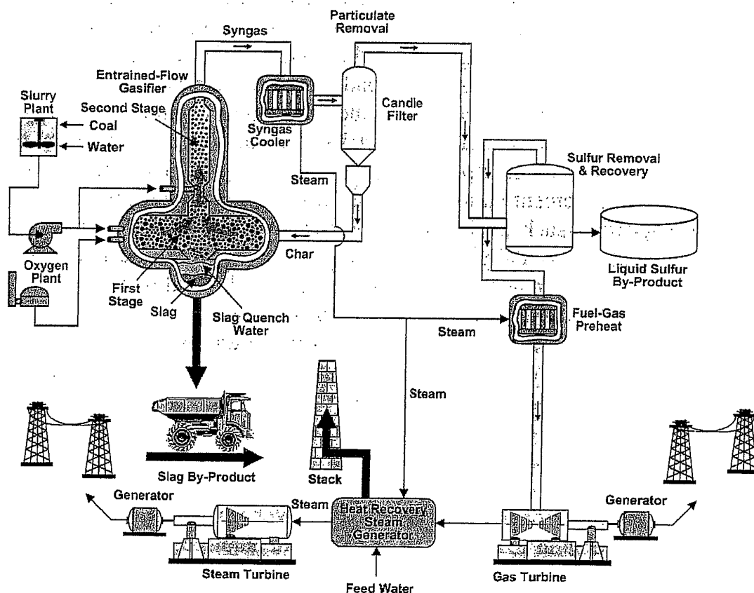
Figure 78 Wabash River Coal Gasification Repowering plant [215]
