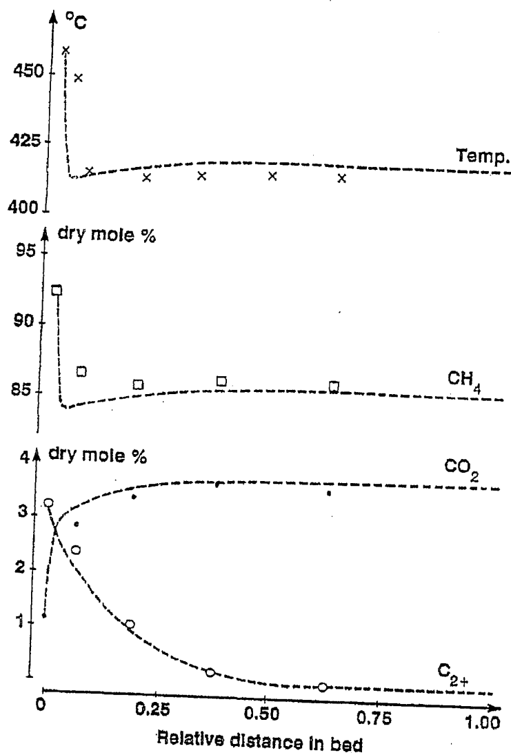
Figure 14 Temperature and conversion profiles for prereforming of natural gas, \text{H}_2\text{O}/\text{C} ratio = 0.40, P = 8 bar. Measured data: x - temperature; \square - \text{CH}_4 concentration, \bullet - \text{CO}_2 concentration; o - \text{C}_{2+} concentration. Calculated profiles are shown as dashed lines. [22].
