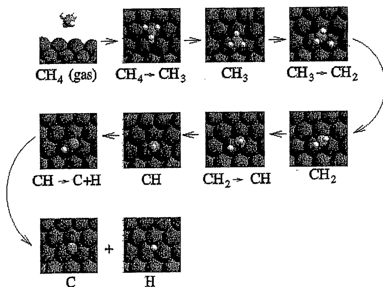
Figure 42 Calculated structures of intermediates and transition states for all elementary processes in the transformation of methane into adsorbed carbon and hydrogen on a Ni(111) surface [89].
