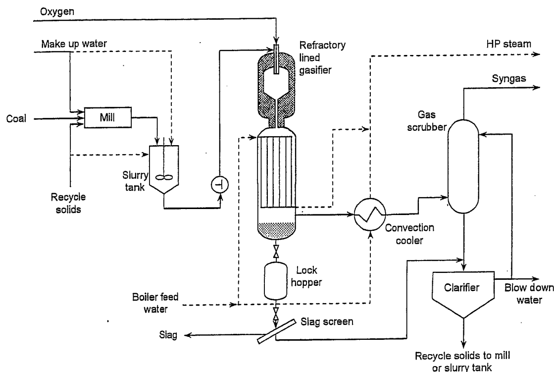
Figure 75 Texaco gasifier with radiant cooling [1].
