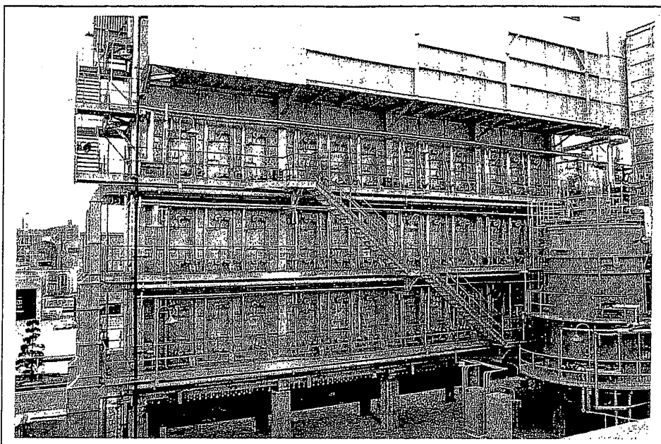
Figure 17 Photo of Topsøe Reformer [34]
