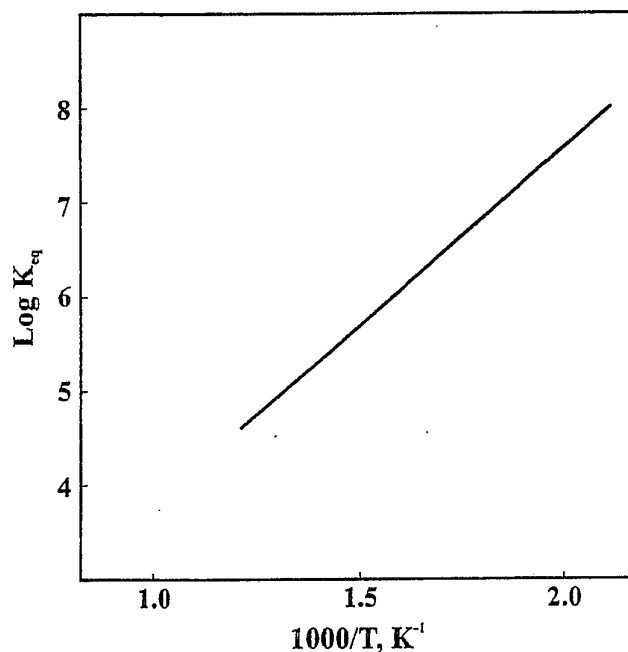
Figure 4 Equilibrium constant for reaction (11)
