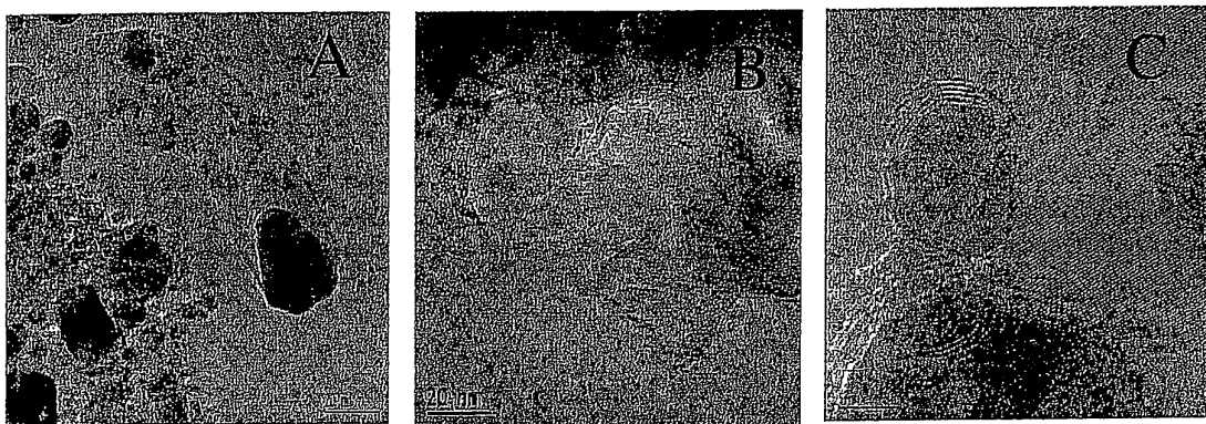
Figure 39 Electron microscopy pictures of whisker carbon (a), pyrolytic carbon on a ceramic carrier b), and encapsulating carbon (c). C_nH_m : Higher hydrocarbons (hydrocarbons with two or more carbon atoms)
