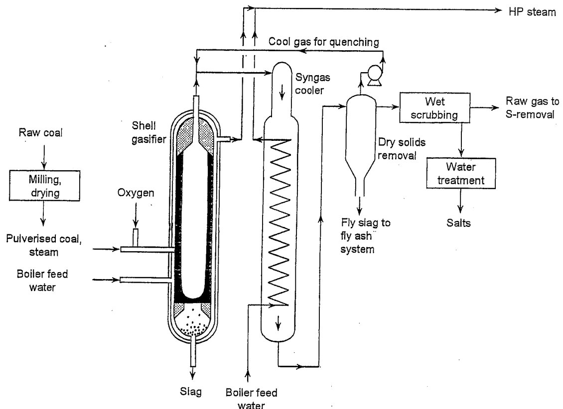
Figure 76 Shell gasifier [218, 219]
