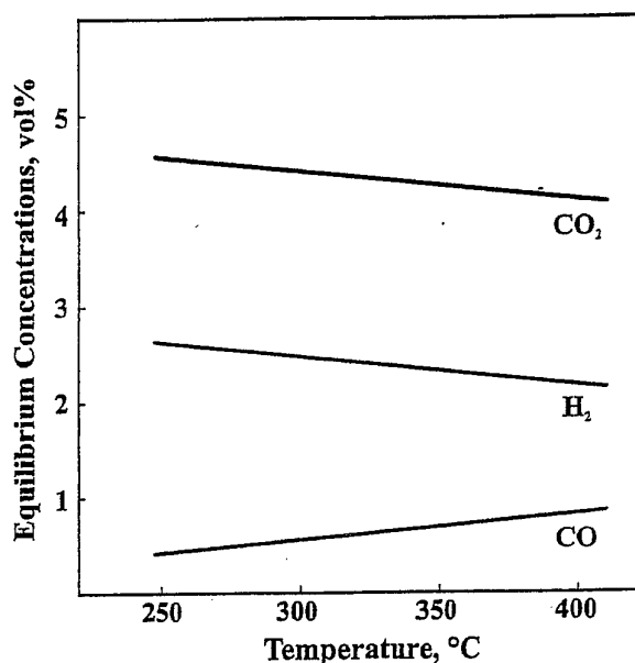
Figure 6 Equilibrium concentrations of CO , CO_2 , and H_2 ; 3% H_2 and 5% CO_2 in the feed
