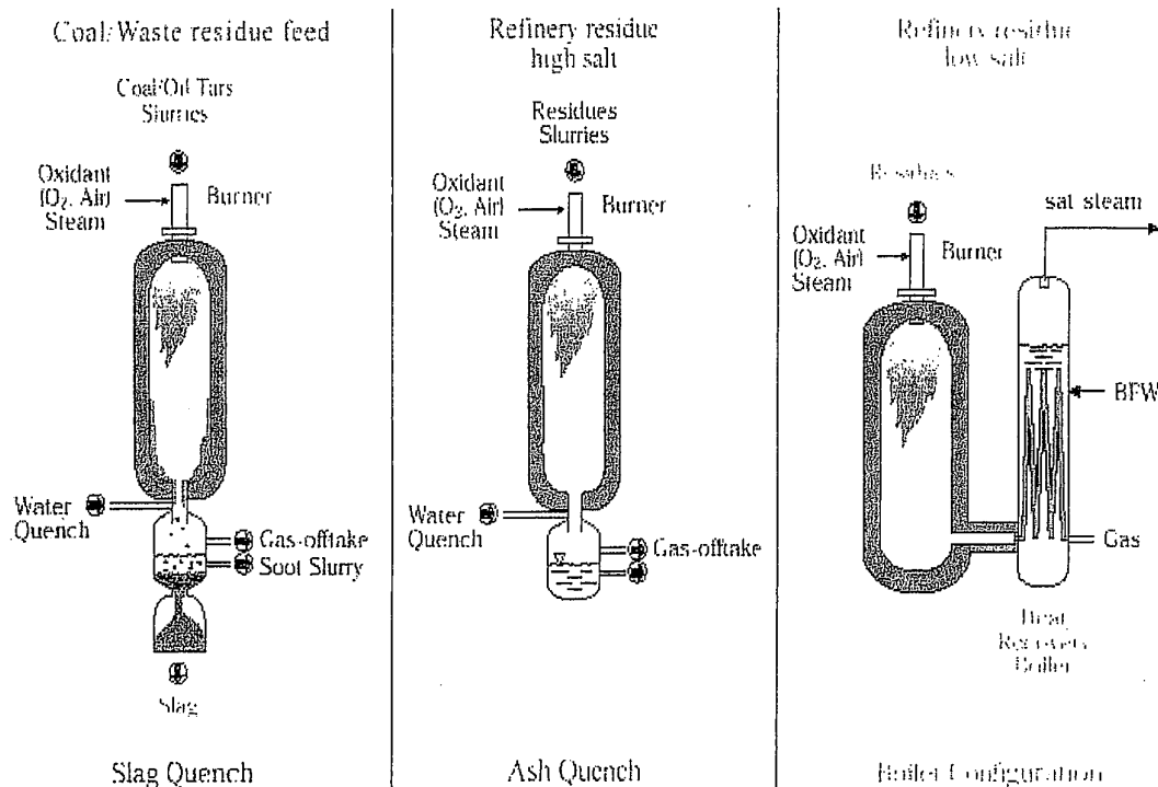
Figure 77 Different modes of operation for a MPG [211]
