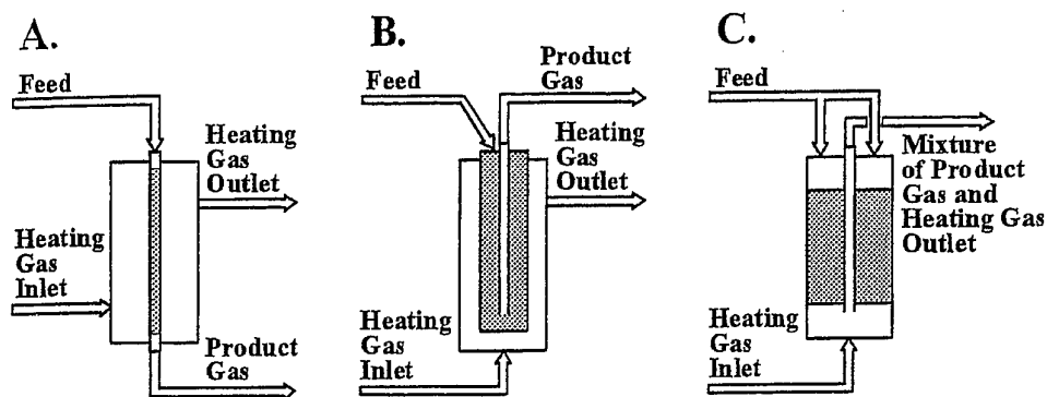
Figure 27 A: Concept with 'straight-through' tubes; B: Concept with bayonet tubes; C: Concept with mixing of heating gas and product gas before heat exchange.
