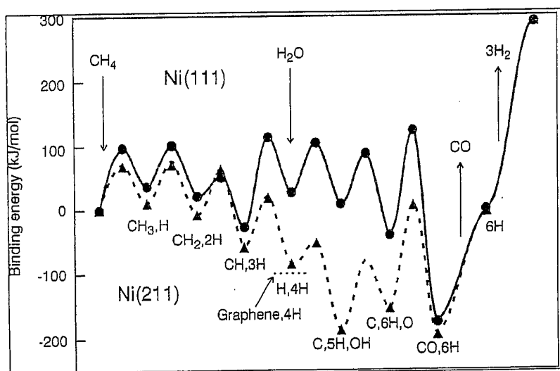
Figure 44 Calculated energies along the reaction path for steam reforming on the Ni(111) and Ni(211) surfaces. The corresponding structures are shown in Figs. 42 and 43. All energies are given relative to a situation in which all reactants are in the gas phase far from the clean surface [89].
