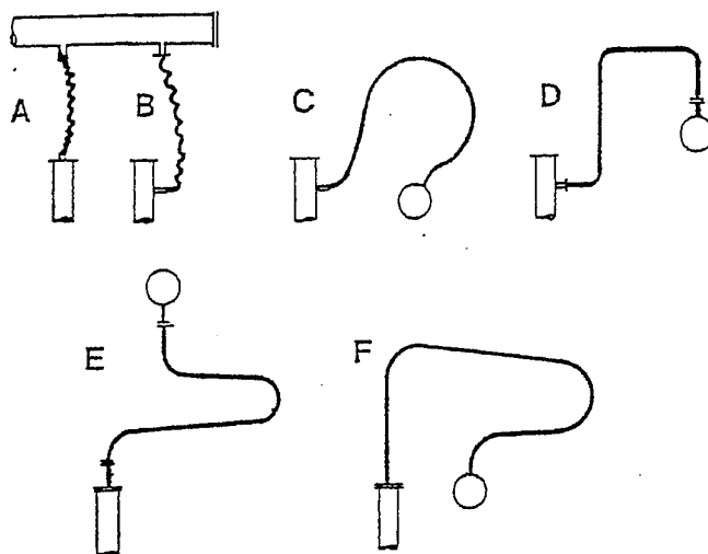
Figure 18 Typical design of gas inlet systems
