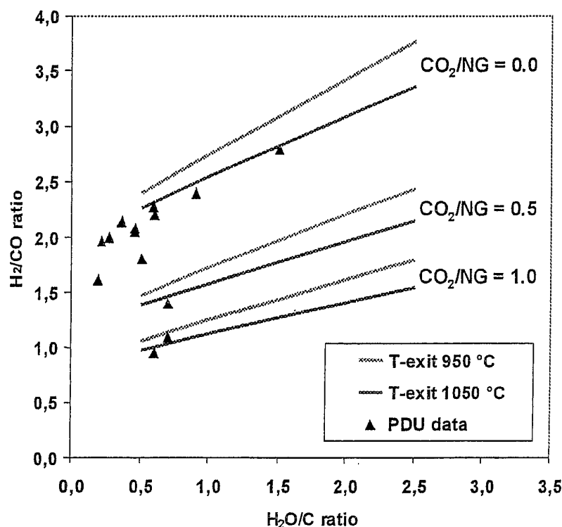
Figure 60 Syngas equilibrium; experimental data from soot-free ATR-operation [155]
