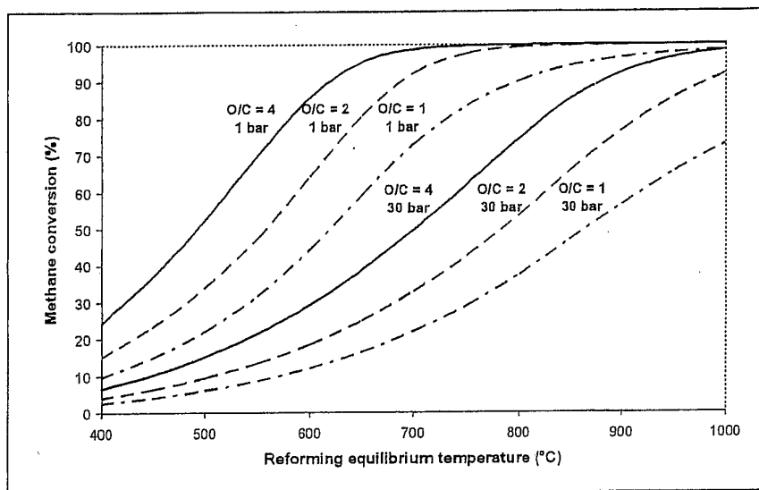
Figure 8 Steam reforming and methane conversion (O/C: ratio of steam to methane in the feed gas).
