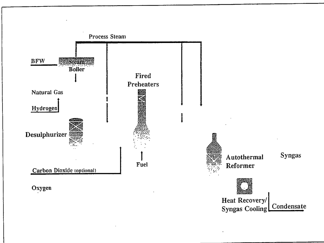
Figure 59 Process layout of ATR Process Demonstration Unit
