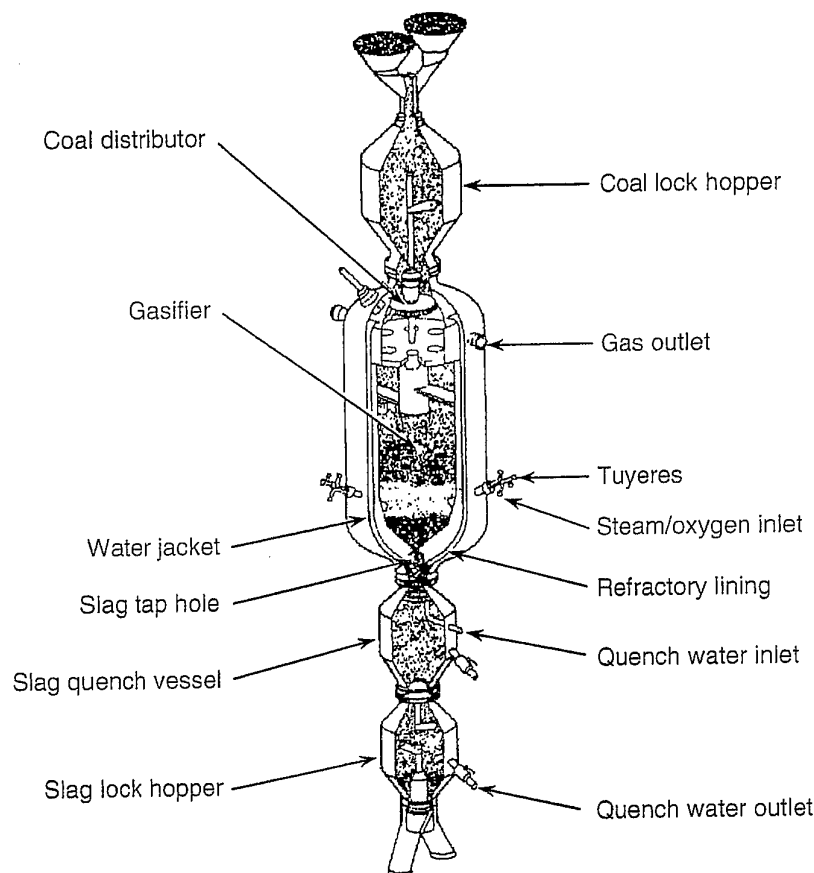
Figure 68 BGL gasifier [174, see also 177]
