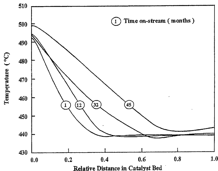
Figure 10 Temperature profile of an adiabatic prereformer with natural gas feed in a 1600 MTPD ammonia plant [22]. H_2O/C=2.8 P=35 bars. The movement of the temperature profile with time is due to catalyst poisoning by sulphur (see Section 2.3.5.2).
