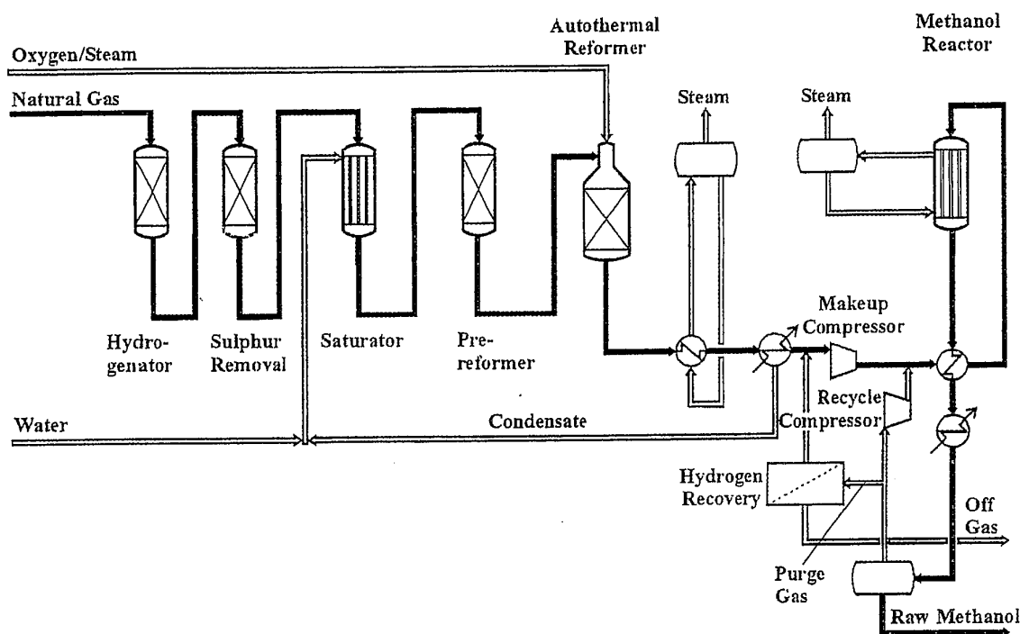
Figure 49 Methanol production by ATR and H_2 recovery and recycle [104]
