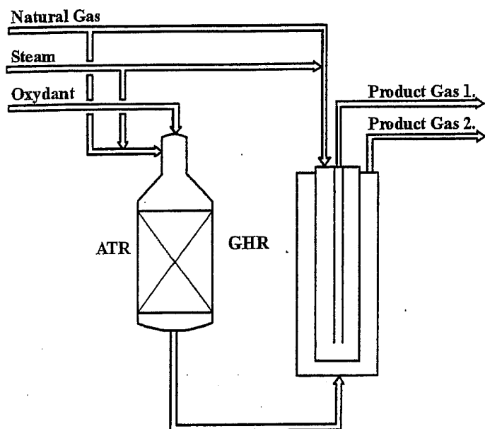
Figure 34 Autothermal reformer (ATR) and Gas Heated Reformer ('Two-in, two-out', GHR) in parallel arrangement
