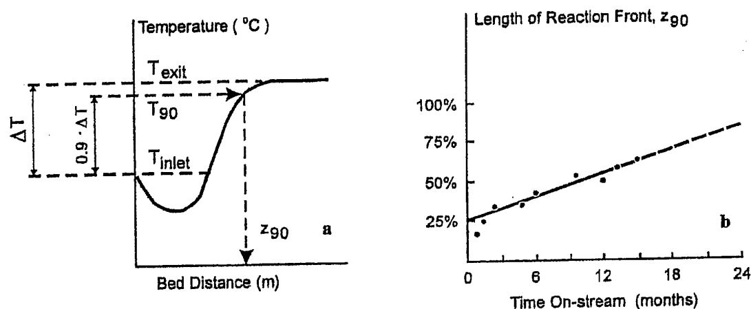
Figure 11 Graphical deactivation plot for performance prediction [25]. a) Estimation of length of reaction front, z_{90} from temperature profile. b) Deactivation plot.
