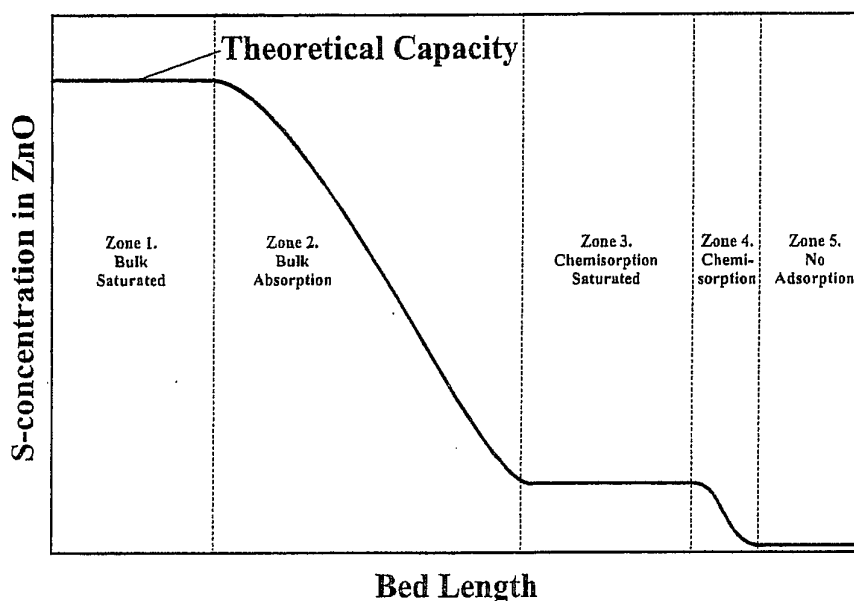
Figure 7 Ideal sulphur profile in a zinc oxide bed
