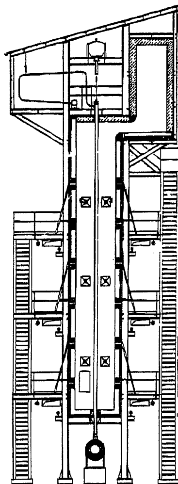
Figure 16 Cross section of side fired reformer
