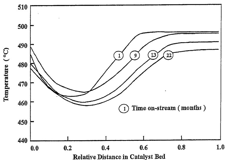
Figure 9 Temperature profile of an adiabatic prereformer with naphtha feed [22]. H_2O/C=3.5 . P=26 bars. The movement of the temperature profile with time is due to catalyst poisoning by sulphur (see Section 2.3.5.2).
