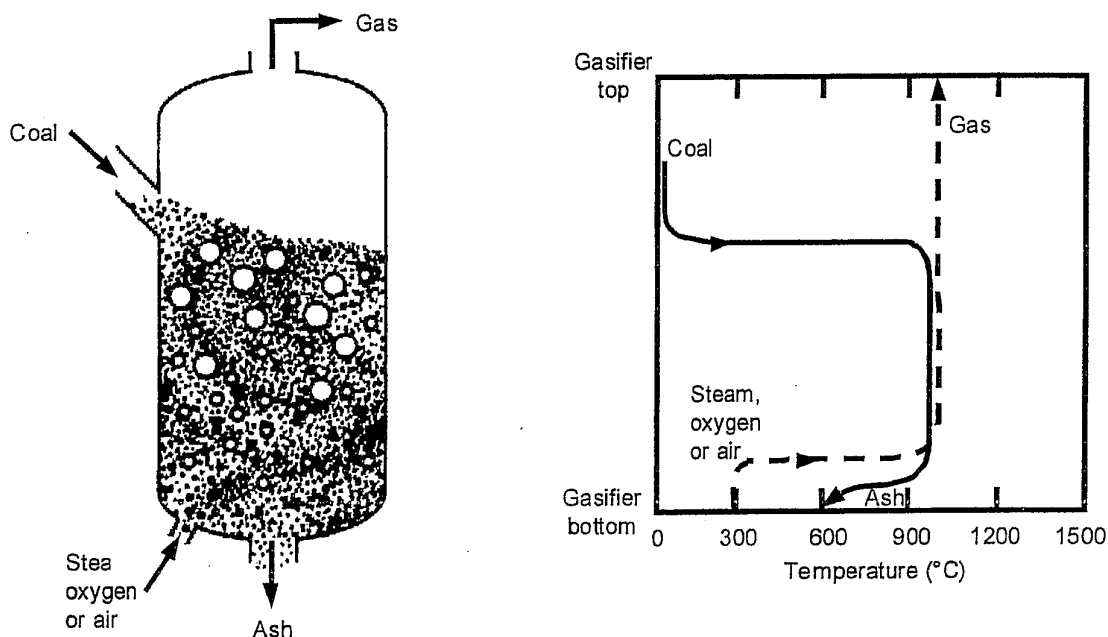
Figure 69 Fluidized bed gasifier and typical temperature profile [174].
