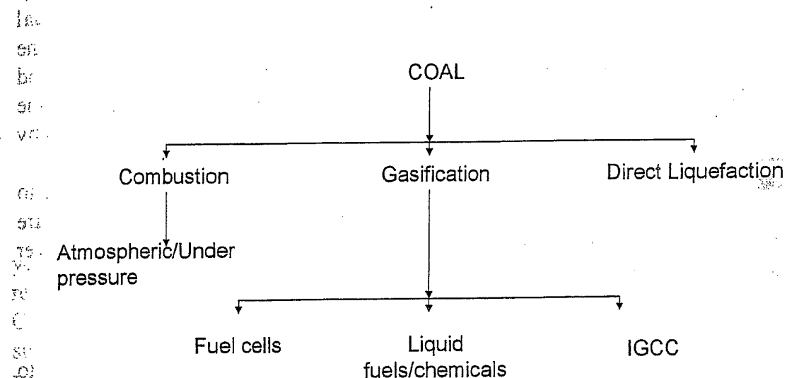
Figure 65 Different options for coal conversion and power generation. [175]
