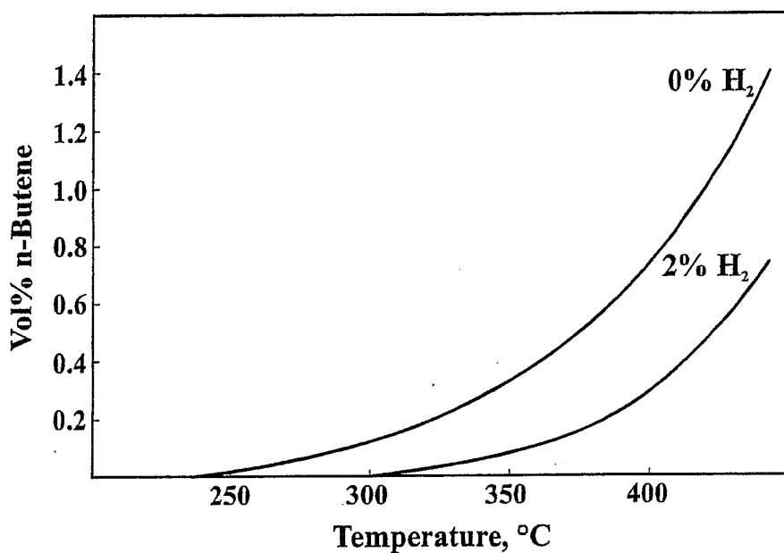
Figure 2 Equilibrium concentration of butene in n-butane at 30 bar g
