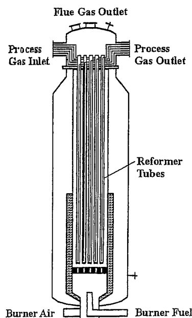
Figure 29 Topsøe Convection Reformer (HTCR) [59]
