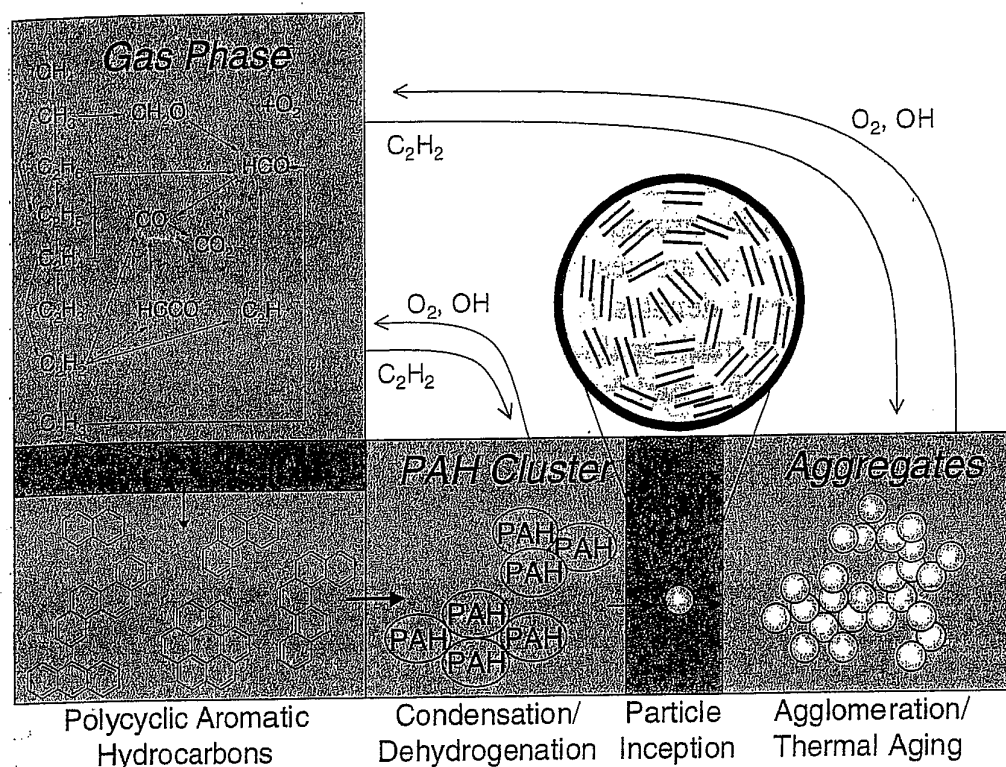
Figure 54 Schematic representation of reaction steps involved in the soot formation in methane combustion, taken from [128].
