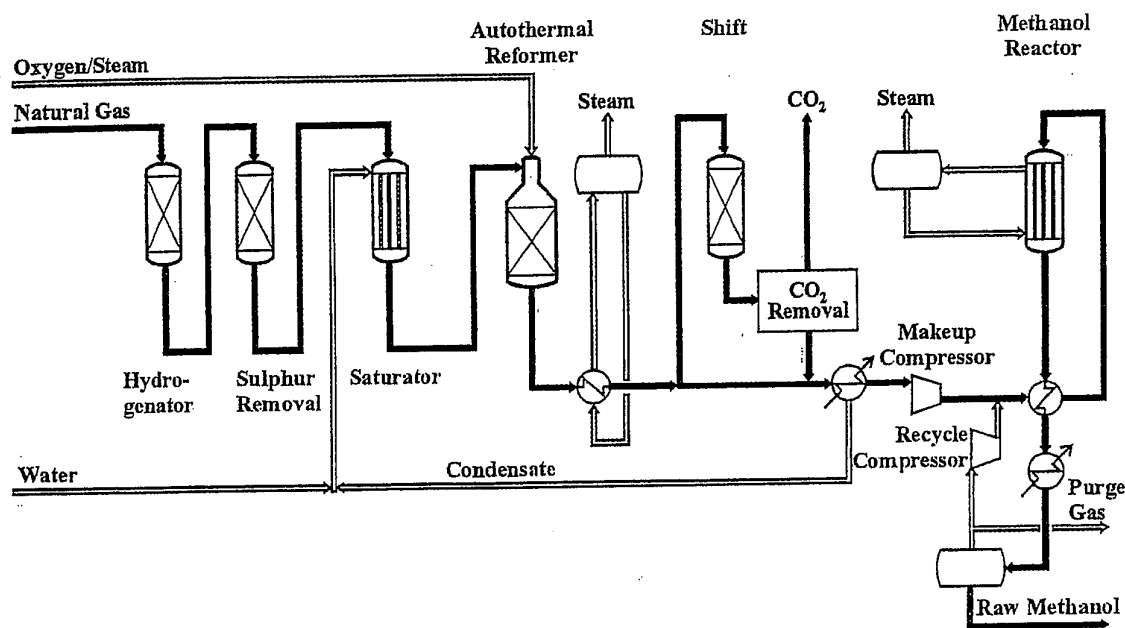
Figure 48 Methanol production by ATR and \text{CO}_2 removal [104].
