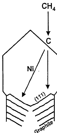
Figure 40 Schematic illustration of the process by which carbon whiskers are formed at the nickel particle during steam reforming.
