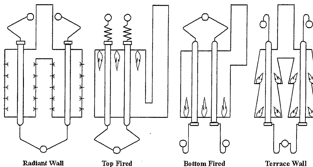
Figure 15 Tube and burner arrangements [4]
