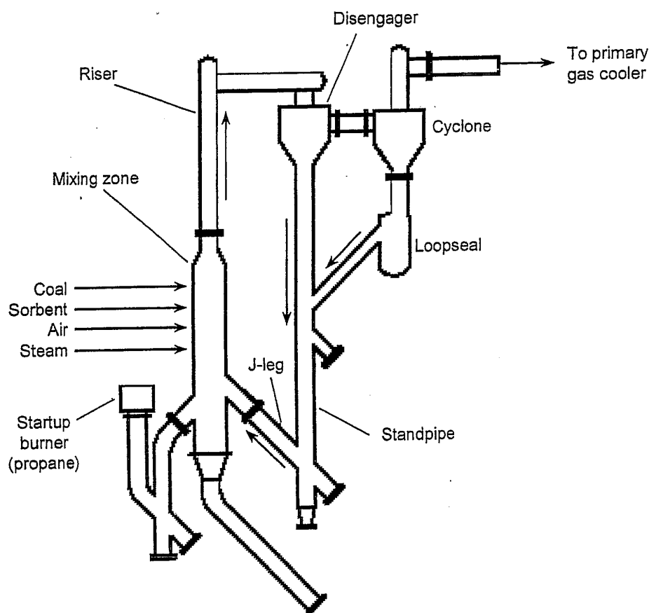
Figure 72 Transport reactor [191]
