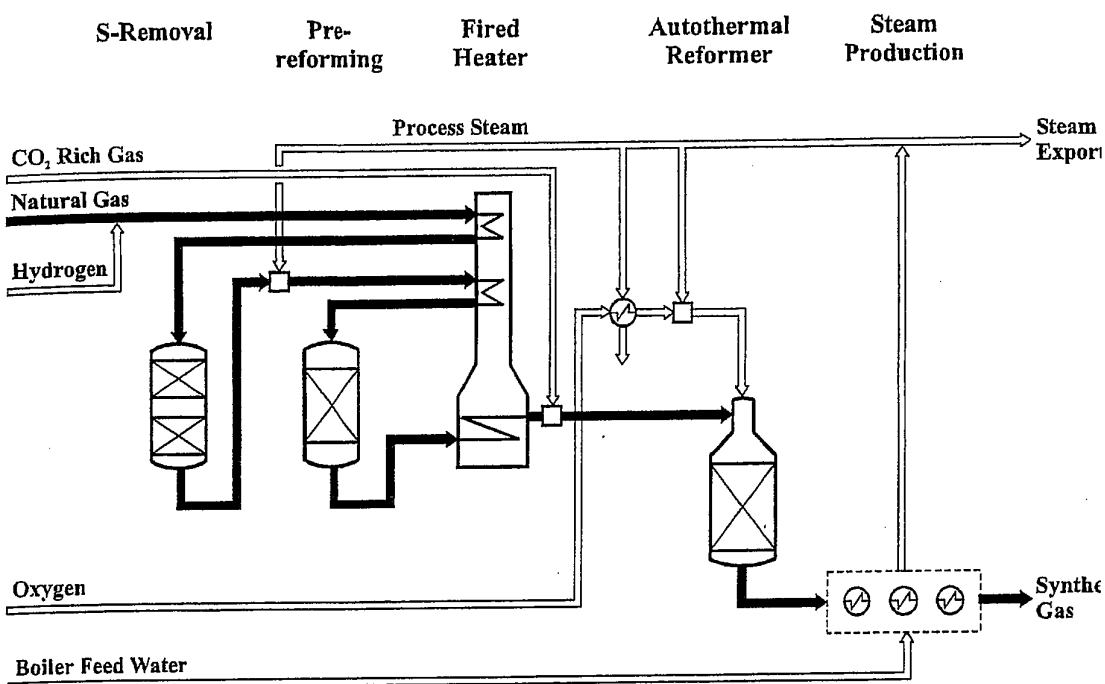
Figure 50 Typical process flow diagram for synthesis gas production for GTL
