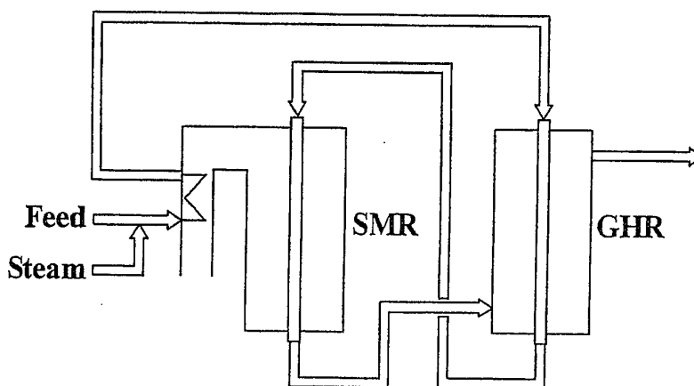
Figure 30 'Gas Heated Prereforming': Fired tubular reforming (SMR) and Gas Heated Reformer (GHR) in series arrangement
