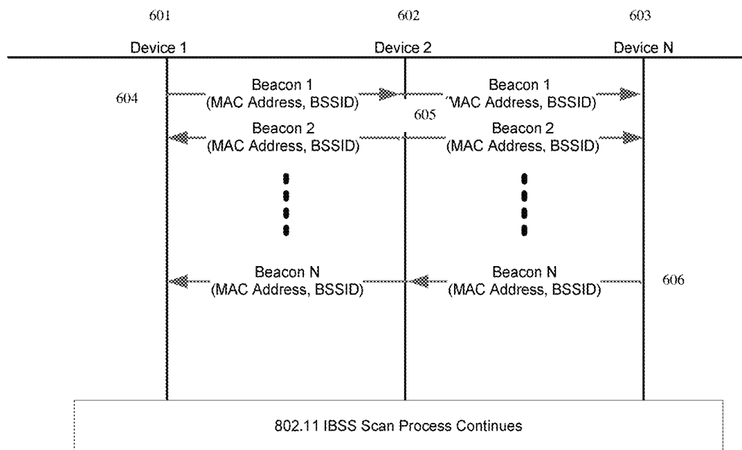
Figure 6 - 802.11 IBSS Beacon Process
