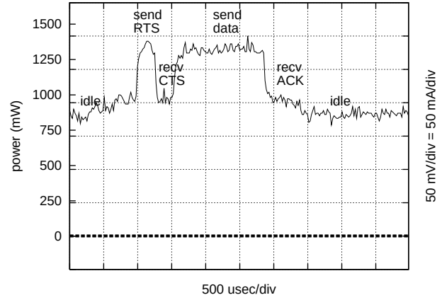
Fig. 5. Sending 2Mbps point-to-point UDP/IP traffic (256 bytes)
