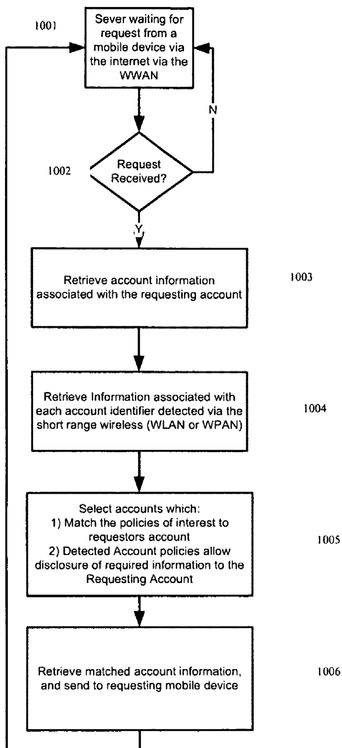
Figure 10 – Server Processing Example for Detected Device
