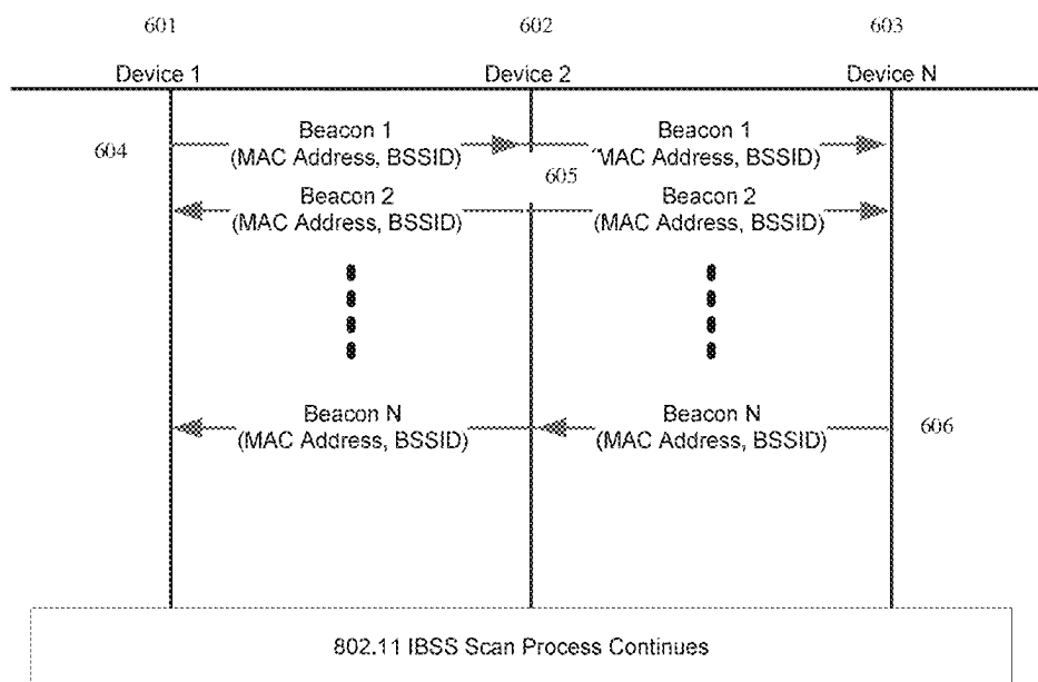
Figure 6 - 802.11 IBSS Beacon Process
