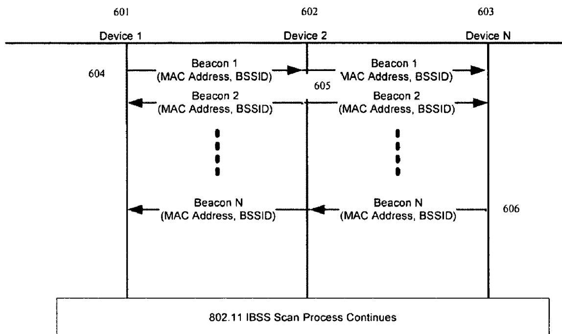
Figure 6 - 802.11 IBSS Beacon Process
